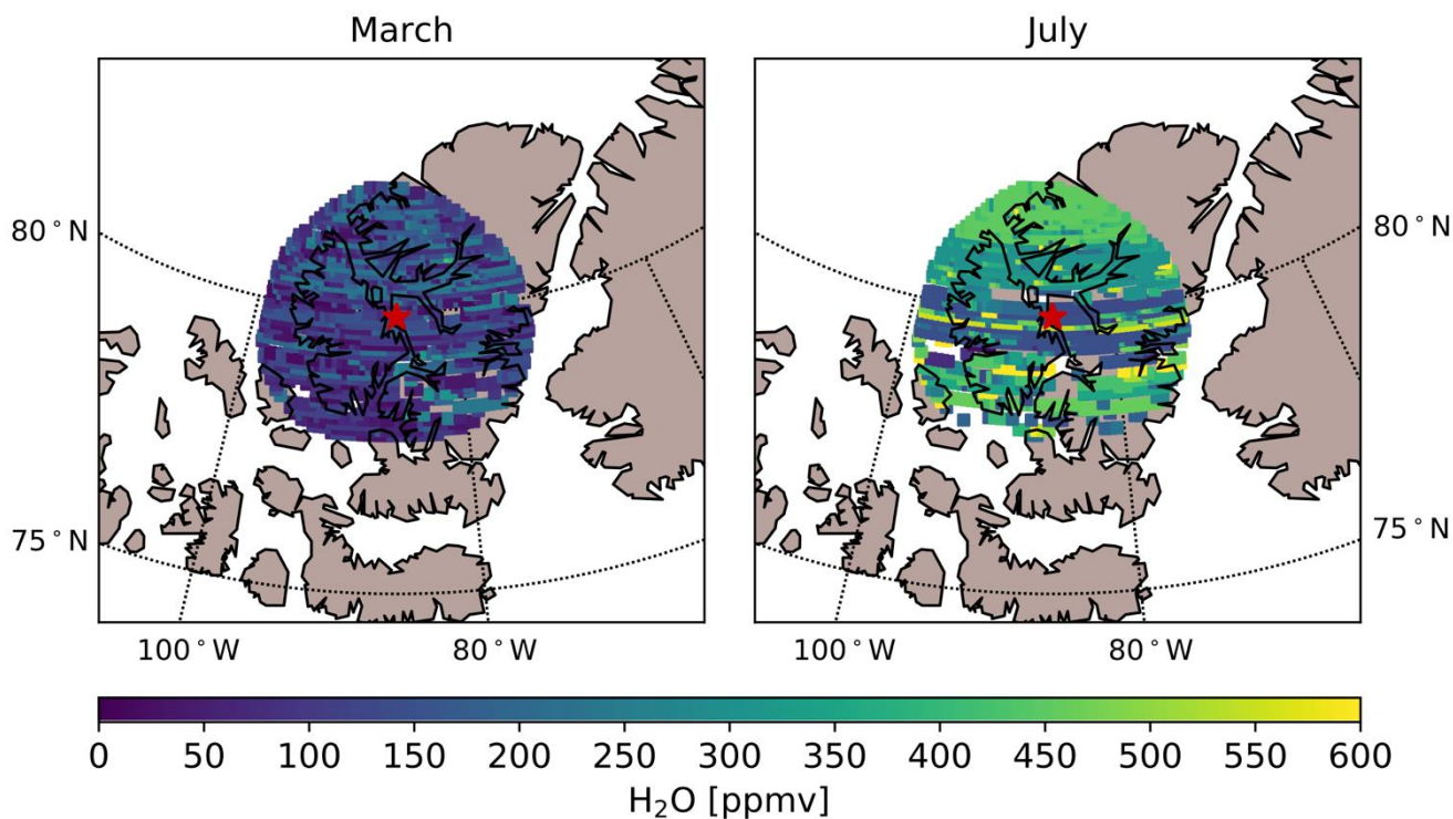
Figure 3: Average AIRS water vapour abundances at 400 hPa near Eureka (indicated by the red star), calculated by taking the mean value of all AIRS measurements between 2006 and 2016 within 50 x 50 km grid boxes.
