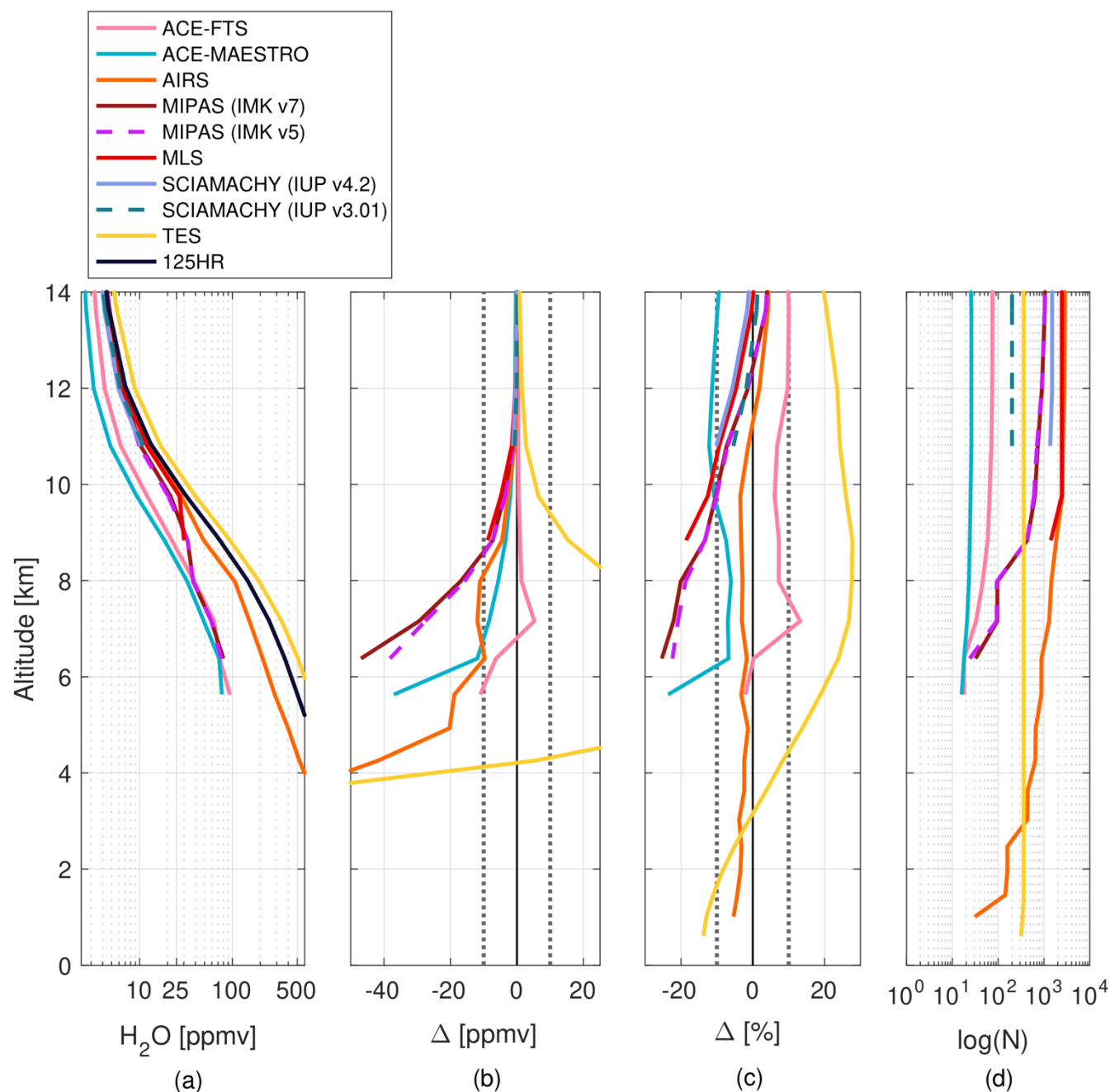
Figure 9: Same as Fig. 6, but a summary of differences between satellite measurements and Eureka radiosondes. A version of this figure with only the ACE-FTS and ACE-MAESTRO is available in the supplementary materials as Fig. S2.
