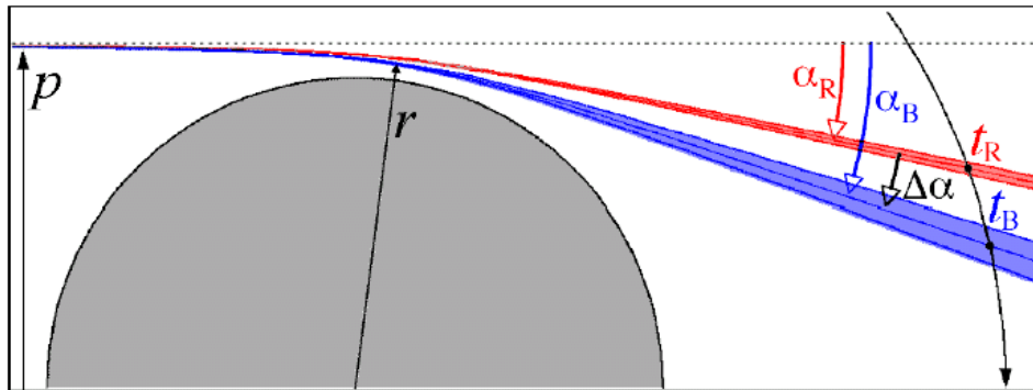
Figure 1 A scheme of chromatic refraction and the principle of refraction angle measurement by GOMOS. Both the refraction angles and the effect of dispersion are strongly exaggerated. However, the width of each beam relative to the angle difference \Delta\alpha is realistic. The impact parameter p is the geometric distance of the ray from the Earth's center. The vertical separation of blue and red rays at ray perigee 30 km is \sim 10 m (Dalaidier et al., 2001).
