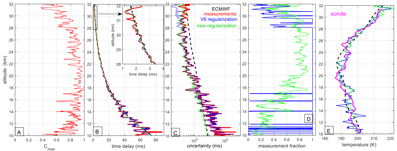
15 Figure 5. Illustration of time delay regularization and retrievals based on occultation R07673/S001; red: pure measurements, blue: V6 regularization, green: new (Bayesian) regularization, black: a priori (ECMWF). A: profile of cross-correlation coefficient C_{max} . B: profiles of time delay, C: uncertainty of time delay; D: measurement fraction, E: retrieved temperature profiles and collocated sonde measurements at Marambio (magenta line)
