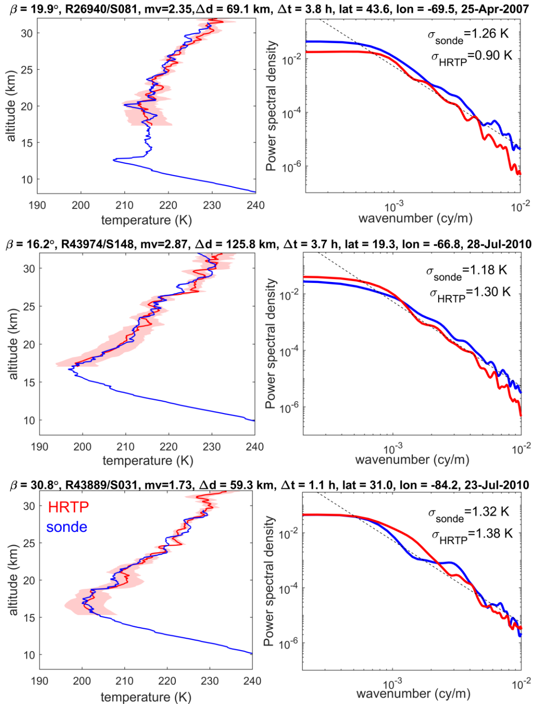
Figure 7. As Figure 6, but for oblique occultations or/and not bright stars.
