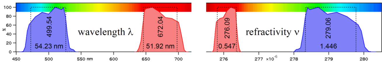
Figure 3 Left: GOMOS optical filter response as a function of wavelength. Right: refractivity bandwidth of the GOMOS optical filters.
