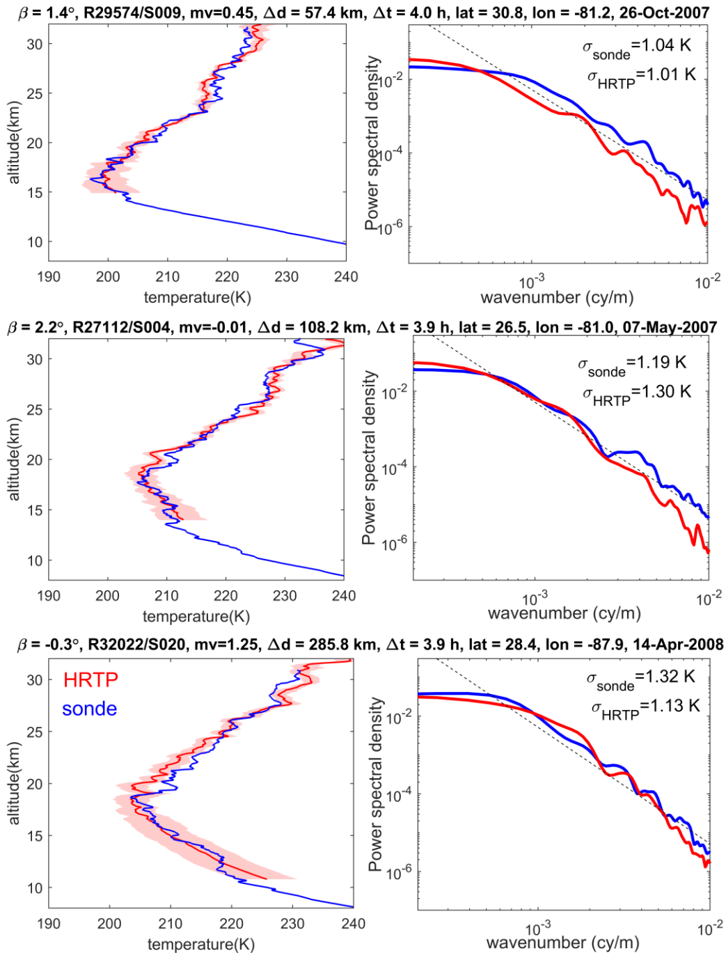
5 Figure 6. Left: examples of HRTP and collocated radiosonde profiles for some full-dark vertical occultations of very bright stars: Right: power spectral densities for these profiles, for the altitude range 18-30 km. Dashed black lines show the spectra corresponding to the saturated gravity waves model with the slope -3 (Smith et al., 1987). The information about GOMOS measurements, obliquity angles \beta , star magnitude mv , spatial \Delta d and temporal \Delta t separation, as well as the values of rms fluctuations are specified in the Figure.
