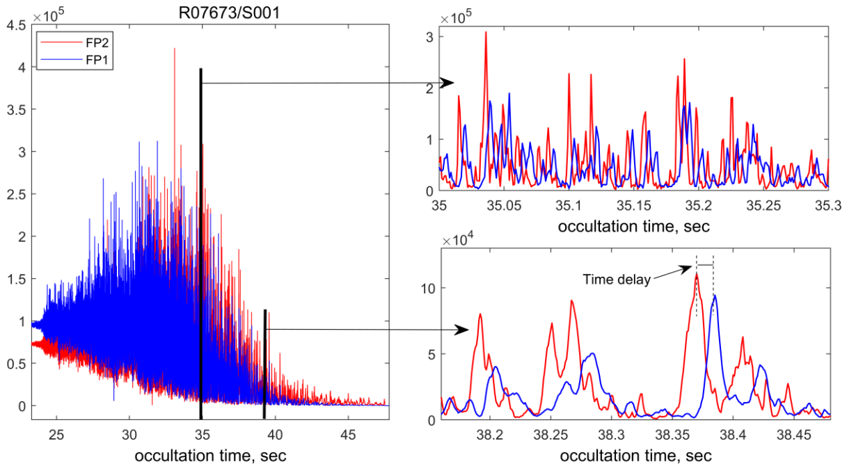
Figure 2. Signals of red (FP2) and blue (FP1) GOMOS photometers.
