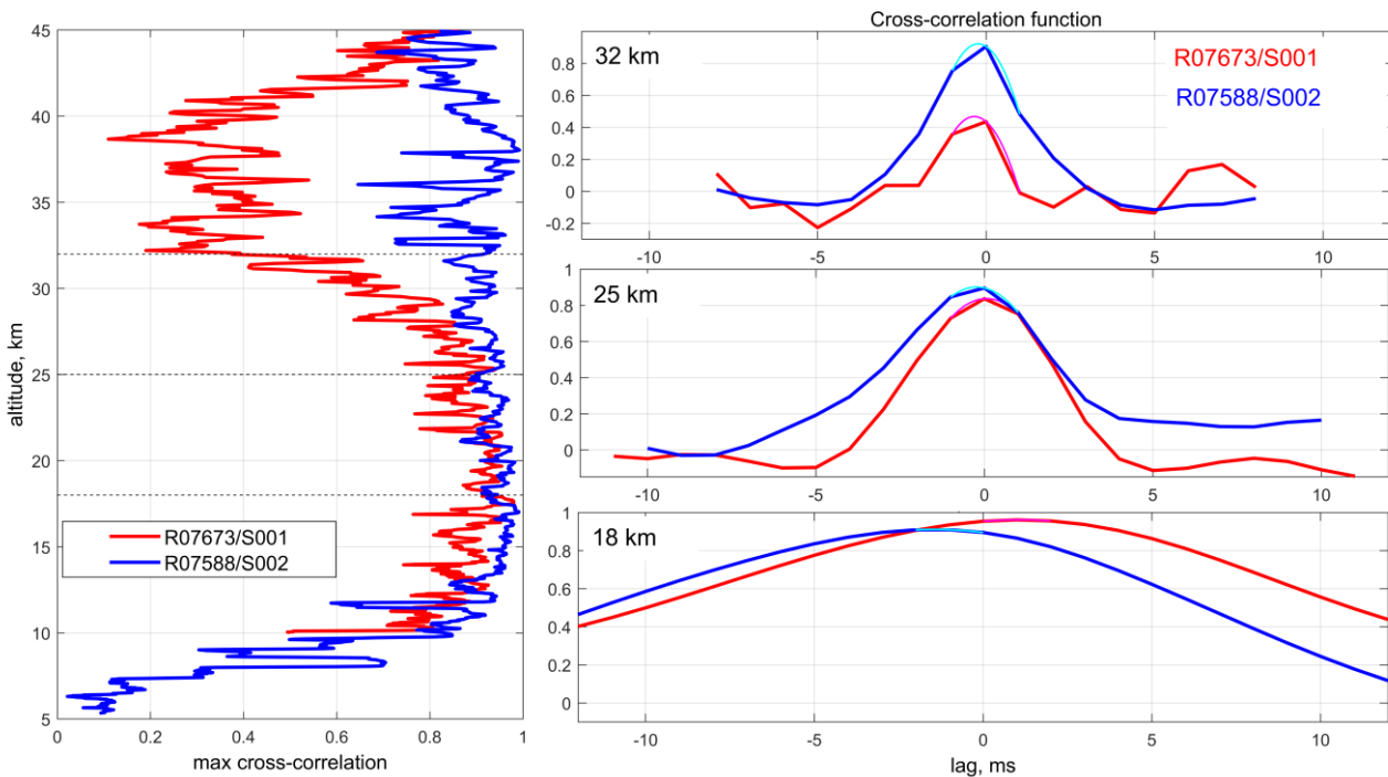
Figure 4 Left: maximum of cross-correlation function for two GOMOS occultations: R07673/S001 (64°S 68°W, \beta=23^\circ , 19-Aug-2003 04:09:23), red line, and R07588/S002 (35°S 135°W \beta=-2.6^\circ 13-Aug-2003 07:28:35), blue line. Right: examples of cross-correlation functions at selected altitudes and their fit with parabola.
