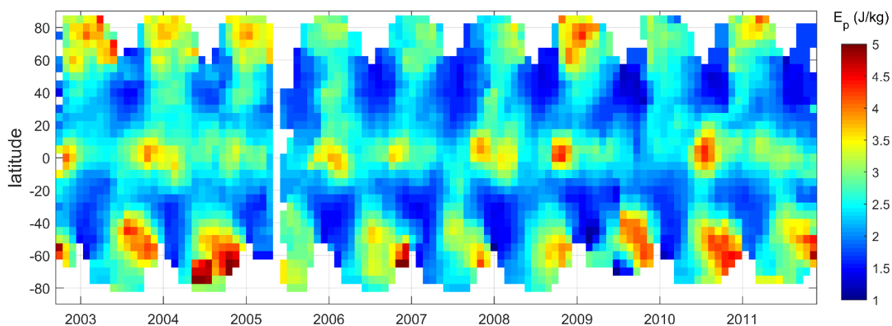
Figure 11. Time series of GW potential energy (zonal average) estimated from GOMOS HRTM in years 2002-2011.
