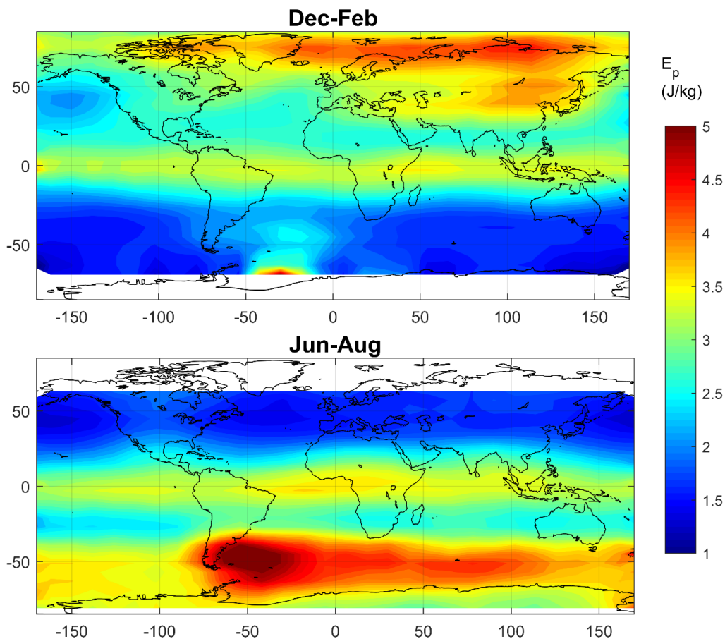
Figure 10. GW potential energy in two seasons, in years 2002-2011.
