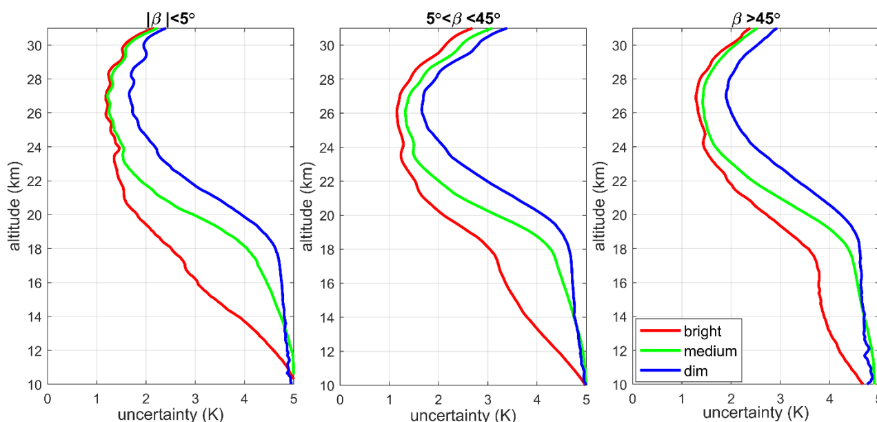
Figure 8. Mean uncertainties of HRTP in the equatorial region 20°S-20°N in 2004, for different obliquity angles \beta specified in the panels, and for different stars: bright ( m_v < 1 ), medium ( 1 < m_v < 2.5 ) and dim ( m_v > 2.5 ).
