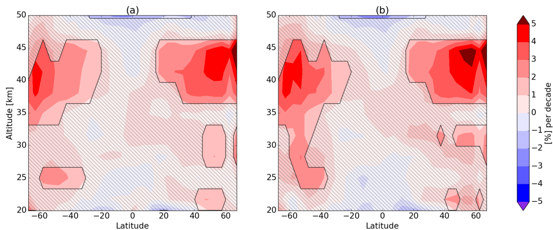
Figure 6. Zonal mean linear long-term ozone changes over the 2003–2018 period derived from the SCIAMACHY/OMPS-LP merged data sets: panel (a) shows the results using anomalies, panel (b) shows the results the 'plain-debiased' data set. Dashed areas indicate non-significant trends.
