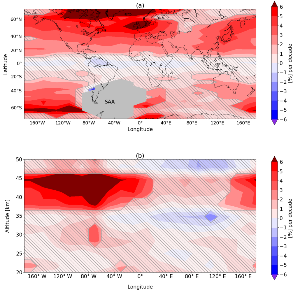
Figure 8. Panel (a) : longitudinally resolved ozone trends at 41.3 km in % per decade, computed over the 2003–2018 period from the SCIAMACHY/OMPS-LP anomalies merged data. Dashed areas indicate non-significant trends and the gray polygon labeled as SAA indicate the location of the South Atlantic Anomaly. In panel (b), cross section of the longitudinally resolved trends at 60° N.
