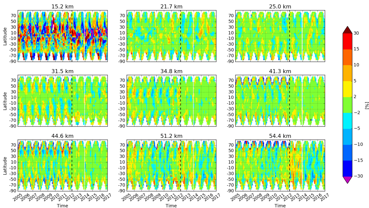
Figure 3. Relative differences of the debiased merged time series ('plain-debiasing' approach) with respect to MLS as a function of latitude for several altitudes, computed according to Eq. 3. The vertical dashed lines indicate the transition between SCIAMACHY and OMPS-LP data sets. MLS data has been offset to SCIAMACHY before the comparison.
