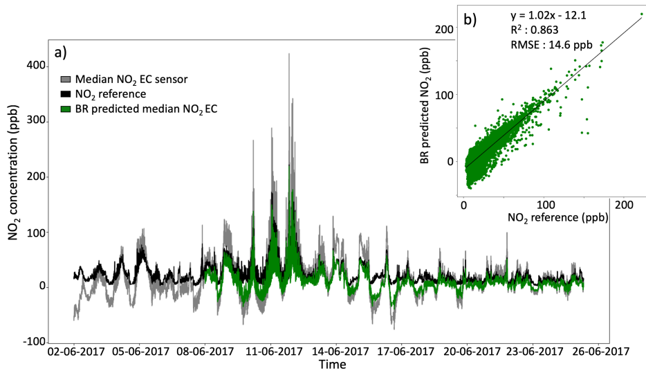
Fig. 1. Bivariate regression – Ordinary Least Squares- was performed on the median NO2 EC sensor (grey) and the NO2 CAPS measurement during the training data set. and the resulting model was applied to the me
