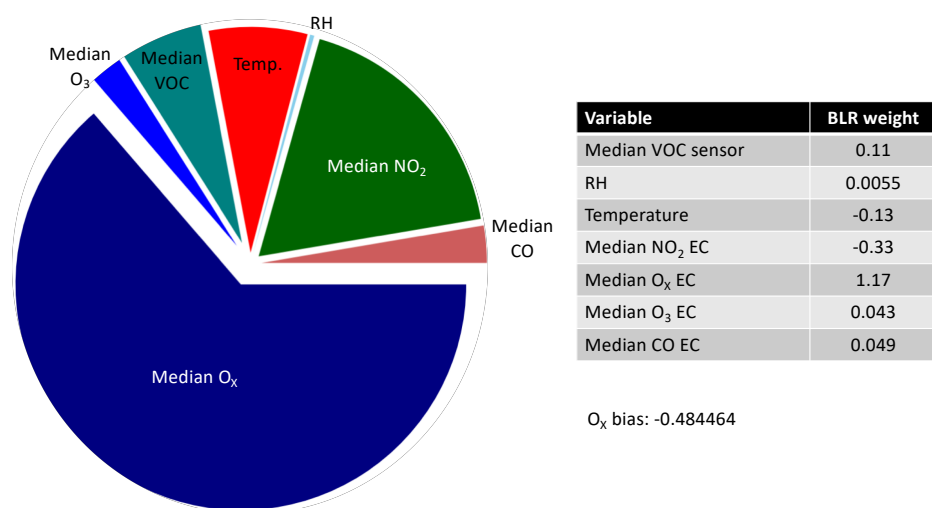
Fig. 4. Weights for the BLR-predicted OX concentration, with normalised variables prior to analysis.
