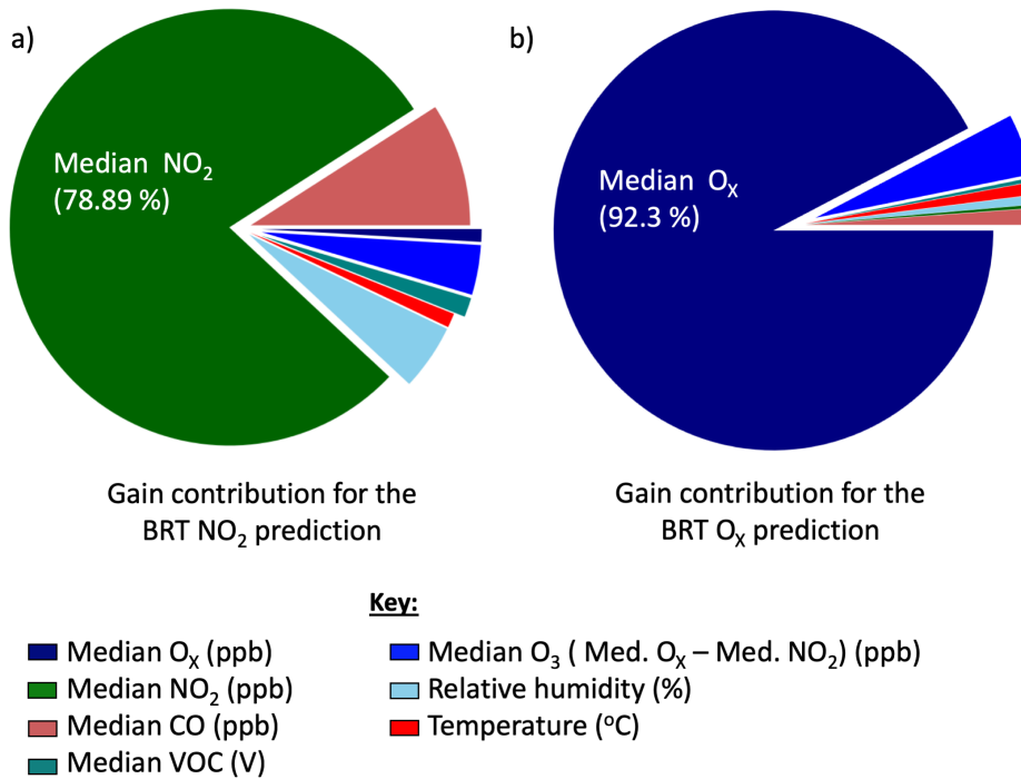
Fig. 2. (Fig. 5 in manuscript): Breakdown of contribution from each variable used by the BRT algorithm to predict the clustered a) NO2 sensor and b) OX concentrations.
