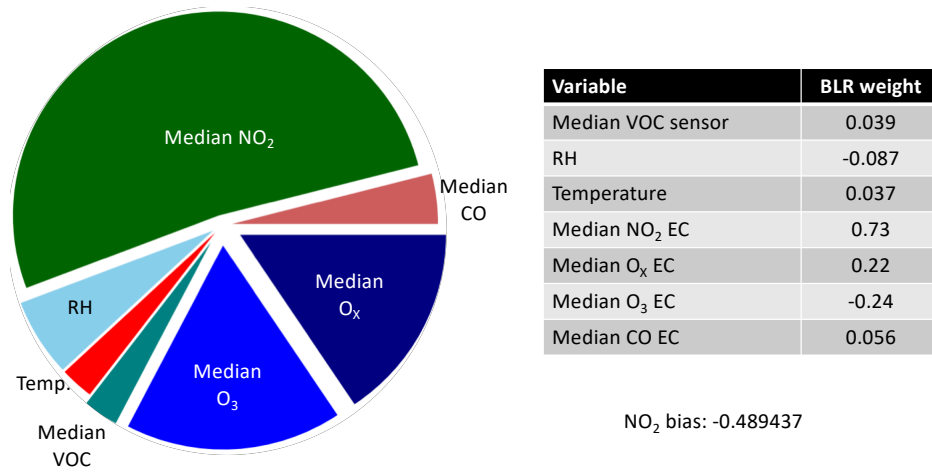
Fig. 3. Weights for the BLR-predicted NO 2 concentration, with normalised variables prior to analysis.
