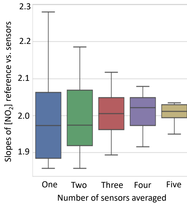
Figure 3: Comparison of slopes of concentrations derived from clusters of NO 2 EC sensors against a reference instrument for ambient Beijing air. As the number of sensors used increases, the spread in data, as seen through the difference in slope, narrows. If data from 3 out of 6 sensors is used there are 20 possible permutations of sensors. The average signal of each was calculated, then plotted against the reference NO 2 CAPS measurements and the gradient extracted. The 20 gradients of these correlation plots (sensitivities) are then plotted in the boxplots above, with the median, 25 th percentile, 75 th percentile in the box and the 5 th and 95 th percentile on the whiskers.
