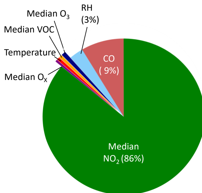
Figure 5: Breakdown of contribution from each variable used by the BRT algorithm to predict the clustered NO 2 sensor concentration.
