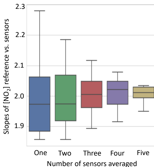
Figure 3: Comparison of slopes of concentrations derived from clusters of \text{NO}_2 EC sensors against a reference instrument for ambient Beijing air. As the number of sensors used increases, the spread in data, as seen through the difference in slope, narrows. If data from 3 out of 6 sensors is used there are 20 possible permutations of sensors. The average signal of each was calculated, then plotted against the reference \text{NO}_2 CAPS measurements and the gradient extracted. The 20 gradients of these correlation plots (sensitivities) are then plotted in the boxplots above, with the median, 25 th percentile, 75 th percentile in the box and the 5 th and 95 th percentile on the whiskers.
