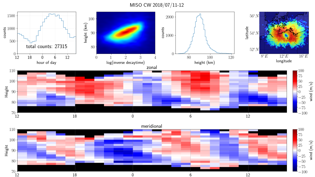
Figure 4. Similar to Figure 2 but for the MISO-CW system, i.e., the signals of 5 synthetic receivers have been incoherently integrated. The transmitter and receiver sites are indicated with green crosses. Note that the region of less counts is over the mid-point of the receiver and transmitter sites.
