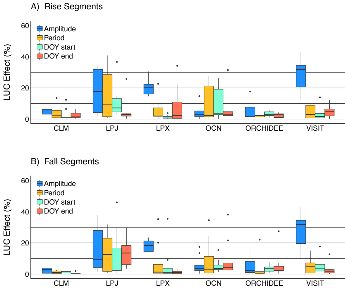
Figure 8. Land Use Change effect on amplitude, period, and day of year (DOY). The percentages were calculated from the difference in the metrics between simulations (S3-S2), scaled relative to amplitude and period of Rise and Fall segments for each region and model; DOY was scaled against the period.
