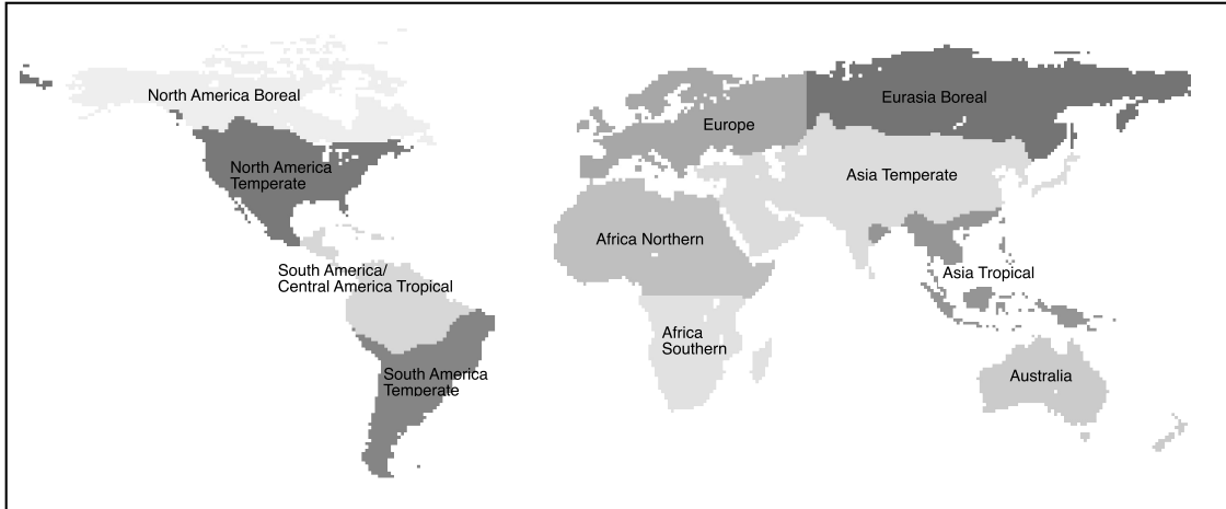
Figure 2. TransCom region map.
