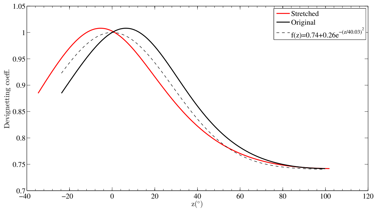
Figure 9. Devignetting coefficient: black line: original data, red line: stretched mirrored curve, dashed line: fit.
