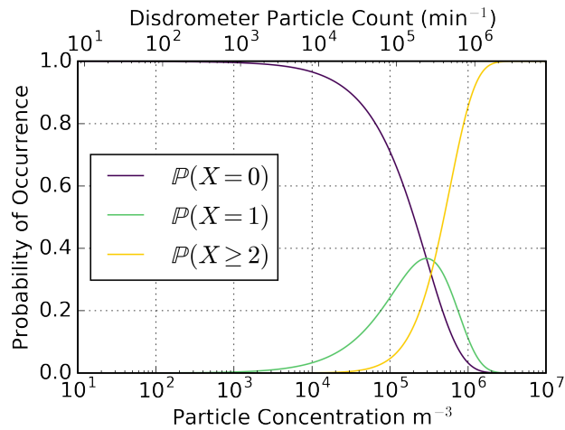
Figure 2. Probability of X number of drops residing in within the disdrometer beam for a given drop concentration. If two or more drops are within the beam simultaneously, data quality can be reduced. More than 12,000 \text{ drops m}^{-3} (equivalent to 10,000 \text{ drops min}^{-1} recorded by the disdrometer*) are required before the probability of 2 or more drops occurring in the beam simultaneously becomes non-negligible. As such, any events with more than 10,000 drops observed per minute should be treated as less reliable. *Drops falling through the disdrometer beam assumes a 3 \text{ m s}^{-1} fall velocity, which from Gunn and Kinzer (1949) is a particle of approximately 0.8 mm diameter, typically the average size observed for a moderate rainfall event. Droplet breakup on the housing of the Thies LPM is not factored into this test.
