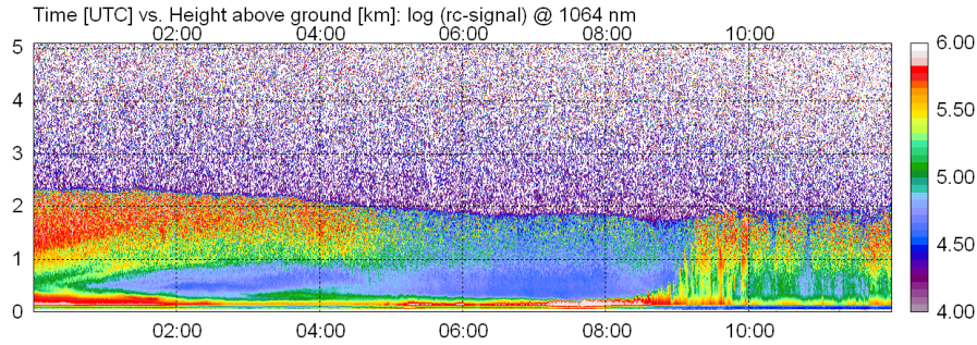
Figure 13. Time-height cross section of the range corrected signal (in arbitrary units, logarithmic scale) of the CHX-2-CHX-1 from 20 August 2015 from midnight until noon (including Case B). Time is given in UTC, and the height above ground in km; note, that the maximum height shown is not the full measurement range of the ceilometer.
