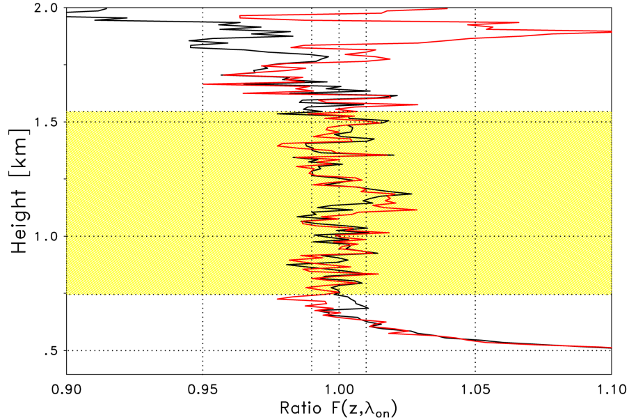
Figure 1: An example of F for CL51-1 (black line) and CL51-2 (red line), \kappa = \text{const.} (Case B). Compare to Fig. 16 of the manuscript and see detailed explanations above.
