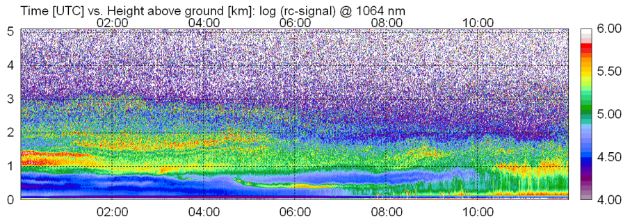
Figure 17. Same as Time-height cross section of the range corrected signal (in arbitrary units, logarithmic scale) of the CHX-1: similar to Fig. 9 but for 14 August 2015 (Case C).
