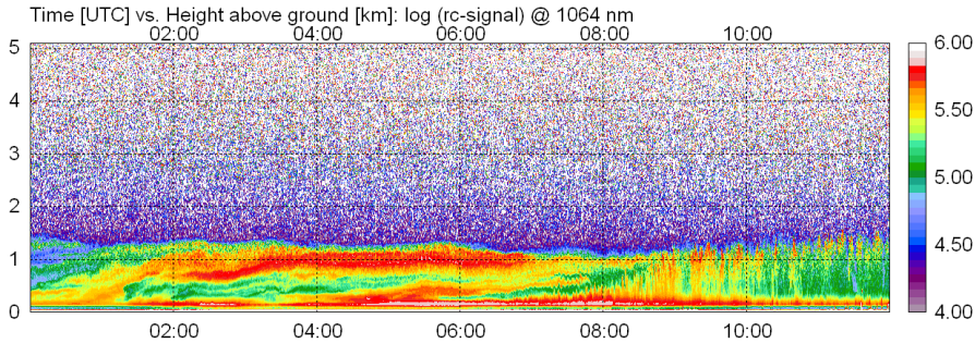
Figure 9. Time-height cross section of the range corrected signal (in arbitrary units, logarithmic scale) of CHX-2-CHX-1 from 2 July 2015 (including Case A) until noon. Time is given in UTC, and the height above ground in km; note, that the maximum height vertical range shown here is not the full measurement range of the ceilometer.
