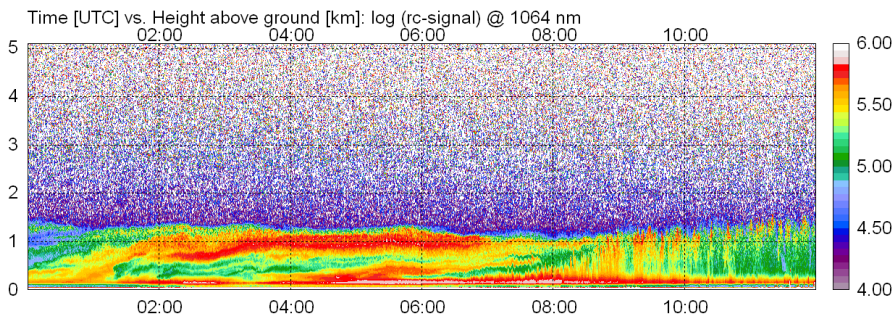
Figure 9. Time-height cross section of the range corrected signal (in arbitrary units, logarithmic scale) of CHX-1 from 2 July 2015 (including Case A) until noon. Time is given in UTC, and the height above ground in km; note, that the vertical range shown here is not the full measurement range of the ceilometer.
