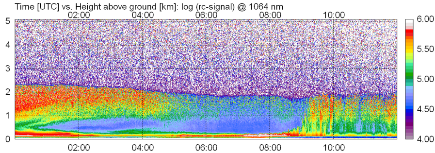
Figure 13. Time-height cross section of the range corrected signal (in arbitrary units, logarithmic scale) of the CHX-1 from 20 August 2015 from midnight until noon (including Case B). Time is given in UTC, and the height above ground in km; note, that the maximum height shown is not the full measurement range of the ceilometer.
