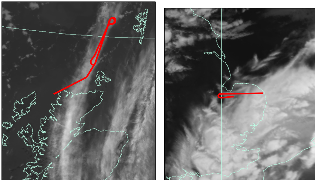
Figure 1. 10.8 \mu m infra-red satellite image from 10:02UTC MetOp-B overpass on March 13th 2015 (left) and 11:01UTC MetOp-A overpass on February 9th 2016 (right). The aircraft track during the remote sensing runs is overlaid in red.
