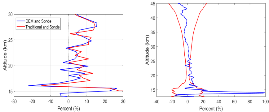
Figure 9. For the night of 26 July 2017. Left panel: The percentage difference between the OEM retrieval and the ozonesonde measurements in the form of: (\frac{\text{sonde}-OEM}{OEM} * 100) (blue curve); the percentage difference between the traditional retrieval and the ozonesonde measurements in the form of (\frac{\text{sonde}-\text{traditional}}{\text{traditional}} * 100) (red curve). The difference between the traditional method as the sonde profile below 14 km is greater than 100%, thus is not shown in the figure. Right panel: The percentage difference between the OEM retrieval and the traditional retrieval (blue curve); the summation of the statistical uncertainty of the traditional and OEM retrievals (red curve).
