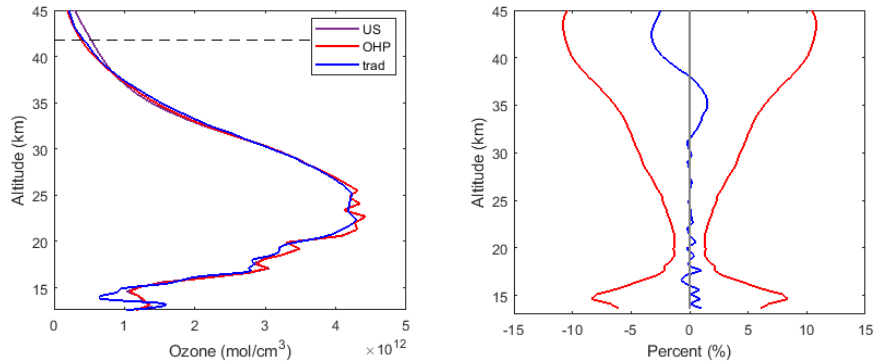
Figure 10. For the night of 26 July 2017. The left panel: the OEM retrieval using the US standard model as a a priori profile (purple curve) and the OEM retrieval using the OHP climatology as a a priori profile (red curve) are plotted. Furthermore, the traditional method retrieval (blue curve) is plotted, thus the OEM retrievals can be compared with each other and with the traditional retrieval. The right panel: Percentage difference between the OEM retrievals using the two different a priori profiles (blue curve) is plotted. This difference is within the retrieval uncertainty. At higher altitudes (above 35 km), when the SNR drops, the difference between the two methods is less than 5%, which is smaller than the retrieval uncertainty at that height.
