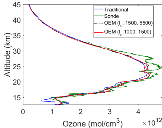
Figure 8. OEM ozone retrieval (red curve) from 20:07 UT to 00:15 UT on 26 July 2017 as well as the ozonesonde profile (green curve) and the traditional ozone retrieval (blue curve) are plotted. The dashed black line shows the OEM retrieval when the correlation length ( l_s ) became larger. The horizontal dashed line shows the cut-off below which the effect of the a priori ozone profile is small less than 10%.
