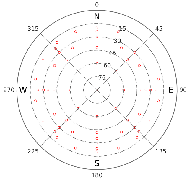
Figure 5. A measurement cycle of the WVR begins begun with two azimuth scans. In order to avoid emission from the ground the lowest elevation angle observed is was 20^\circ . Starting in the north, first turning at an elevation angle of 20^\circ clockwise to the north (excluding the azimuth angles of 40^\circ and 60^\circ due to a nearby radio telescope), and then turning counterclockwise at an elevation angle of 35^\circ . Thereafter four tip curves are were made over the zenith direction (implying four observations in the zenith direction during each cycle): from the north to the south, from the southwest to the northeast, from the east to the west, and from the northwest to the southeast. The cycle is was about 8 min long and is was repeated continuously, implying that almost two complete cycles with a total of \approx 100 \approx 100 observations are were used when estimating gradients every 15 min.
