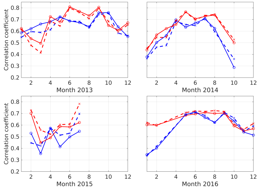
Figure 13. Correlations between estimated wet gradients from the WVR data and the GPS data from ONSA (solid lines) and ONS1 (dotted lines) averaged over 15 min when the hydrostatic gradients have been are removed from the total GPS gradients for each month of the four years. The east gradients are presented with red lines and the north gradients with blue lines.
