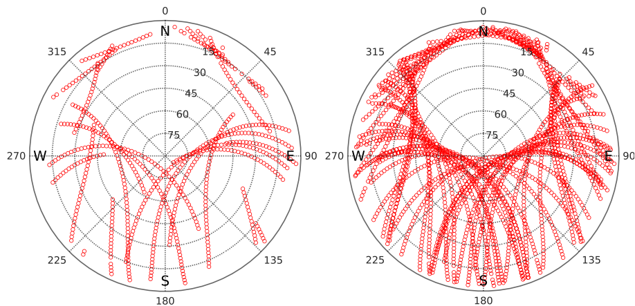
Figure 3. Sky plots of GPS observations at Onsala from 6 to 12 UT (left) and from 0 to 24 UT (right) on May 12, 2014. This particular day was chosen because results from this day are discussed it is included in the CONT14 campaign presented in Section 5.3. The sky distribution of observations is very similar, although not identical, for all days.
