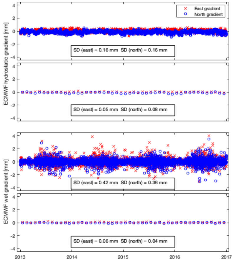
Figure 8. The ECMWF gradients for the ONSA (ONSA) site during the 4-year time period studied in Section ??5. From the top: hydrostatic gradients every 6 h, their monthly averages, wet gradients every 6 h, and their monthly averages.
