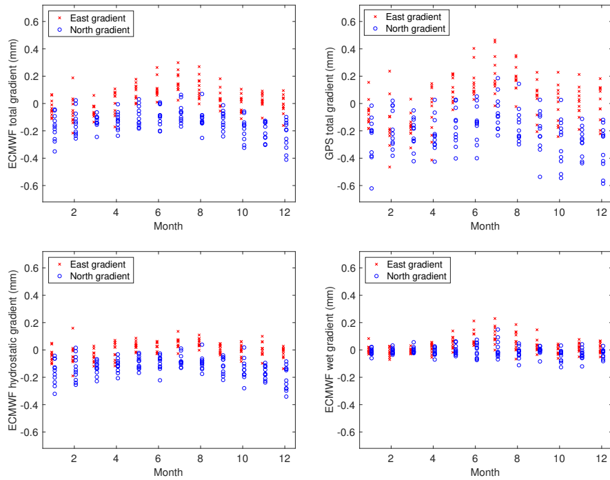
Figure 9. Monthly means of estimated gradients at the Onsala-ONSA station for the period 2006–2016. The top graphs show the total gradients from ECMWF (left) and GPS (right). The graphs at the bottom show the ECMWF gradients when separated into the hydrostatic (left) and the wet gradient (right).
