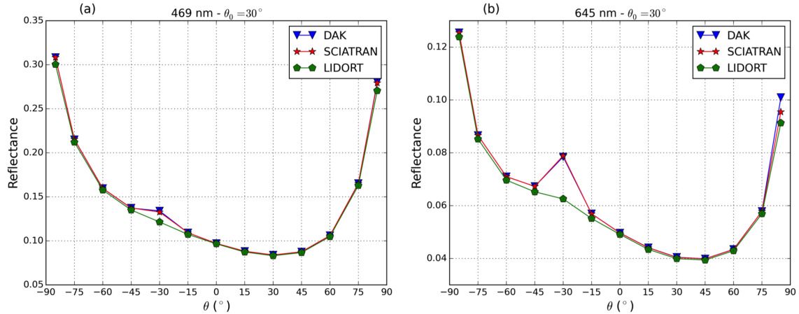
Figure 5. TOA reflectance at (a) 469 nm and (b) 645 nm simulated by DAK (blue), SCIATRAN (red) and LIDORT (green) with the Ross-Li surface BRDF model with parameters representing a vegetated surface over Amazonia as in Fig.4 as a function of the viewing zenith angle in the principal plane ( \varphi - \varphi_0 = 180^\circ for negative \theta and \varphi - \varphi_0 = 0^\circ for positive \theta ), for \theta_0 = 30^\circ .
