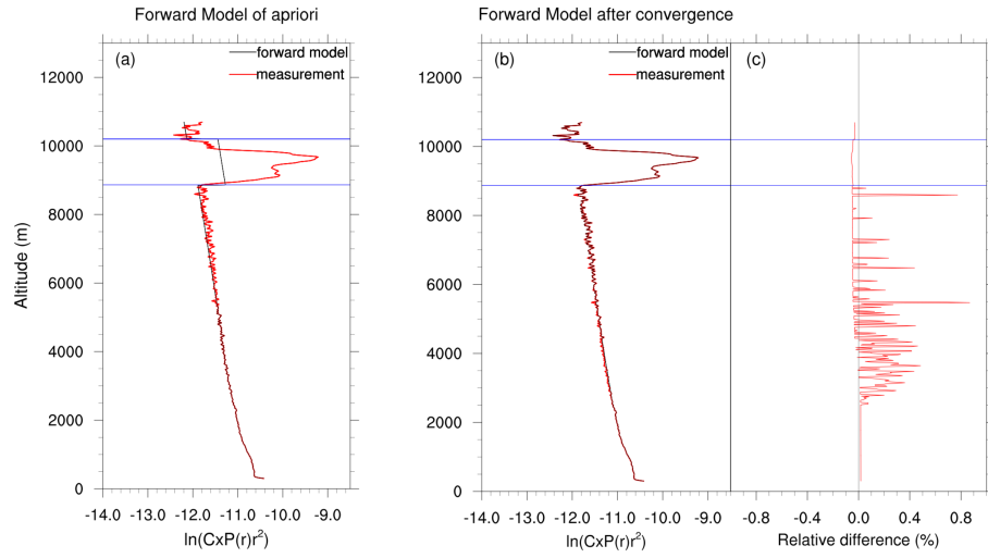
Figure 2. Forward model of the (a) a priori, and (b) after the last iteration step (represented by the black lines) for the lidar profile measured on November 30, 2016 at 18.18 UTC. The red lines represent the measurement, the horizontal blue lines indicate the defined cloud base and top altitudes. (c) Relative difference between the forward model and the measurement after convergence.
