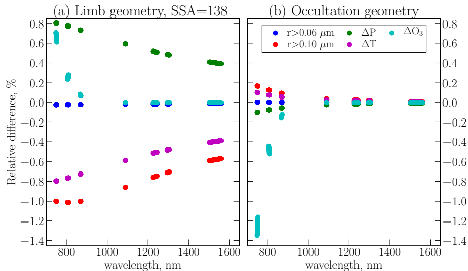
Figure 2. Relative changes in the radiance at 21.7 km for limb (panel (a)) and occultation (panel (b)) geometry. The responses in radiance due to 10% changes in temperature, atmospheric pressure and ozone concentration are presented by magenta, green and cyan dots, respectively. The cut off in PSD at 0.06 \mu\text{m} is depicted with blue dots, and the cut off at 0.10 \mu\text{m} is presented with red dots.
