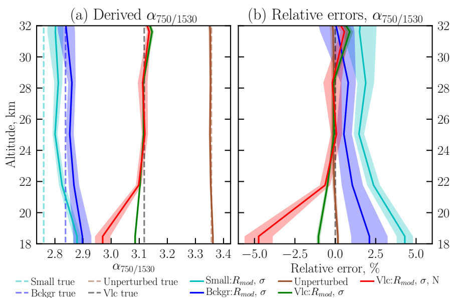
Figure 4. Ångström exponent profiles ( \alpha_{750/1530} ) (a) and their relative errors (b) for a typical tropical observation geometry. The solid lines show the derived from PSD product profiles, while the dashed lines represent the true values. The shaded areas stand for \pm 1 standard deviation. The scenarios used for the simulations are listed in Table 2.
