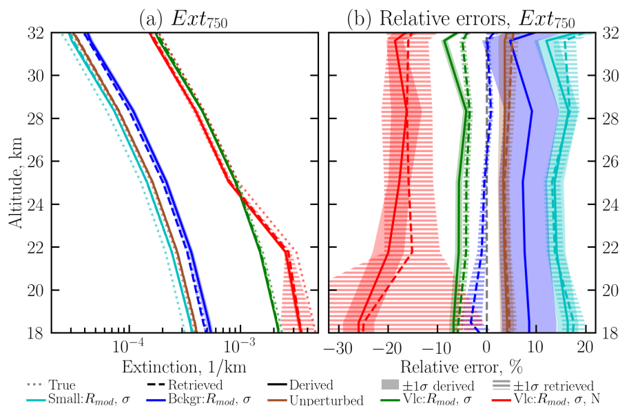
Figure 3. Profiles of Ext_{750} (a) and their relative errors (b) for a typical tropical observation geometry. The solid lines show the calculated from PSD product profiles, dashed lines depict the directly retrieved profiles, while the dotted lines represent the true values. The shaded areas stand for \pm 1 standard deviation. The scenarios used for the simulations are listed in Table 1.
