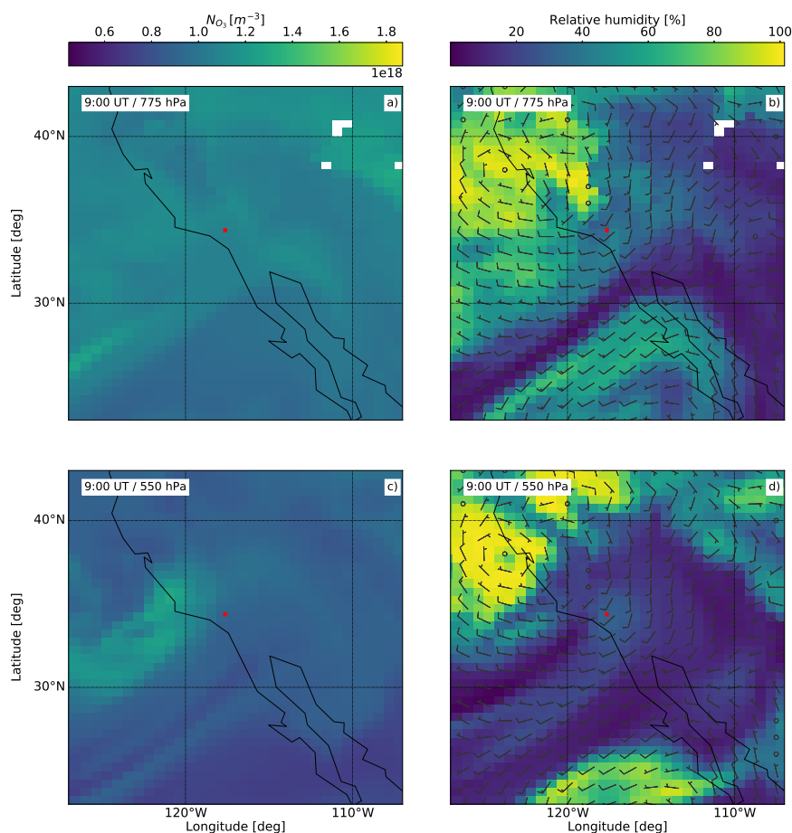
Figure 9. MERRA-2 reanalysis at 9:00 UT on 25 May 2018 for two different pressure levels (775 hPa and 550 hPa). a,c) Ozone number concentration. b,d) Relative humidity and wind speed/direction. TMF site location is indicated with a red dot.
