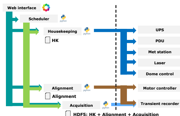
Figure 2. Block diagram of the new acquisition and lidar control software.
