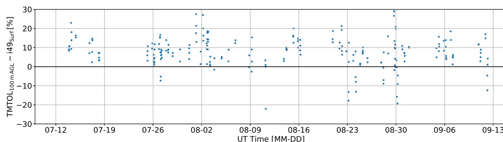
Figure 12. Relative difference between the first valid lidar data point (100 m AGL) and the collocated i49 surface ozone meter for the period comprehended between 13 July and 12 September 2018. Each point corresponds to a 30 minute average.
