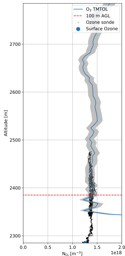
Figure 8. Comparison between the TMTOL very-near-range receiver retrieval (solid, blue), an ozonesonde tethered system (dots, black) and a surface ozone monitor (dot, blue). Lidar retrieval 1 - \sigma uncertainty is shown (gray, shaded).
