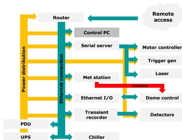
Figure 1. Block diagram describing the the power distribution (orange) and data transfer (green) between different subsystems of the lidar. Hatch hardware interlock based on rain sensing is shown in red.
