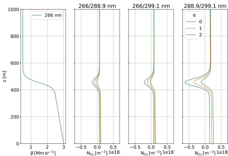
Figure 4. Aerosol error contribution (differential backscatter and extinction contributions) based for the different available DIAL wavelength pairs and three different Ångström exponents ( \alpha ).
