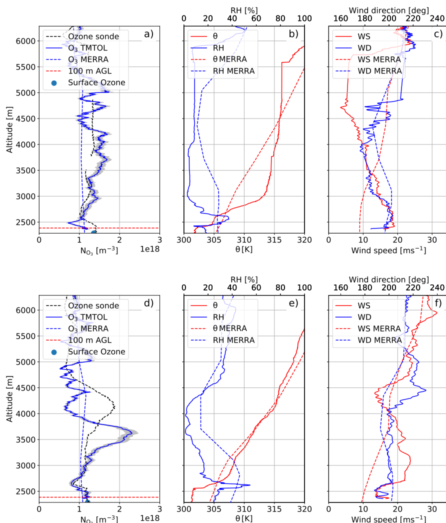
Figure 11. Comparison between the retrieved lidar ozone profile (together with 1 - \sigma uncertainty), collocated radiosondes, surface ozone meter and MERRA-2 reanalysis at the time of the first (upper row, 4:40 UT) and second launch (lower row, 9:10 UT). a,d) Lidar ozone profile (solid, blue), ozone sonde profile (dashed, black), MERRA-2 ozone concentration and surface ozone measurements (light blue). b,e) Radiosonde potential temperature (solid, red), MERRA-2 potential temperature (dashed, red), radiosonde relative humidity (solid, blue) and MERRA-2 relative humidity (dashed, blue). c,f) Radiosonde wind speed (solid, red), MERRA-2 wind speed (dashed, red), radiosonde wind direction (solid, blue) and MERRA-2 wind direction (dashed, blue).
