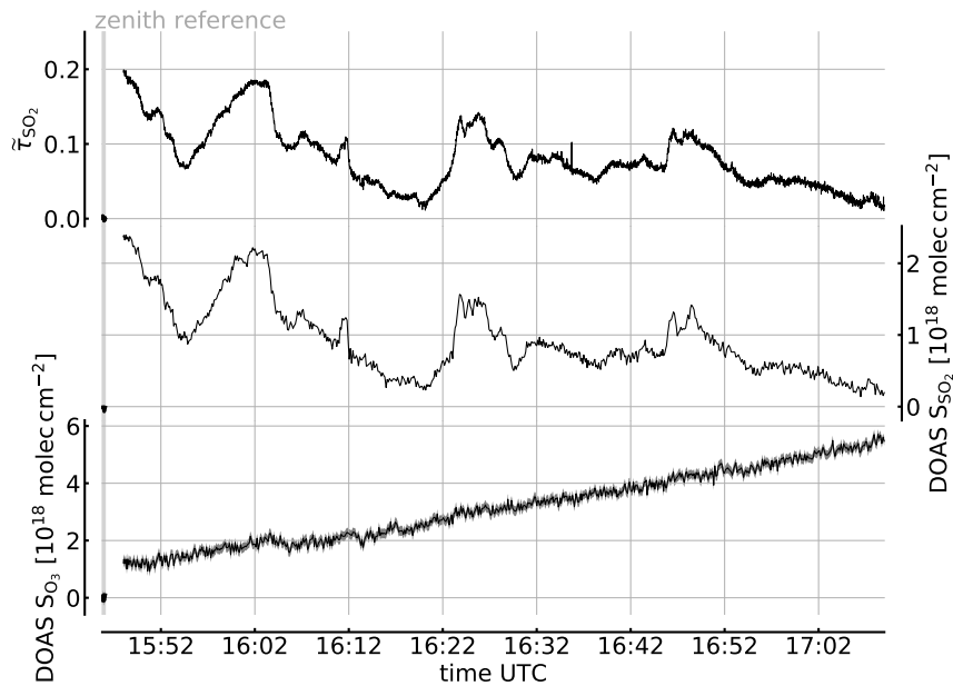
Figure 6. Time series of the apparent absorbance of the one pixel FPI Correlation Spectroscopy prototype for \text{SO}_2 detection (top trace, left scale) recorded at Etna, Sicily on 30 July 2017. A co-aligned telescope was used to simultaneously record spectra for DOAS evaluation of \text{SO}_2 and \text{O}_3 (center and bottom traces and right and bottom left scales, respectively). The apparent absorbance nicely correlates with the \text{SO}_2 CD (see Fig. 7), while no \text{O}_3 impact is observable. The growth of the retrieved \text{O}_3 differential CD is expected due to the increasing stratospheric \text{O}_3 column for increasing solar zenith angle (see text).
