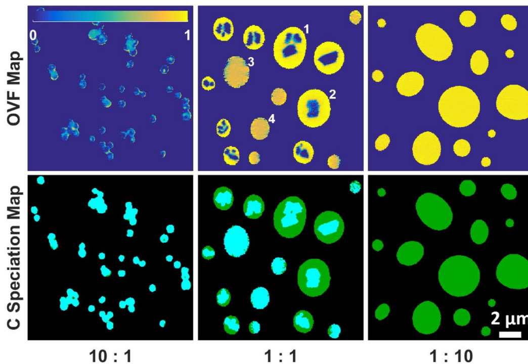
Figure 4: Representative Organic Volume Fraction (OVF) maps and C speciation maps for the ammonium sulfate/sucrose systems. Samples shown were collected from impactor stage C (0.5–0.25 μm nominal size range). For the C speciation maps, green represents inorganic dominant and blue represents inorganic dominant regions. The 4 particles are labeled in the top middle image, have OVFs of: 0.56, 0.41, 0.77, and 0.79 for particles labeled #1, 2, 3, and 4, respectively.
