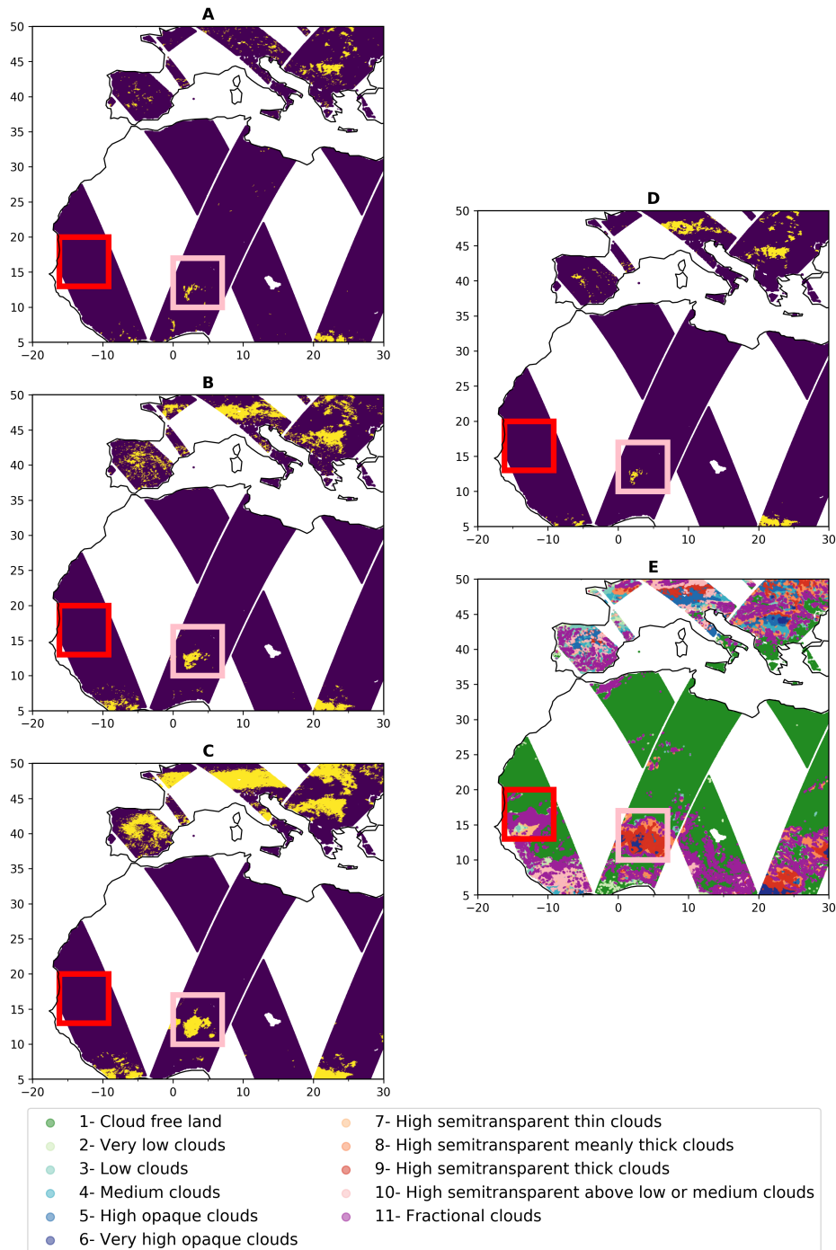
Figure 6. Maps showing for the 15th of June 2015: (A) the predicted grid cells flagged given by 3 models and thresholds the model using channels below 40GHz with different a 0.1 threshold; (B) by the model using channels available on June 15, 2015, compared to below 100GHz with a 0.05 threshold; (C) by the detecting model using channels below 190GHz with a 0.01 threshold; (D) the detected precipitating cells according according to Ferraro (1997); and (E) the cloudy classes from SEVIRI. The red and the pink squared boxes highlight two smaller regions further discussed in Section 4.3.
