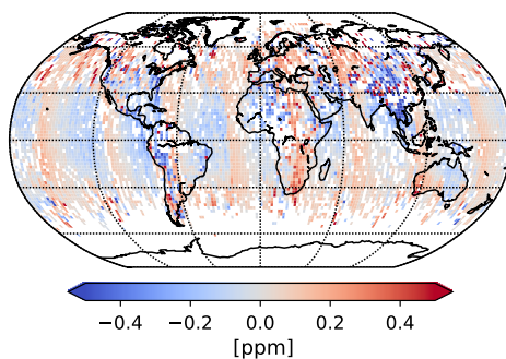
Figure 13. Global difference between v8 and v9 ( v9 - v8 ) bias corrected X_{CO_2} for April 2016. Only soundings that passed the v8 and v9 filtration are taken into account. A mean bias of 0.15 ppm (mainly introduced by the different global scaling factors for v8 and v9) is subtracted. Data is aggregated into 2^\circ \times 2^\circ latitude-longitude square grids.
