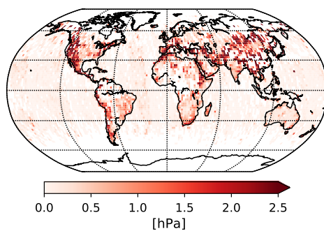
Figure 8. Difference between v9 and v8 ( v_9 - v_8 ) of the surface pressure prior standard deviation in each grid cell for April 2016. Data is aggregated into 2^\circ \times 2^\circ latitude-longitude square grids.
