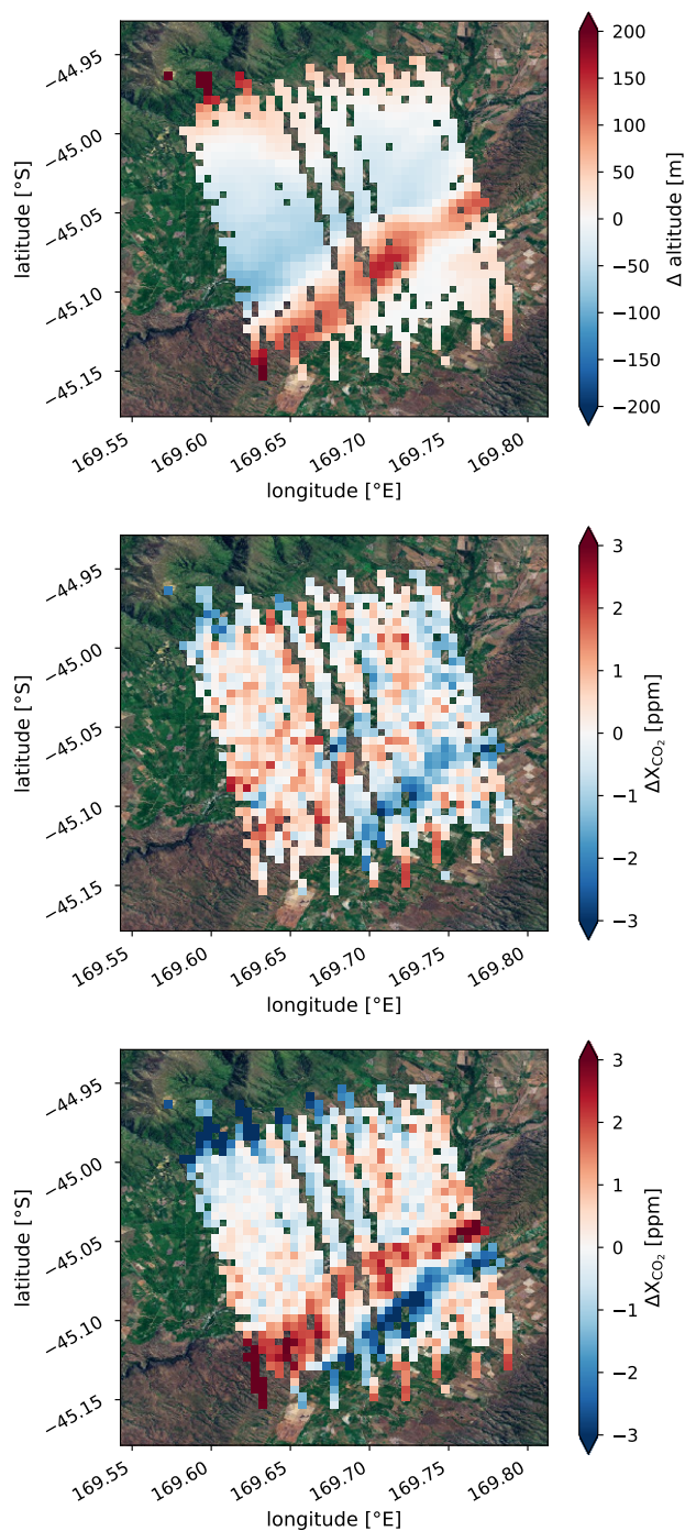
Figure 1. OCO-2 target mode observation over Lauder, New Zealand on February 17, 2015. The upper panel shows \Delta altitude (defined as the sounding altitude minus the median altitude of all soundings in the given latitude and longitude limits). The middle and lower panel show the variation of raw and bias-corrected OCO-2 v8 \Delta X_{CO_2} (defined in the same way as \Delta altitude) after applying the v8 filters. Individual soundings are aggregated into 0.005^\circ \times 0.005^\circ latitude-longitude square grids.
