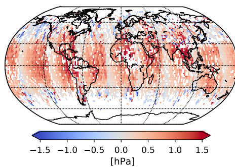
Figure 7. Mean difference between v9 and v8 ( v_9 - v_8 ) surface pressure prior for April 2016. Data is aggregated into 2^\circ \times 2^\circ latitude-longitude square grids.
