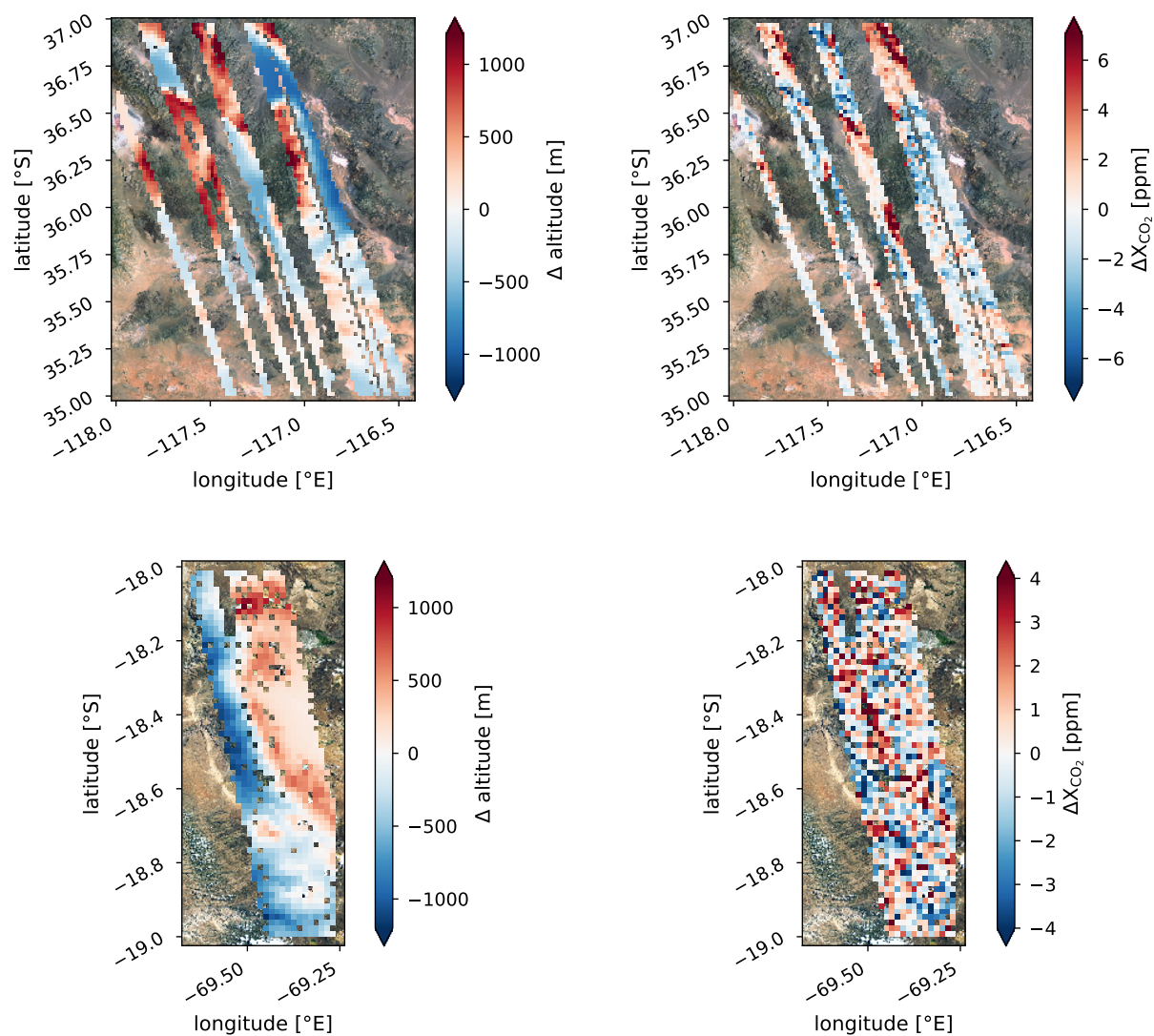
Figure 3. Variation of altitude over the two selected areas in the Death Valley National Park (upper row) and Atacama Desert (lower row). Steep topography with altitude changes of up to \pm 1000 m are observed in both areas. A topography related bias in \Delta X_{CO_2} derived from the ACOS L2FP retrieval is apparent in both regions. Individual observations are aggregated into 0.02^\circ \times 0.02^\circ latitude-longitude square grids.
