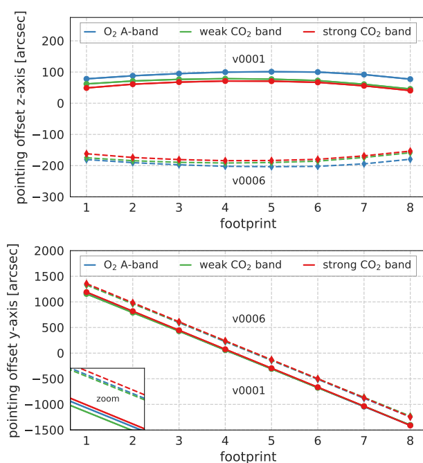
Figure 2. OCO-2 pointing offsets for each footprint and spectral band for the z-axis (upper panel) and y-axis (lower panel) derived from the pre-launch (v0001) and on-orbit (v0006) analyses.
