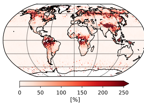
Figure 11. Relative increase of soundings that pass the v9 filtration scheme compared to v8 for the entire year 2016. Data is aggregated into 2^\circ \times 2^\circ latitude-longitude square grids.
