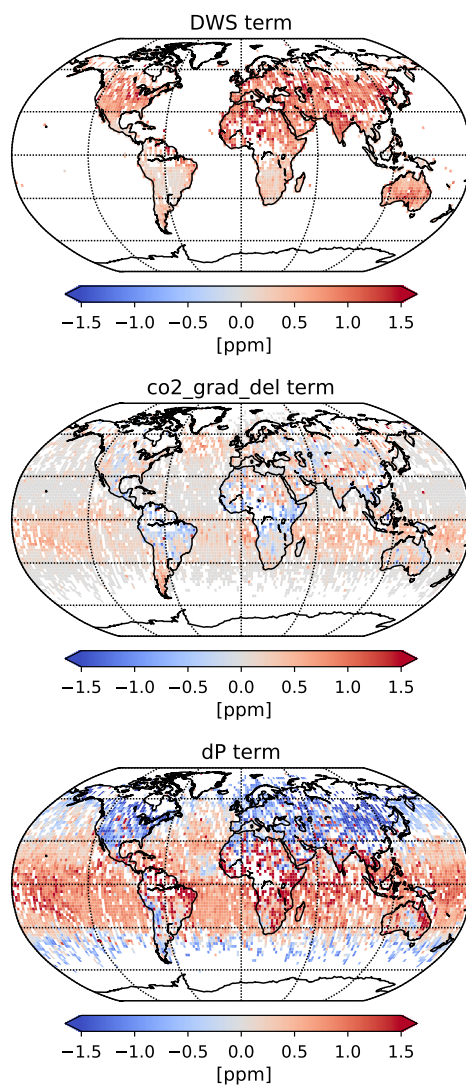
Figure 9. Contributions of the parametric bias correction terms to raw X_{CO_2} from DWS (upper panel, only over land), co2\_grad\_del (middle panel), and the two dP terms over land and ocean (lower panel) for April 2016. Data is aggregated into 2^\circ \times 2^\circ latitude-longitude square grids.
