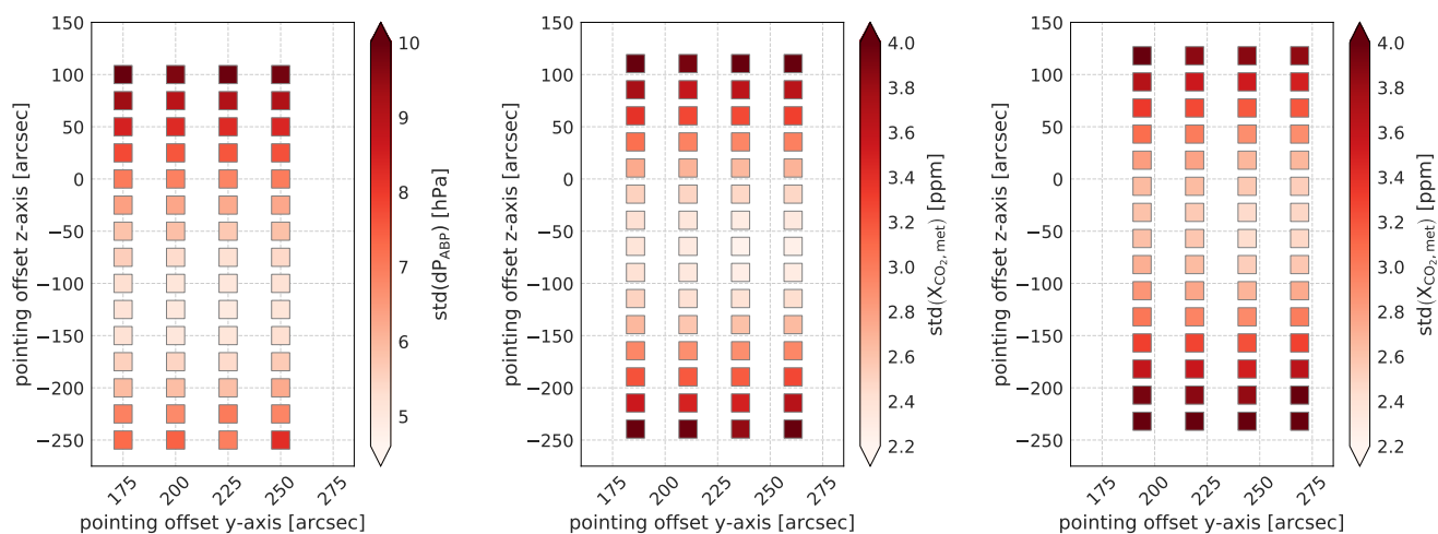
Figure 4. Standard deviation of dP_{ABP} (left panel) and X_{CO_2,met} for the weak (middle panel) and strong (right panel) CO_2 band for FP4 for all 60 geolocation configurations for the Death Valley National Park.
