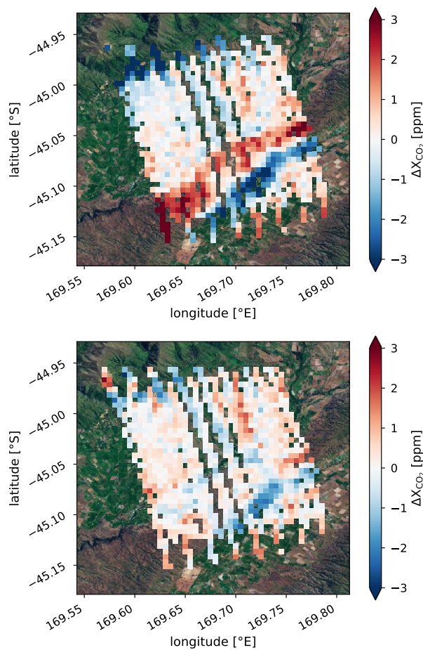
Figure 12. v8 (upper panel) and v9 (lower panel) bias corrected X_{CO_2} over Lauder, New Zealand on February 17, 2015. \Delta X_{CO_2} is defined in the same way as in Fig. 1. Data is aggregated into 0.005^\circ \times 0.005^\circ latitude-longitude square grids.
