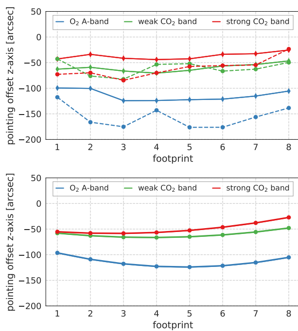
Figure 6. Upper panel: z-axis footprint pointing offsets for the three spectral bands for the Death Valley National Park (solid) and Atacama Desert (dashed); lower panel: z-axis footprint pointing offsets used in the OCO-2 v9 geometric calibration algorithm.
