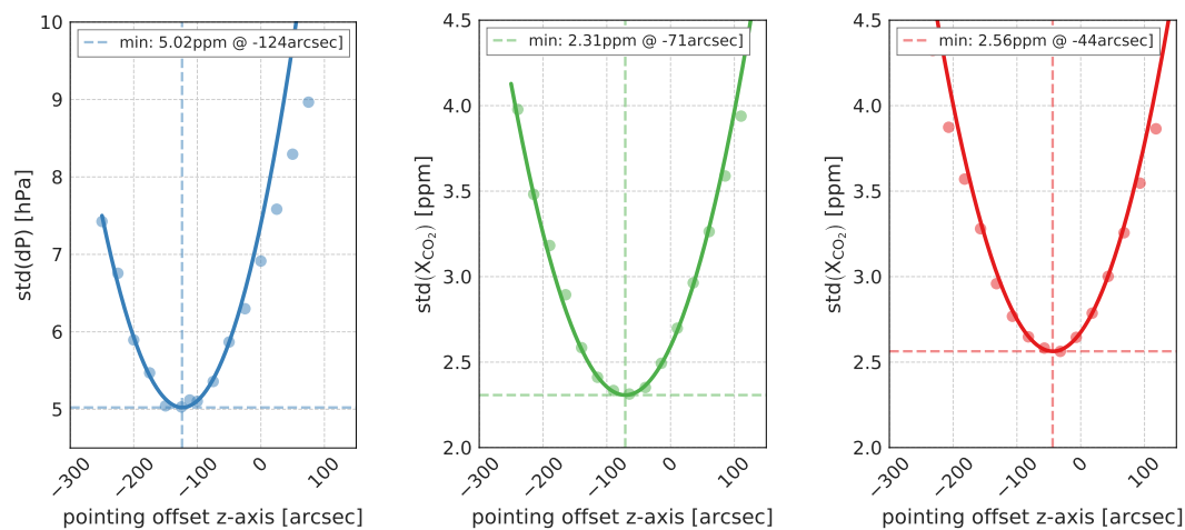
Figure 5. Standard deviation of dP_{ABP} (left panel) and X_{CO_2,met} of the weak (middle panel) and strong (right panel) CO_2 bands as a function of z-axis pointing offsets for FP4 for the Death Valley National Park. To determine the minimum, only values that are distributed symmetrically around the minimum are taken into account for the quadratic regression.
