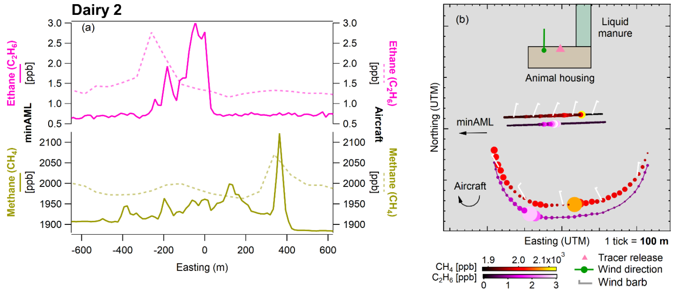
Figure 3. Plumes observed by the miniature Aerodyne Mobile Laboratory (minAML) and aircraft. Plots of methane ( CH_4 ) and ethane ( C_2H_6 ) are overlaid for each platform (panel a). Observations occurred during transects by each vehicle to the south of Dairy 2, during a release of C_2H_6 into a southerly wind (panel b). Potential emission sources on the farm have been identified as colored sections, though not as an exact scaled representation.
