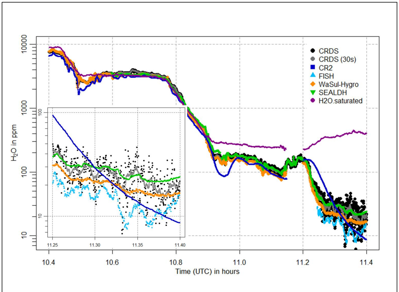
Figure 8: Water vapor mole fractions measured by the CRDS analyzer (black points, 30 seconds mean as grey points), the CR-2 (dark blue squares) and FISH (light blue triangles) instruments, as well as the WaSul-Hygro (orange diamonds) and SEALDH-I (green triangles) analyzers, for a time period during the flight on 31 May 2011. An enlarged section for the time period from 11:15 to 11:24 is shown in the lower left part of the plot.
