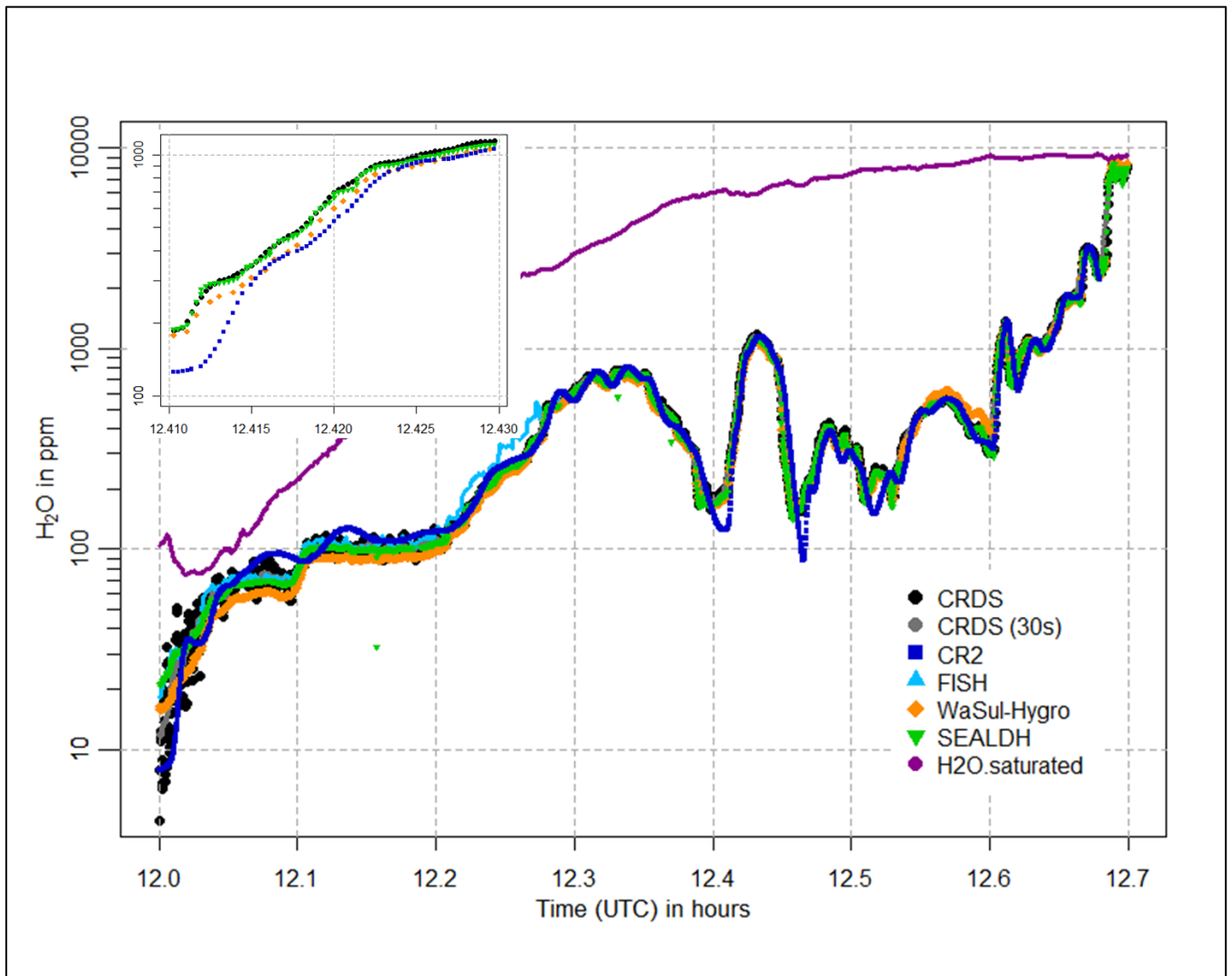
Figure 9: Same as Fig. 8, but for a time period during the flight on 1 June 2011. An enlarged section for the time period from 12:24:36 to 12:25:48 is shown in the upper left part of the plot. Here the water vapor increases in one minute about an order of magnitude from 200 to 1200 ppm.
