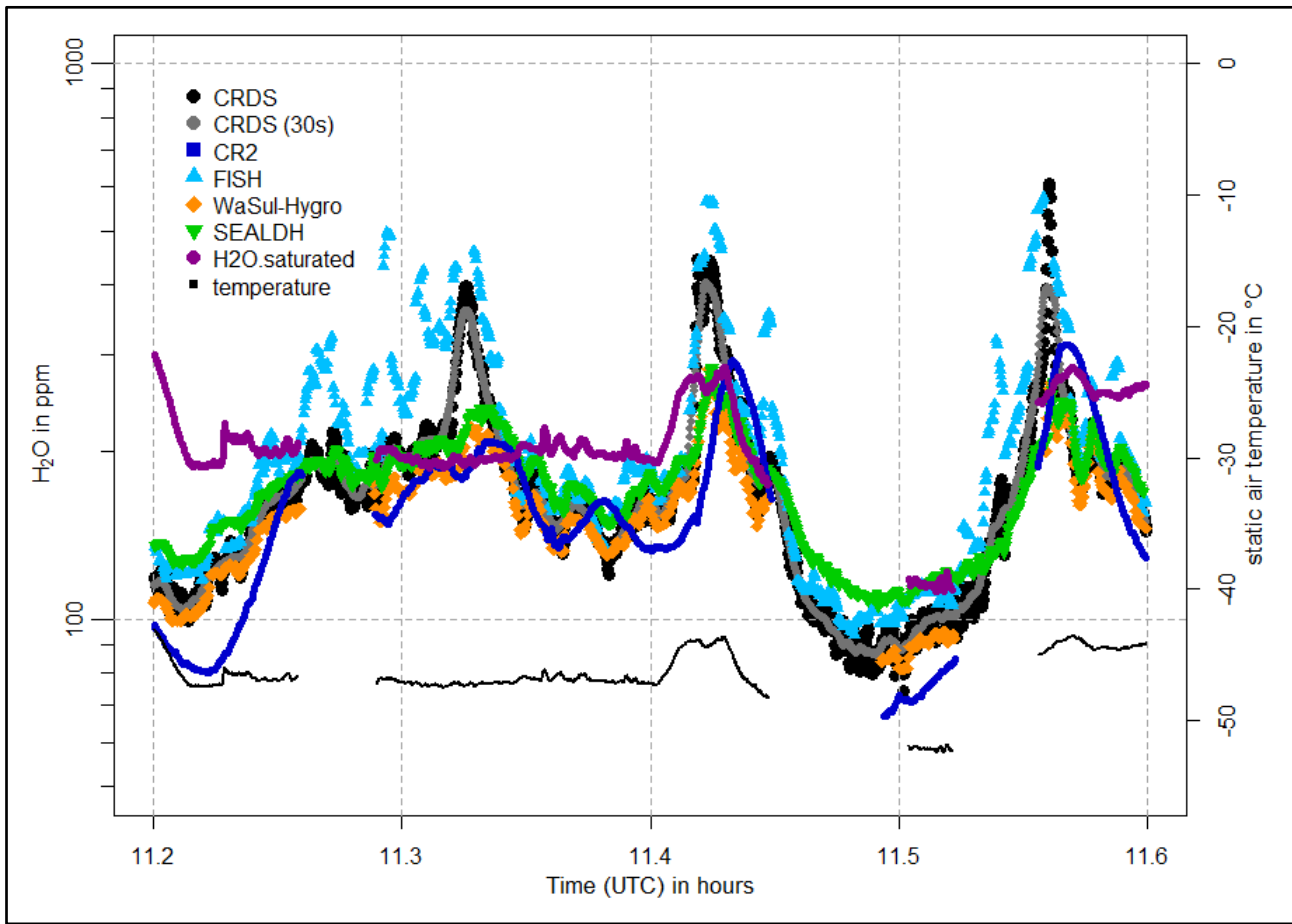
Figure 12: Water vapor mole fractions from the CRDS analyzer (black points, 30 seconds mean as grey points), the CR-2 (dark blue squares) and FISH (light blue triangles) instruments, as well as the WaSul-Hygro (orange diamonds) and SEALDH-I (green triangles) analyzers, during the flight on 1 June 2011, in the presence of clouds. Also shown are the water vapor mole fraction corresponding to saturation (violet points) and the static air temperature (black line).
