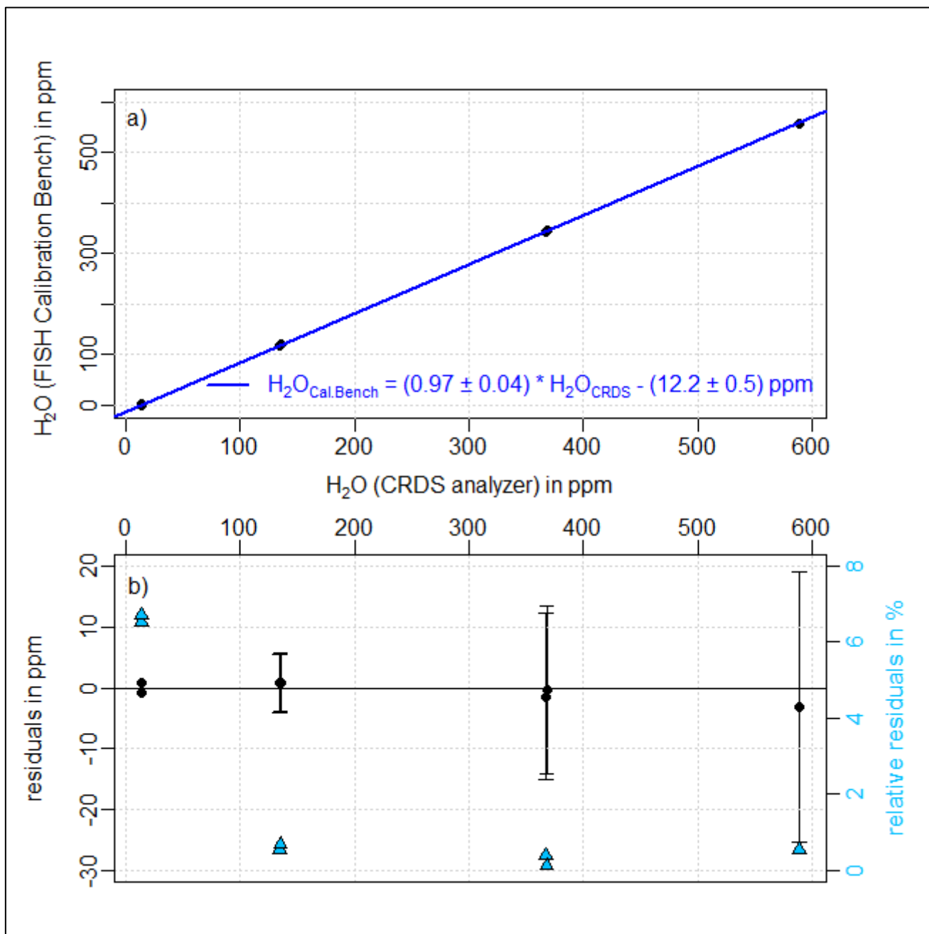
Figure 5: a) Dry air water vapor mole fractions measured by the CFKB2004 CRDS analyzer and the FISH calibration bench during a comparison in 2011. The CRDS data are offset corrected and calibrated according to the 2013 comparison against a dew point mirror. The corresponding fit is shown in blue. Residuals (difference between water vapor mole fractions measured by FISH calibration bench and the linear fit) can be seen in the plot (b). Error bars indicate the uncertainty range of the calibration bench of 4 %. The relative residuals are plotted on the right axis as light blue triangles.
