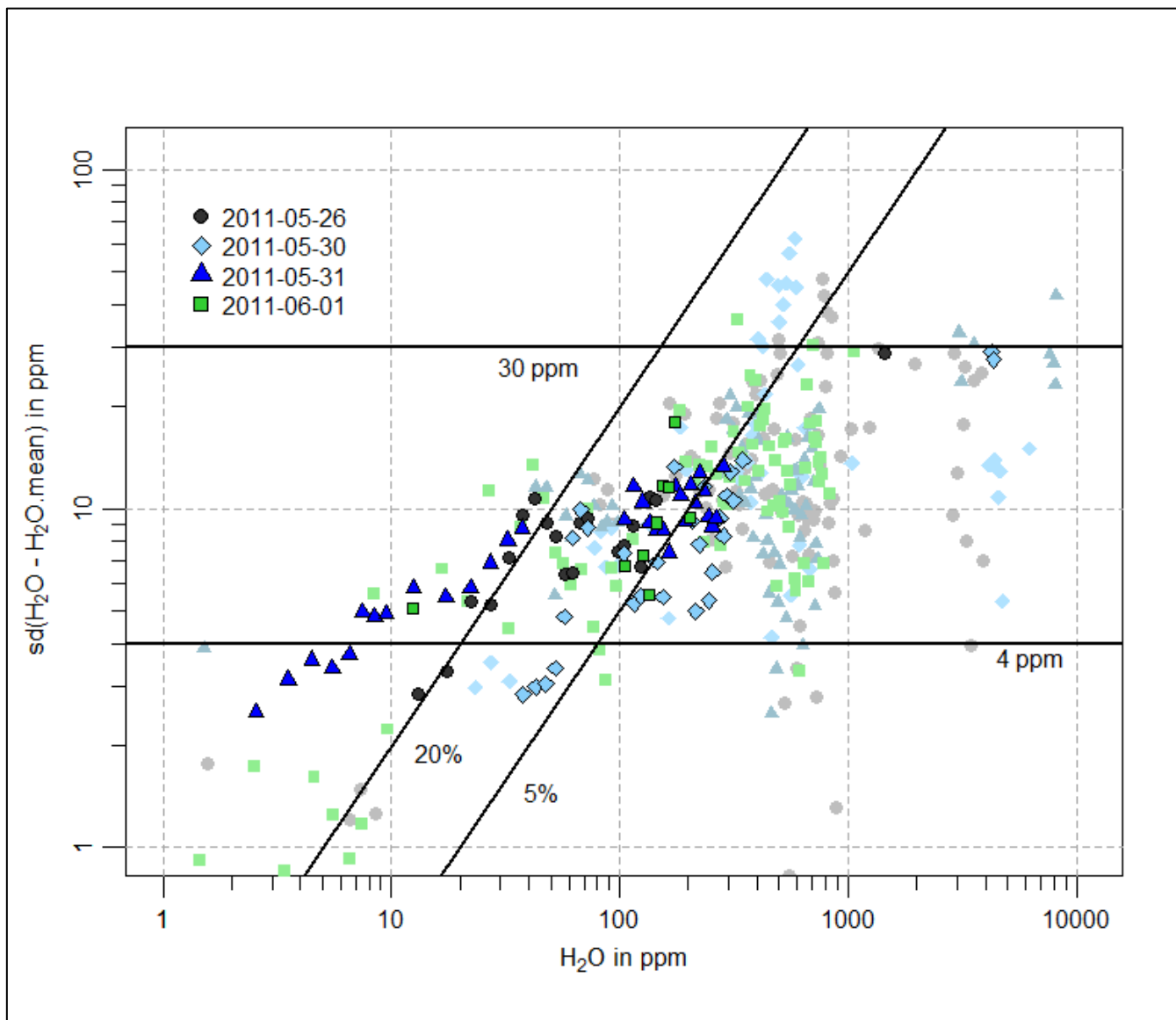
5 Figure 7: Standard deviation of the difference between the 0.4 Hz CRDS flight data and the 60 second averages, averaged for intervals of 1 ppm, 5 ppm, 10 ppm, and 100 ppm water vapor in the corresponding water vapor ranges of 0-10 ppm, 10-100 ppm, 100-1000 ppm, 1000-10000 ppm, respectively. Different colors and symbols indicate different flights. Results with higher priority are highlighted. The horizontal and diagonal black lines indicate standard deviations of 4 and 30 ppm, and 5 and 20 % respectively.
