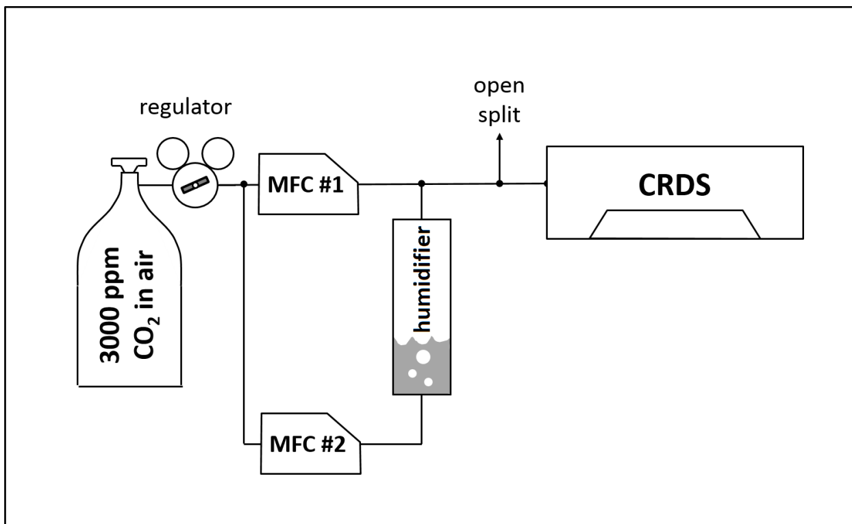
Figure 2: Experimental setup for the water vapor calibration by the CO 2 dilution effect. MFC #1 and 2 are mass flow controllers.
