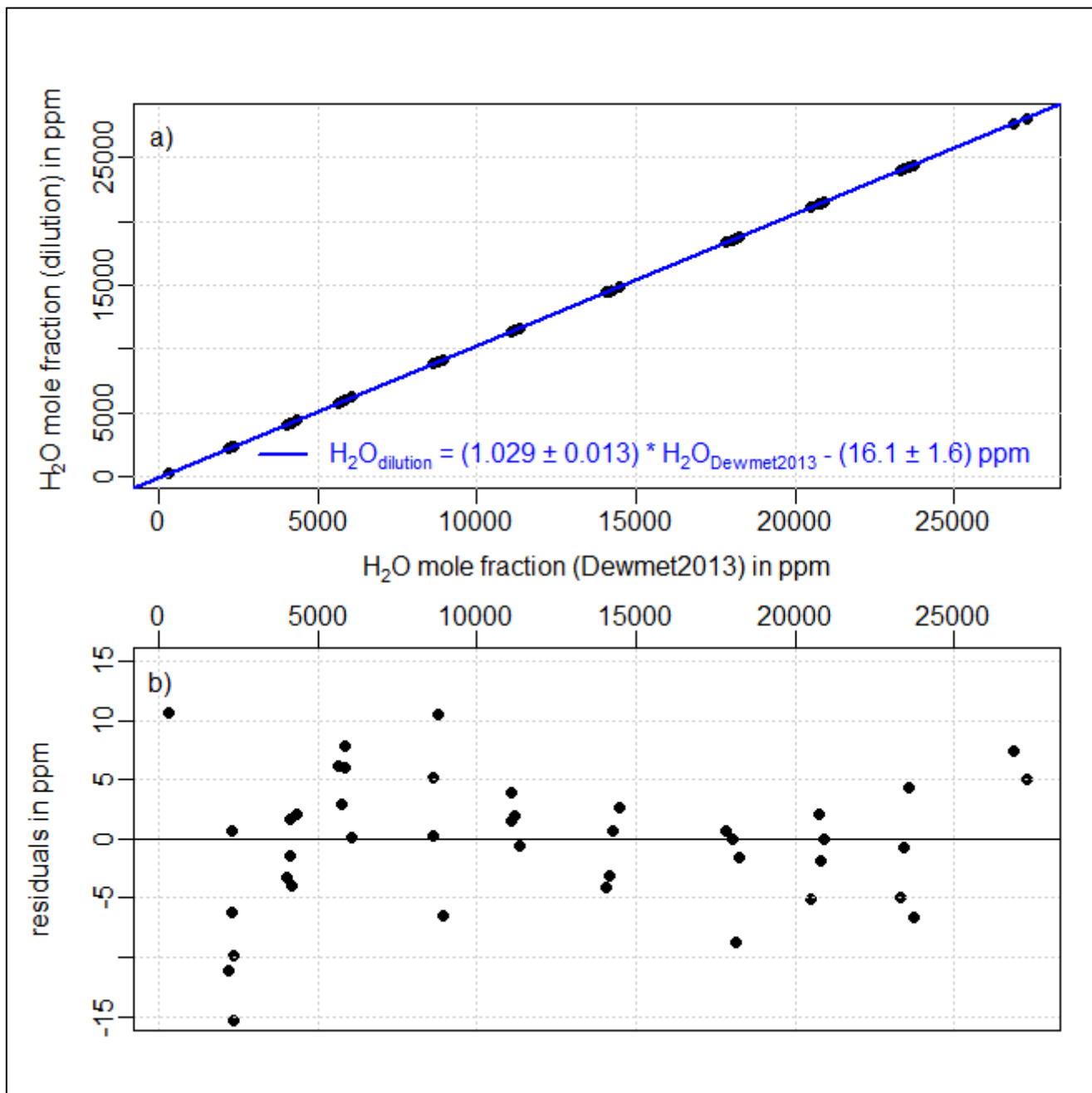
5 Figure 6: a) Water vapor mole fraction based on the CO 2 dilution method plotted against the water vapor mole fraction measurement from the CRDS analyzer (offset corrected and calibrated according to the comparison against a dew point mirror in 2013) during the fine scan experiment. The corresponding fit is shown in blue. Residuals (difference between water vapor mole fraction based on dilution method and the linear fit) can be seen in plot (b).
