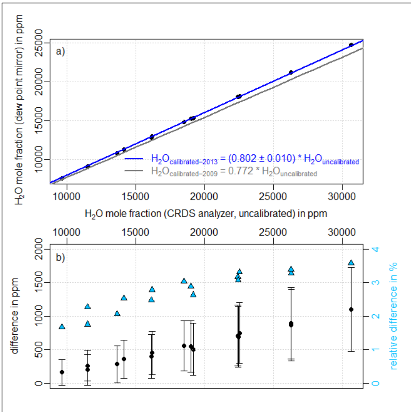
Figure 3: a) Uncalibrated water vapor measurements from the Picarro CRDS analyzer (CFKBDS2003) against the measurements from the dew point mirror (Dewmet TDH) during the 2013 calibration. The corresponding fit is shown as blue line, the calibration curve of the 2009 comparison as a grey line. The uncertainty of the fitted slope is composed of the fitting error and the uncertainty of the dew point mirror. b) Water vapor difference between the 2009 and 2013 experiments. The error bars indicate the uncertainty range, which results from the combination of the dew point mirror uncertainties during the 2009 and the 2013 calibration. The relative differences are plotted on the right axis as light blue triangles.
