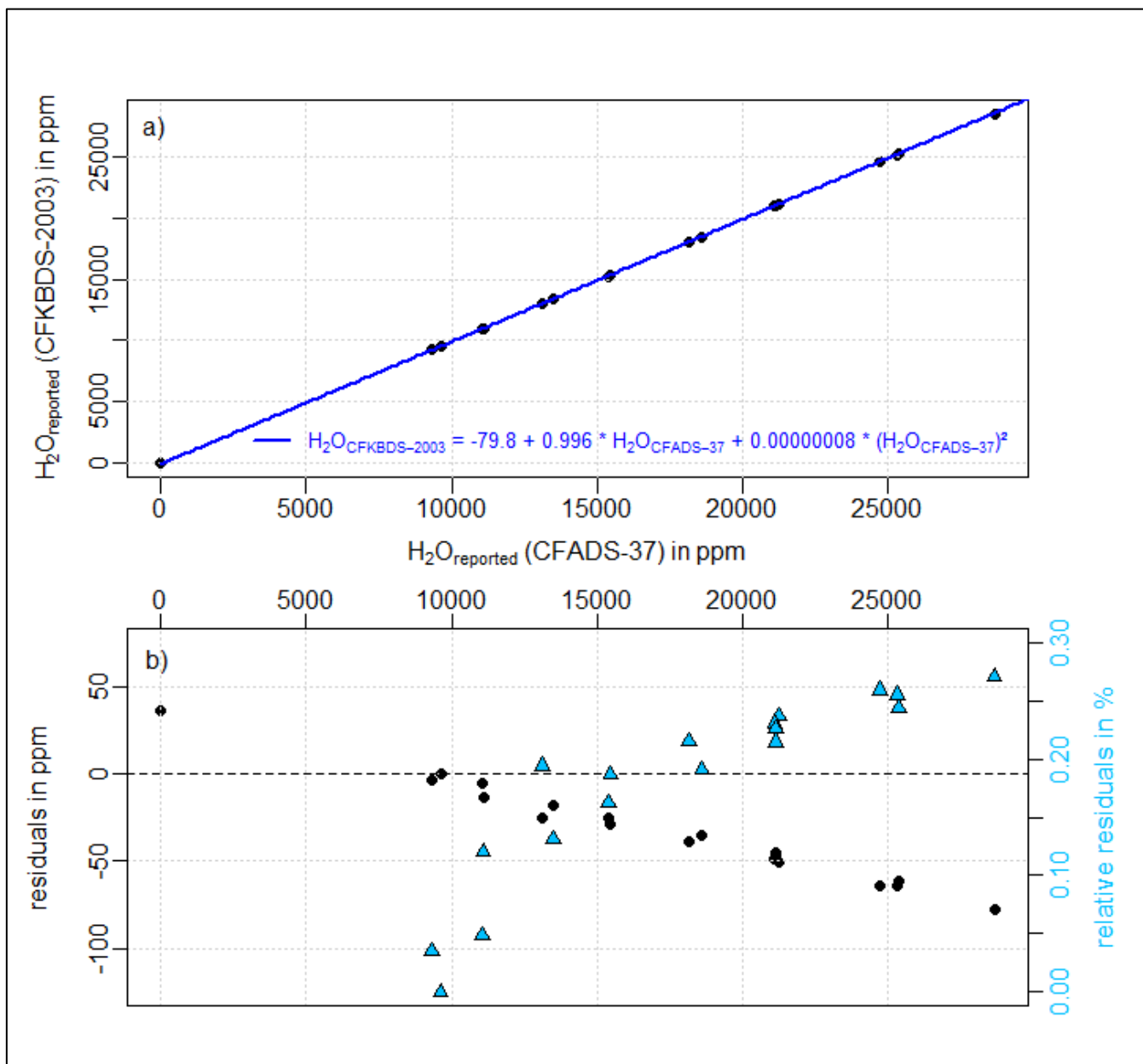
Figure 4: a) Uncalibrated water vapor mole fractions from the two Picarro CRDS analyzers CFADS37 and CFKBDS2003 during a comparison experiment in 2014 (black points). The blue line indicates the quadratic fit of an earlier comparison between the same instruments in 2011. The differences between the two comparisons, thus the drift of the two analyzers over the three years from 2011 to 2014, are shown in plot (b). The relative residuals are plotted on the right axis as light blue triangles. Since the analyzers were not offset corrected before the experiment, the relative difference of 800 % of the data point at 4.5 ppm is less meaningful and is therefore not shown in order to improve the clarity of the plot.
