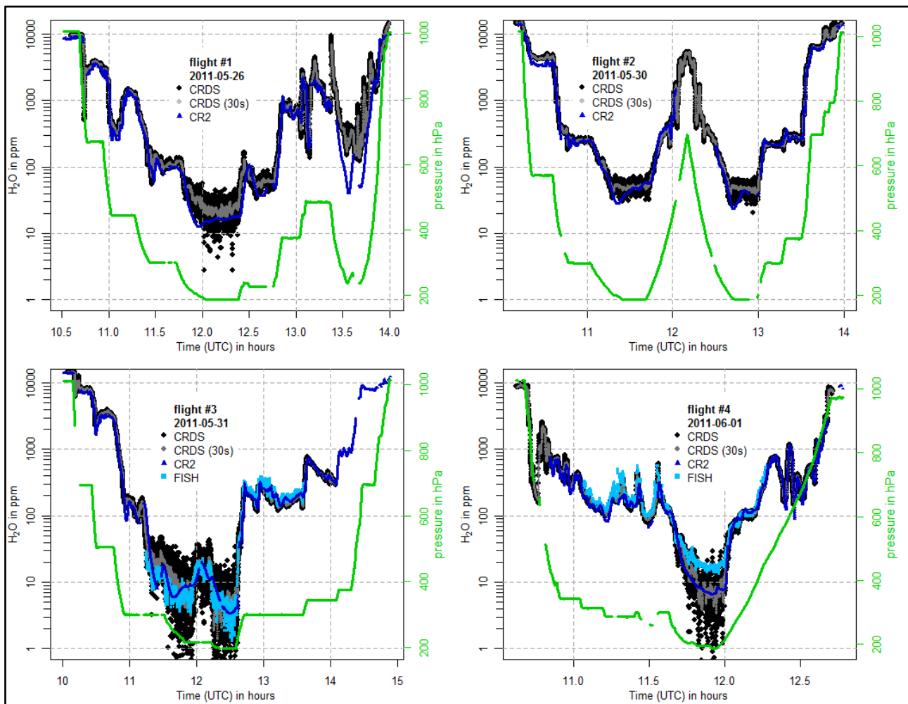
Figure 10: In-flight water vapor data from the CRDS analyzer (in black, 30 seconds mean in grey) and the reference instruments CR-2 (in dark blue) and FISH (in light blue) for the four flights on 26 May, 30 May, 31 May, and 1 June 2011. The corresponding atmospheric pressure levels are shown in green. The CRDS data are offset corrected and calibrated according to the 2013 dew point mirror comparison.
