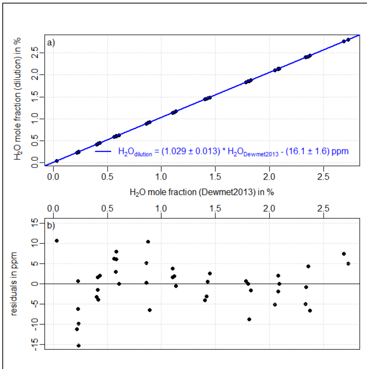
5 Figure 6: a) Water vapor mole fraction based on the CO 2 dilution method plotted against the water vapor mole fraction measurement of the CRDS analyzer (offset corrected and calibrated according to the comparison against a dew point mirror in 2013) during the fine scan experiment. The corresponding fit is shown in blue. Residuals (difference between water vapor mole fraction based on dilution method and the linear fit) can be seen in plot (b).
