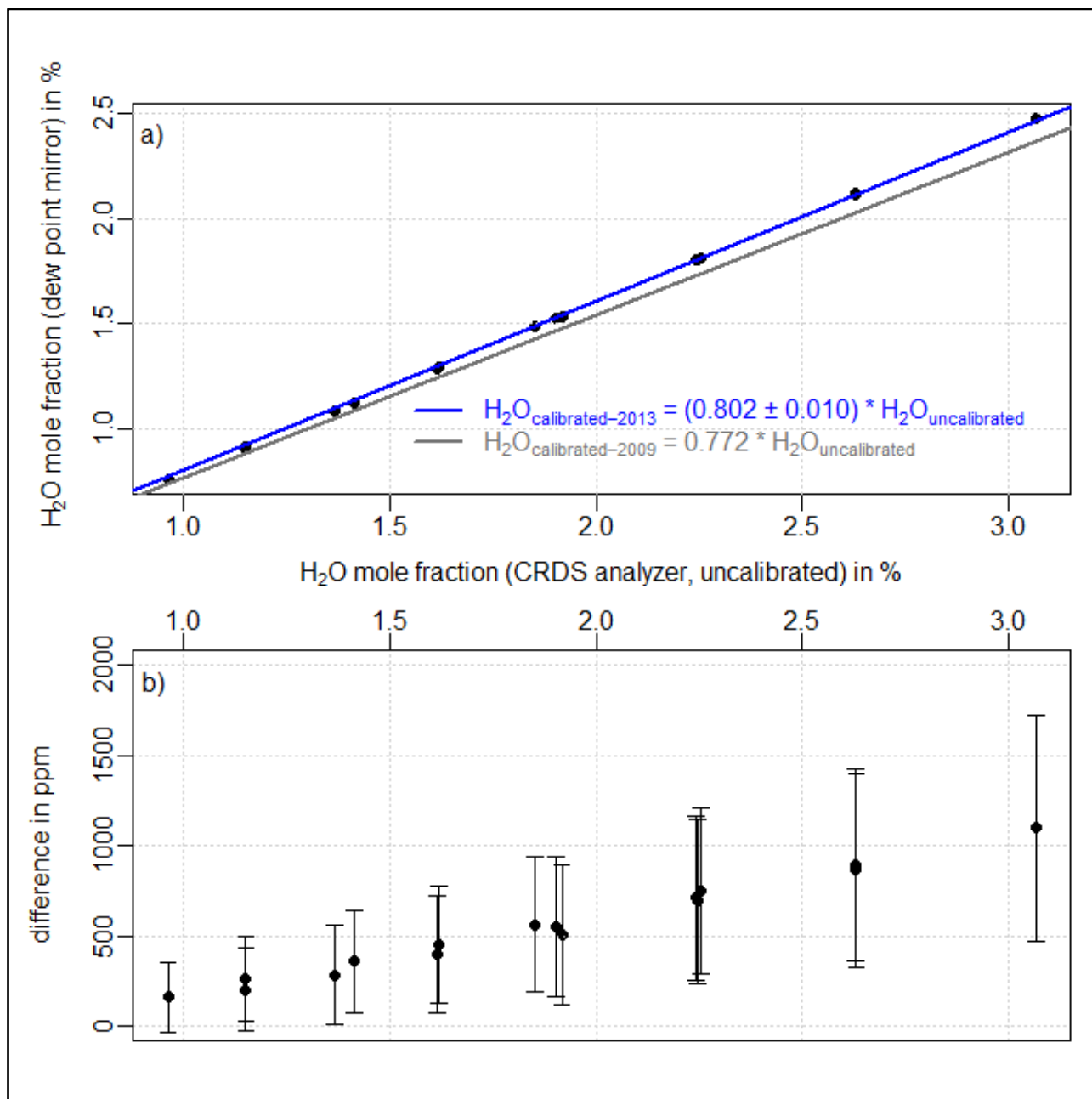
5 Figure 3: a) Uncalibrated water vapor measurements of the Picarro CRDS analyzer (CFKBDS2003) against the measurements of the dew point mirror (Dewmet TDH) during the 2013 calibration. The corresponding fit is shown as blue line, the calibration curve of the 2009 comparison as a grey line. The uncertainty of the fitted slope is composed of the fitting error and the uncertainty of the dew point mirror. b) Water vapor difference between the 2009 and 2013 experiments. The error bars indicate the uncertainty range, which results from the combination of the dew point mirror uncertainties during the 2009 and the 2013 calibration.
