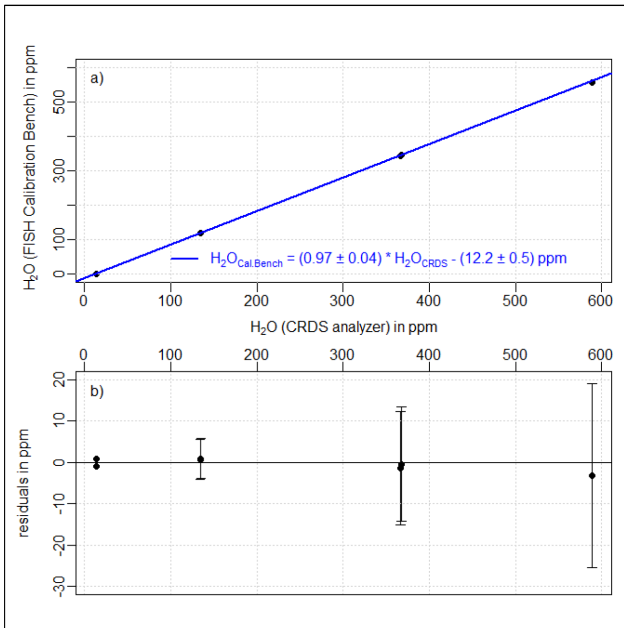
5 Figure 5: a) Dry air water vapor mole fractions measured by the CFKB2004 CRDS analyzer and the FISH calibration bench during a comparison in 2011. The CRDS data are calibrated according to the 2013 comparison against a dew point mirror. The corresponding fit is shown in blue. Residuals (difference between water vapor mole fractions measured by FISH calibration bench and the linear fit) can be seen in the plot (b). Error bars indicate the uncertainty range of the calibration bench of 4 % (rel.).
