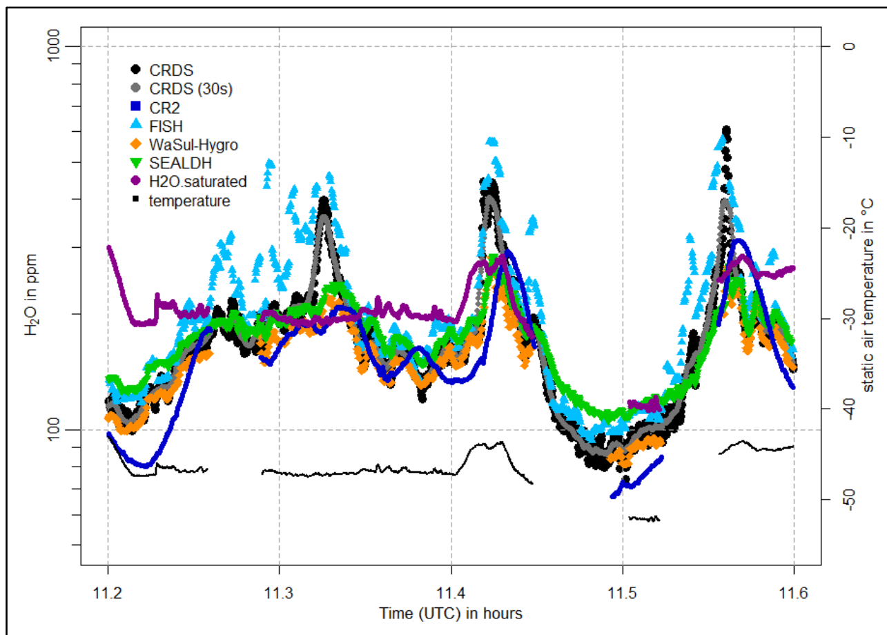
5 Figure 12: Water vapor mole fractions of the CRDS analyzer (offset corrected and calibrated according to the 2013 dew point mirror comparison) (black points, 30 seconds mean as grey points), the CR-2 (dark blue squares) and FISH (light blue triangles) instruments, as well as the WaSul-Hygro (orange diamonds) and SEALDH-I (green triangles) analyzers, during the flight on 1 June 2011, in the presence of clouds. Also shown are the water vapor mole fraction corresponding to saturation (violet points) and the static air temperature (black line).
