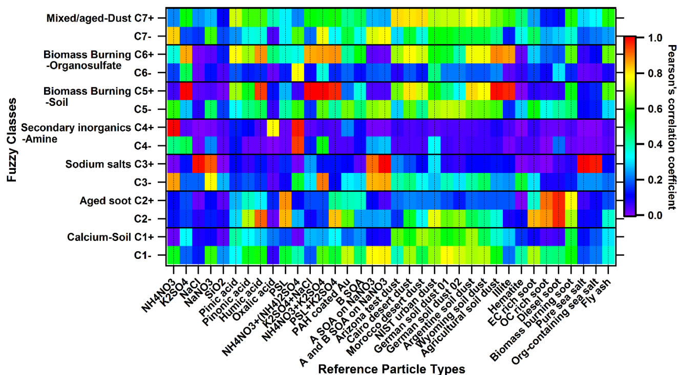
Figure 5: Correlation diagram of fuzzy classification results (7 classes, C1 to C7) and 36 laboratory-based reference spectra. Correlation results for the positive and negative spectra (e.g., for C1) are in the separated rows (e.g., C1+ and C1-). PAH is short for poly(allylamine hydrochloride), B SOA is short for biogenic SOA ( \alpha -pinene SOA in this study), A SOA is short for anthropogenic SOA (toluene SOA in this study), biomass burning soot is the lignocellulosic char from Chestnut wood. Note that, the strong and good correlations mentioned in the paper stand for Pearson's correlation coefficient \gamma \geq 0.8 and \gamma \geq 0.6 , respectively. The seven classes are class 1 "Calcium-Soil"; class 2 "Aged soot"; class3: "Sodium salts"; class 4 "Secondary inorganics-Amine"; class 5 "Biomass burning-Soil"; class 6 "Biomass burning-Organosulfate"; and class 7 "Mixed/aged-Dust".
