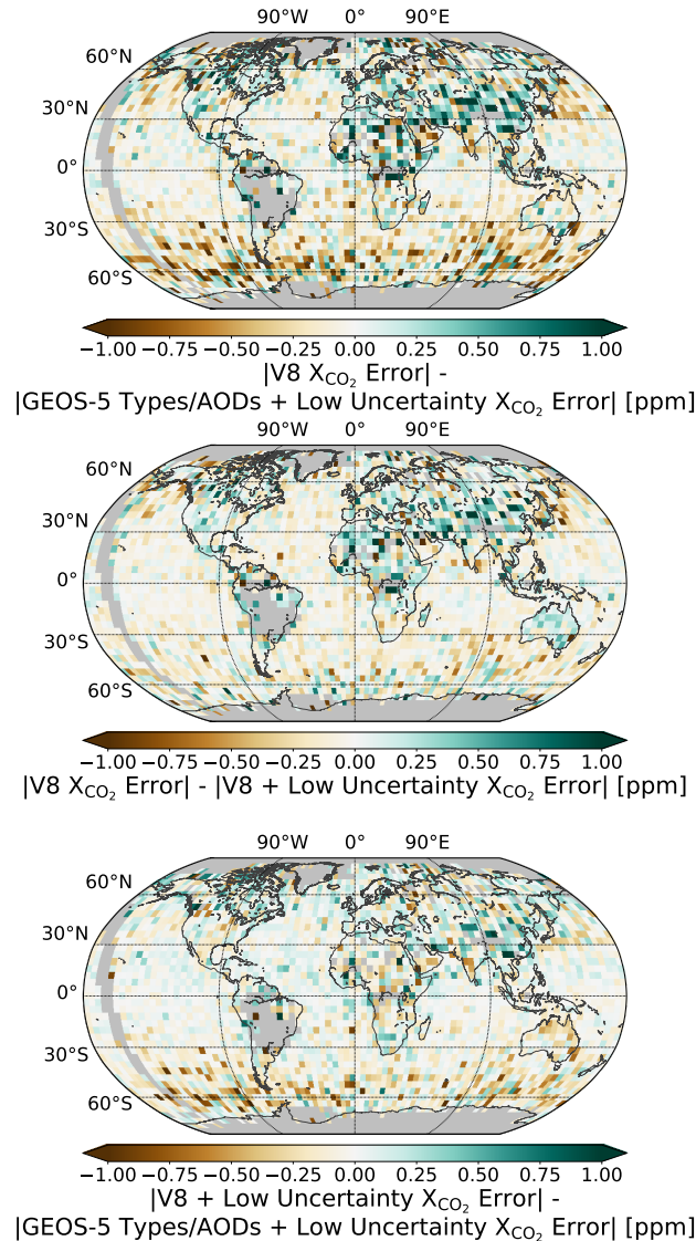
Figure 8. Top: 4x4 degree binned absolute value of V8 X_{CO_2} error against the model validation minus the absolute value of the GEOS-5 Types-types and AODs with low uncertainty X_{CO_2} error against the model validation. Middle: 4x4 degree binned absolute value of V8 X_{CO_2} error against the model validation minus the absolute value of V8 with low uncertainty X_{CO_2} error against the model validation. Bottom: 4x4 degree binned absolute value of V8 with low uncertainty X_{CO_2} error against the model validation minus the absolute value of GEOS-5 Types-types and AODs with low uncertainty X_{CO_2} error against the model validation. Green grid cells represent an improvement relative to the model validation while brown grid cells represent a worse comparison to the model validation. Grey bins represent no data.
