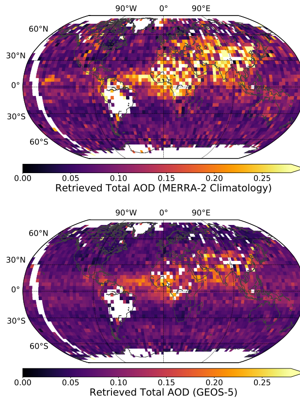
Figure 10. Top: 4x4 degree binned retrieved AOD for V8. Bottom: 4x4 degree binned retrieved AOD for V8 + GEOS-5 Types-types and AODs with low uncertainty. White bins represent no data.
