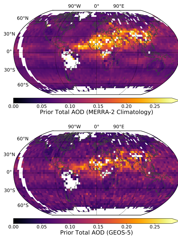
Figure 9. Top: 4x4 degree binned prior AOD for V8, derived from a MERRA-2 monthly climatology. Bottom: 4x4 degree binned prior AOD for V8 + GEOS-5 Types-types and AODs with low uncertainty, derived from co-located GEOS-5 AODs. White bins represent no data.
