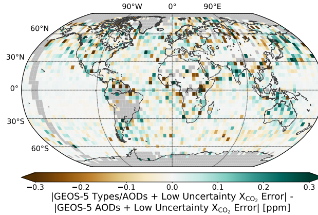
Figure 11. 4x4 degree binned absolute value of GEOS-5 types and AODs with low uncertainty X_{\text{CO}_2} error against the model validation minus the absolute value of GEOS-5 AODs with low uncertainty X_{\text{CO}_2} error against the model validation. Green grid cells represent an improvement relative to the model validation while brown grid cells represent a worse comparison to the model validation. Grey bins represent no data.
