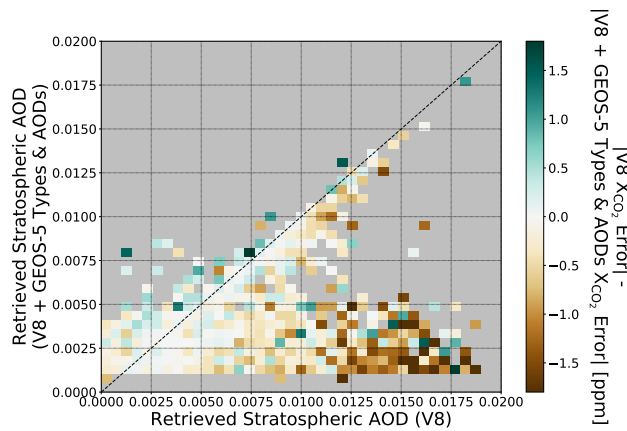
Figure 12. Retrieved stratospheric AOD from V8 versus retrieved stratospheric AOD from V8 + GEOS-5 types and AODs with low uncertainty for the Southern Ocean. Color represents the change in the absolute value of the X_{\text{CO}_2} error between the two retrieval types, where green demonstrates an improvement over V8 and brown represents a worsening.
