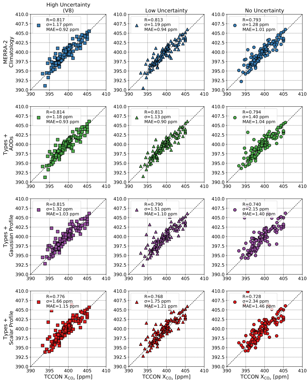
Figure 6. Retrieved OCO-2 X_{\text{CO}_2} (y-axes) against TCCON X_{\text{CO}_2} (x-axes). Overpass means are plotted. The first row is the operational retrieval (V8). The second row is ingesting GEOS-5 types and AODs, the third row is ingesting GEOS-5 types and Gaussian profile priors, and the fourth row is ingesting GEOS-5 types and solving for a scalar to the prior aerosol profile. The left column is high uncertainty, the middle column is low uncertainty, and the right column is no uncertainty (see Table 2). For each panel, R is the correlation coefficient, \sigma is the standard deviation of the error against TCCON, and MAE is the mean absolute error against TCCON. The TCCON sites used are listed in Table 1, shown in Fig. 2, and were required to have valid data between 17 September 2014 and 2 May 2016.
