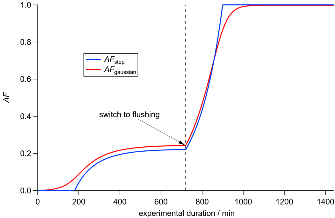
Figure 5: Global AF response functions inside a CSTR for a uniform aerosol population (blue line) and an aerosol population with an activation time distribution P(t_{act}) represented by a Gaussian distribution (red line).
