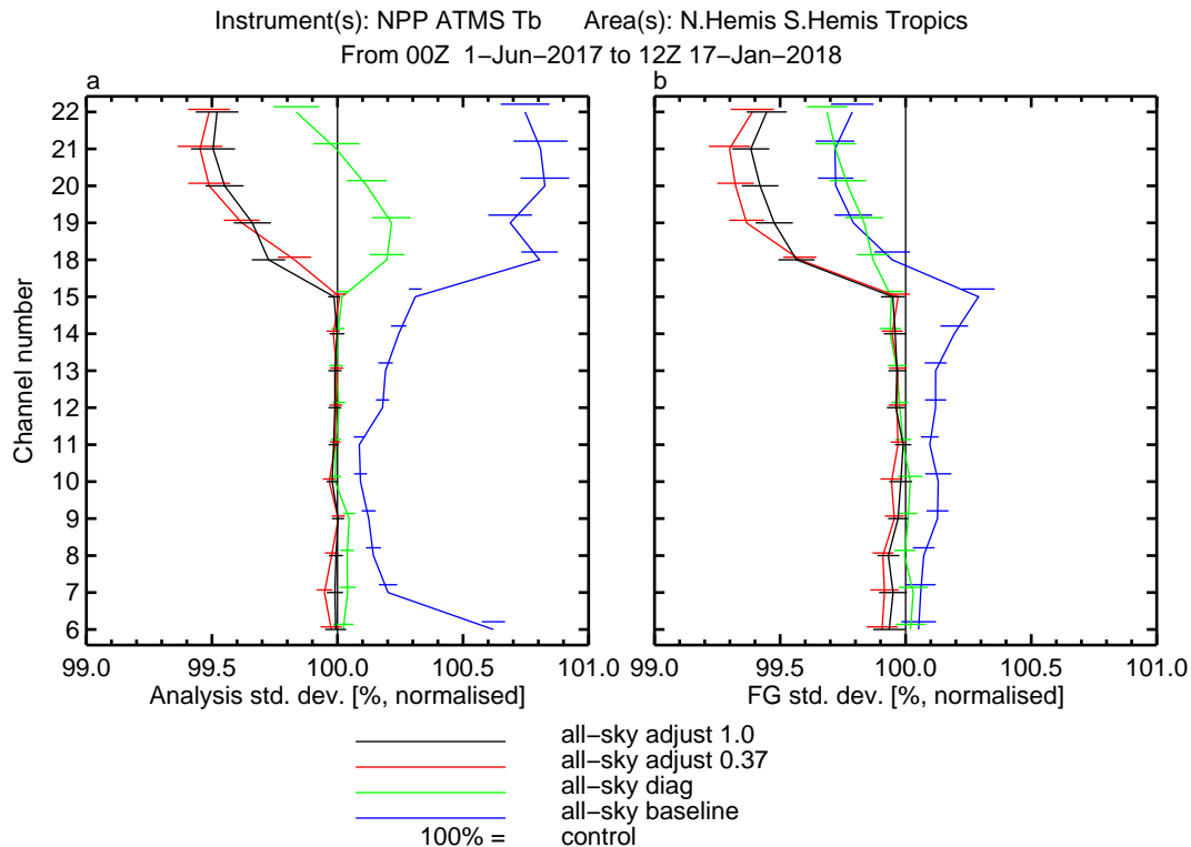
Figure 17. As Fig. 16 but for a set of experiments that inflate some of the trailing eigenvalues.
