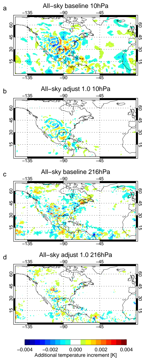
Figure 20. Additional temperature increments generated by all-sky IR assimilation on top of the otherwise full observing system, at 00Z on 1st June 2017 at the beginning of the experiments where the background is identical across all experiments.
