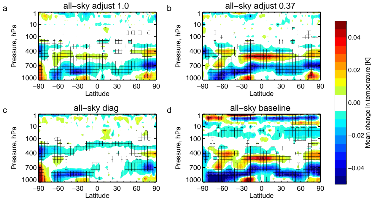
Figure 18. Mean change in zonal mean temperature analysis between experiments and the control. Cross-hatching indicates 95% confidence with Sidak correction for 20 independent tests.
