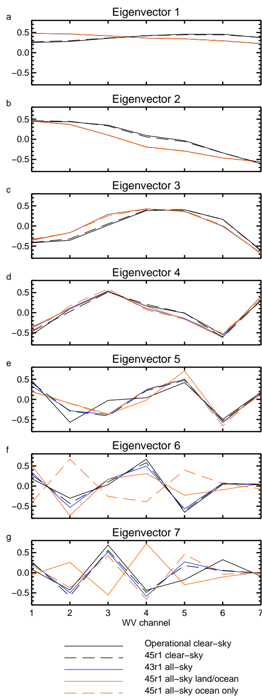
Figure 3. Eigenvectors of possible observation error covariance matrices for the 7 assimilated IASI upper-tropospheric water vapour channels. Generally the black lines (clear-sky error matrices) are almost totally overlaid, and similarly the coloured lines (all-sky error matrices) are also often overlaid.
