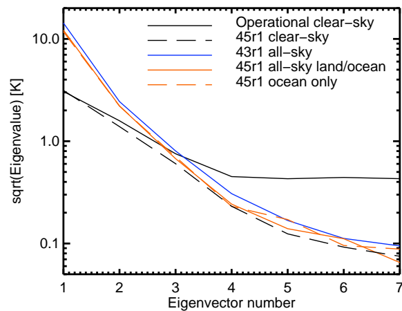
Figure 4. Square root of the eigenvalues associated with the eigenvectors in Fig. 3
