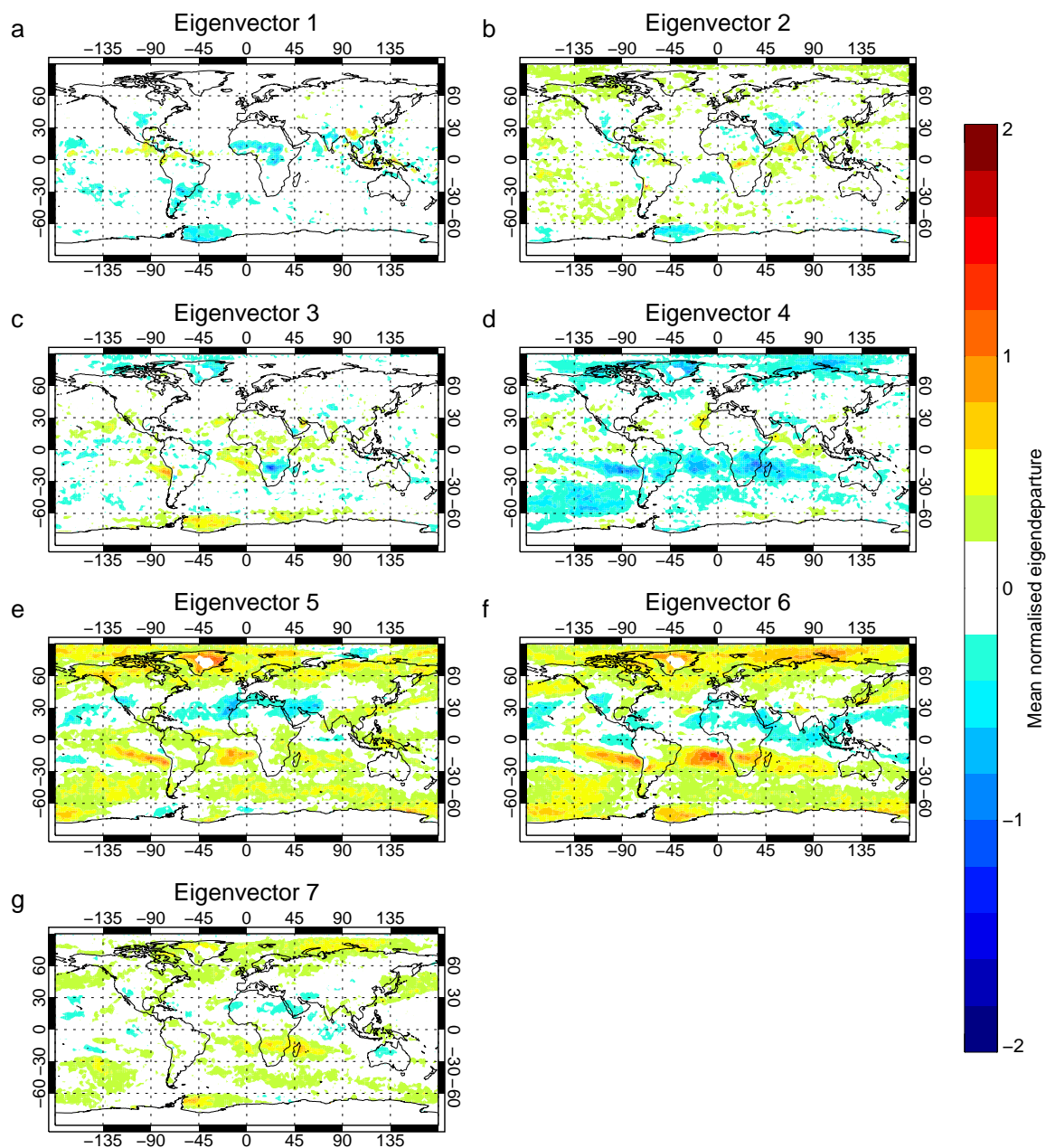
Figure 11. Mean mean normalised background eigendepartures, e_j^T d / (\lambda_j)^{0.5} , after bias correction. Based on a sample of passive background departures from 1-20 June, 2017, as Fig. 10
