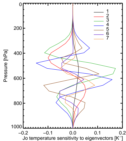
Figure 7. Temperature sensitivity of the Jo costfunction, by eigenvector ( \mathbf{H}^T \mathbf{E} \mathbf{A}^{0.5} ), showing (by comparison to Fig. 5b) the role of the eigenvalues of the error covariance matrix in amplifying sensitivities to smaller vertical wavelengths, and reducing sensitivities to broad vertical features.
