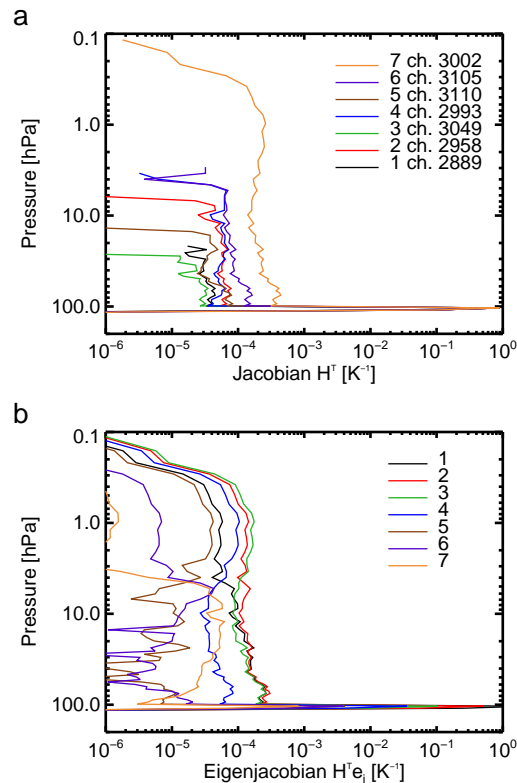
Figure 21. Temperature parts of the Jacobians h_i and eigenjacobians ( \mathbf{H}^T e_j ) for a tropical profile with an optically thick, full-coverage cloud placed exactly at the temperature tropopause.
