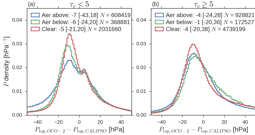
Figure 8. OCO-2 minus CALIPSO P_{top} statistics for Quality_flag = 0 cases, subset for aerosol layer above cloud (N~1.5×10 6 ), aerosol layer below cloud (N~0.5×10 6 ) or no aerosol layer detected (N~6.8×10 6 ) by CALIPSO's 05kmALay. Legend reports median [14 th , 18 th percentiles]. (a) clouds with posterior \tau < 5 , (b) clouds with posterior \tau \geq 5 .
