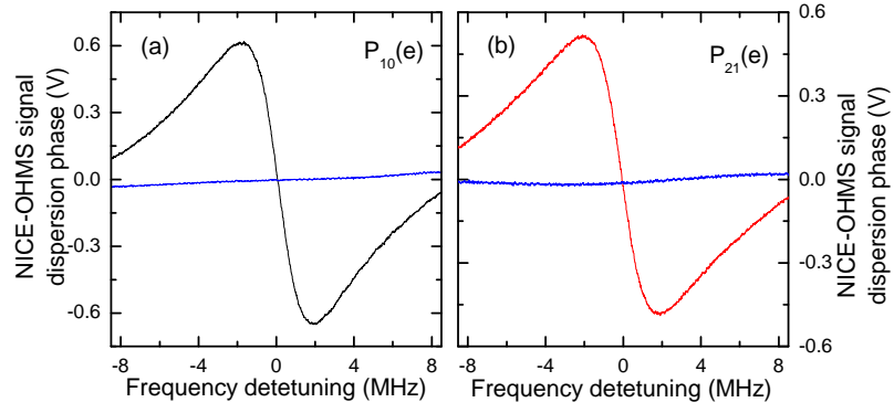
Figure 3: The sD NICE-OHMS signals detected at dispersion phase on the P_{10}(e) and P_{21}(e) transitions from 100 mTorr of acetylene detection by an EDFL and a WGM laser, respectively. The blue lines in both panels are the background signals when the cavity was evacuated.
