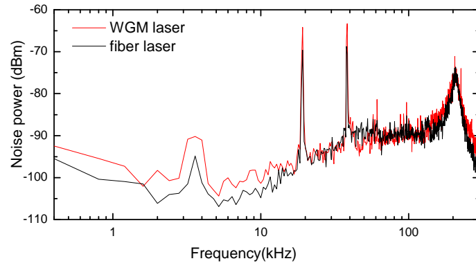
Figure 2: In loop frequency spectrum of the error signal of the PDH locking for EDFL (black curve) and WGM laser (red curve).
