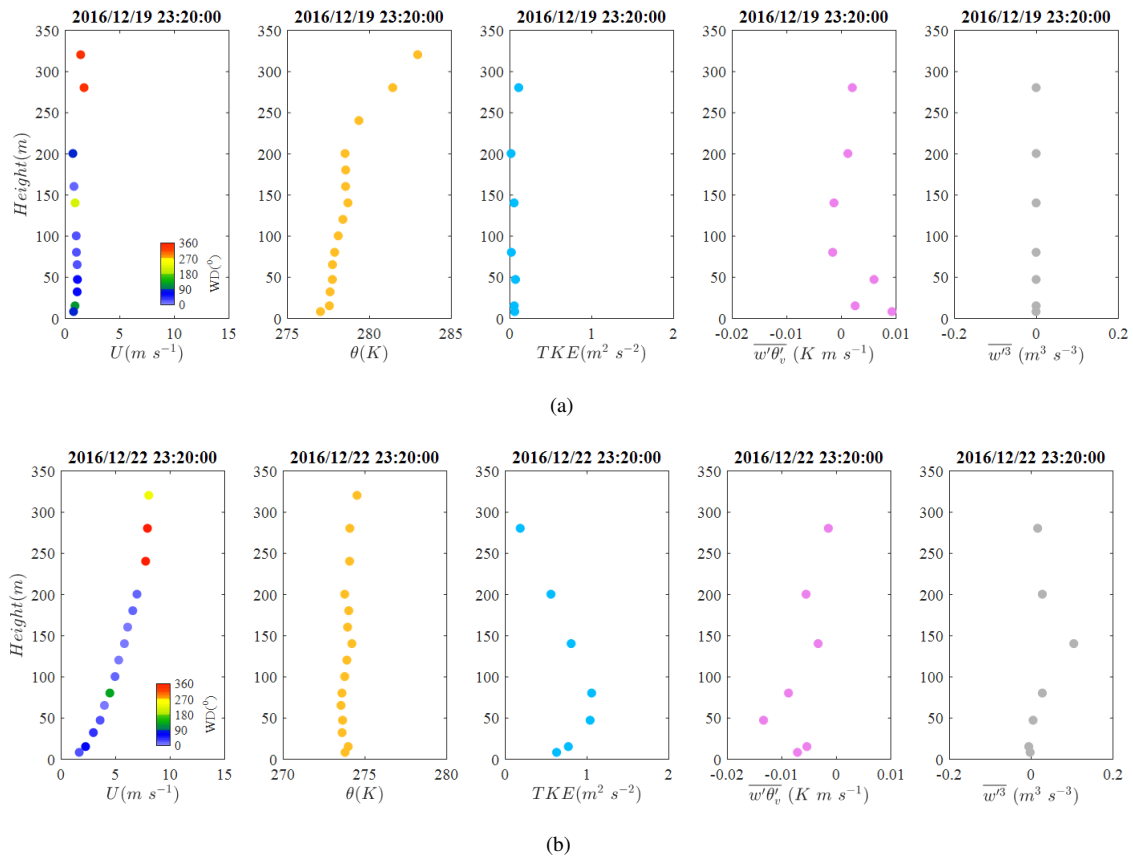
Figure 7. Vertical profiles of wind speed( U ),wind direction( WD ),potential temperature( \theta ),turbulent kinetic energy( TKE ), sensible heat flux( \overline{w'\theta'_v} ) and third order moment of vertical velocity( \overline{w'^3} ) at 23:20 on 19 December,2016(a)and 22 December,2016(b).
