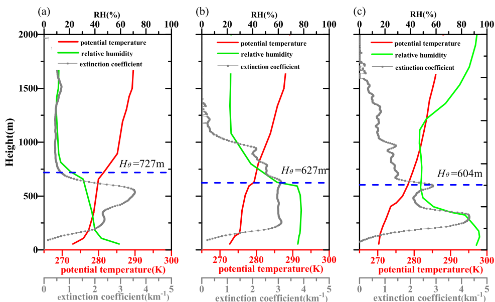
Figure 4. Vertical profiles measured at ZBAA meteorological station.(a) 20:00,16 December, 2016 (b)20:00, 17 December, 2016(c) 08:00 21 December,2016.Red line: potential temperature(K);Green line:RH(%);Grey line:extinction coefficient( \text{km}^{-1} );blue dotted line:ABL height determined by radiosonde expressed in H_{\theta} (m).
