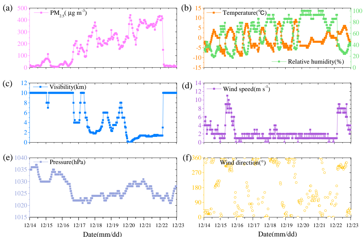
Figure 2. Time series of ground level PM_{2.5} (a),relative humidity and temperature(b),visibility(c),wind speed(d),surface pressure(e) and wind direction(f)during 14 to 22 December 2016,the units of those meteorological parameters are \mu\text{g m}^{-3} ,%, ^{\circ}\text{C} ,km, \text{m s}^{-1} ,hPa and ^{\circ} respectively.
