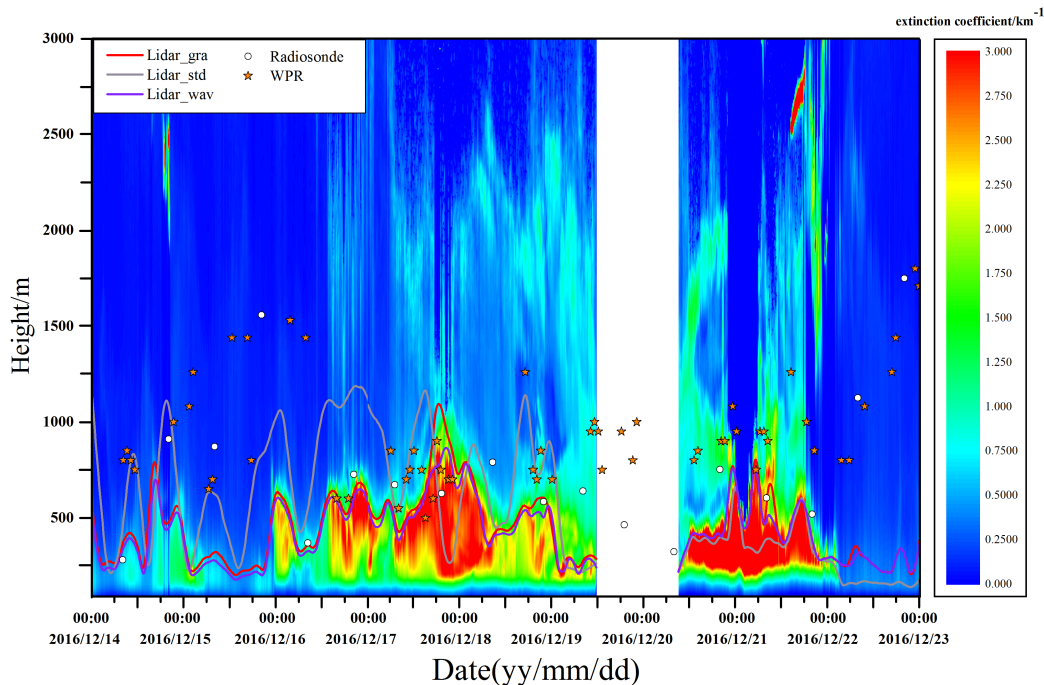
Figure 3. Temporal and spatial variation of extinction coefficient (shaded, unit: \text{km}^{-1} ) from 14 to 23 December, 2016 and ABL height (m) determined by different instruments. Red line (Lidar_gra), grey line (Lidar_std), purple line (Lidar_wav) represent ABL height determined by Lidar using gradient method, standard deviation method, and wavelet method respectively. White points: ABL height determined by radiosonde; Five-pointed star: ABL height determined by WPR. It should be noted that the blank part of the extinction coefficient is due to a technical failure, and the lidar data were missing from 11:00 on December 19 to 09:00 on December 20.
