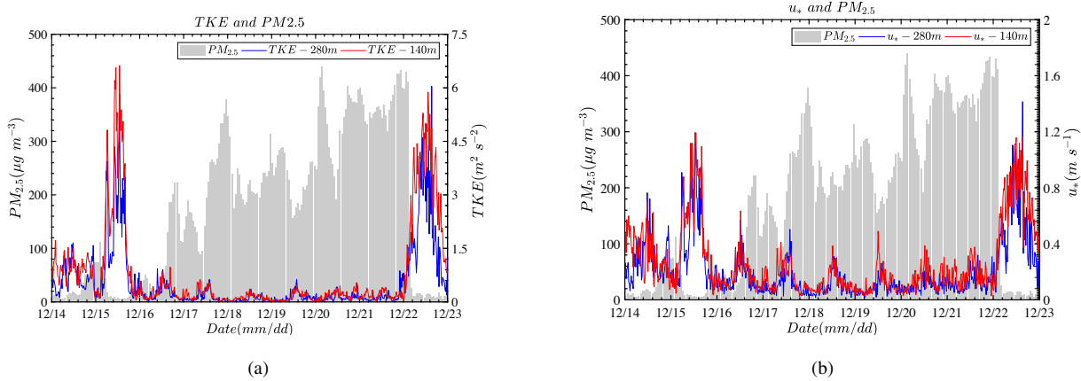
Figure 6. Time series of (a) turbulent kinetic energy ( m^2 s^{-2} ) and (b) friction velocity ( u_* , m s^{-1} ) at 140m (red line) and 280m (blue line), PM_{2.5} ( \mu g m^{-3} ) concentration are also drawn in the figures (grey column).
