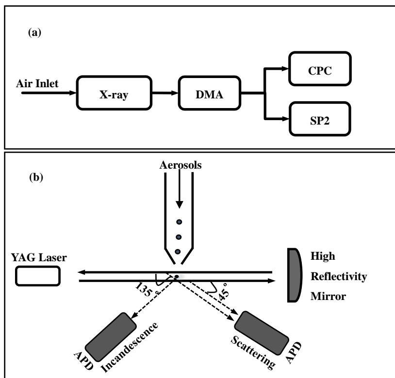
547 Figure 1. (a) Schematic of the measurement system. (b) Diagram of SP2 Chamber.
