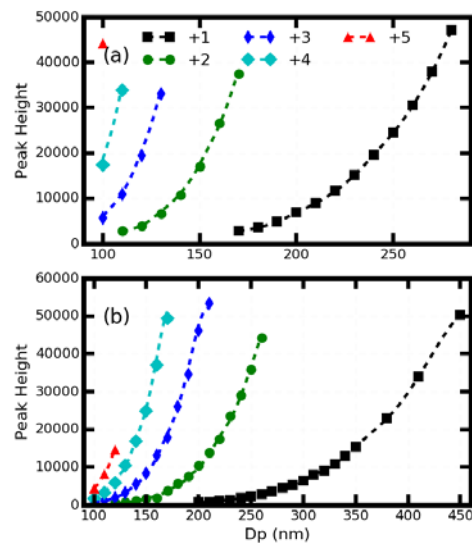
552 Figure 3. The geometric mean peak height for different diameters of the high gain channel. The 553 markers gives the measured values and the dotted line shows the theoretically calculated value. 554 Different colors represent the different number of elementary charges.
