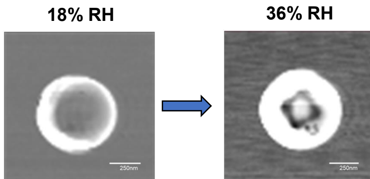
Figure S1. AFM phase images of 1:8 (M) glucose:NaCl particle at varying RH (left - 18% RH, right - 36% RH). Image from 36% RH shows greater contrast between the core and shell, which aided in OVF quantification.
