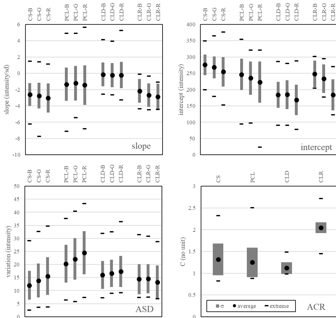
Figure 5. Photographic sky type properties. Slope and intercept (top row) for the radial fit; areal standard deviation (ASD) of brightness (bottom left); average colour ratio (ACR) (bottom right). Sky types were assigned visually. Black circles indicate the mean, grey boxes the range of the first standard deviation, black bars limit the extreme values found in the master table.
