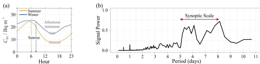
Figure 3: (a) Summer and winter diurnal composite hourly radon concentration, and (b) spectral analysis of the LjB hourly atmospheric pressure data for winter.
