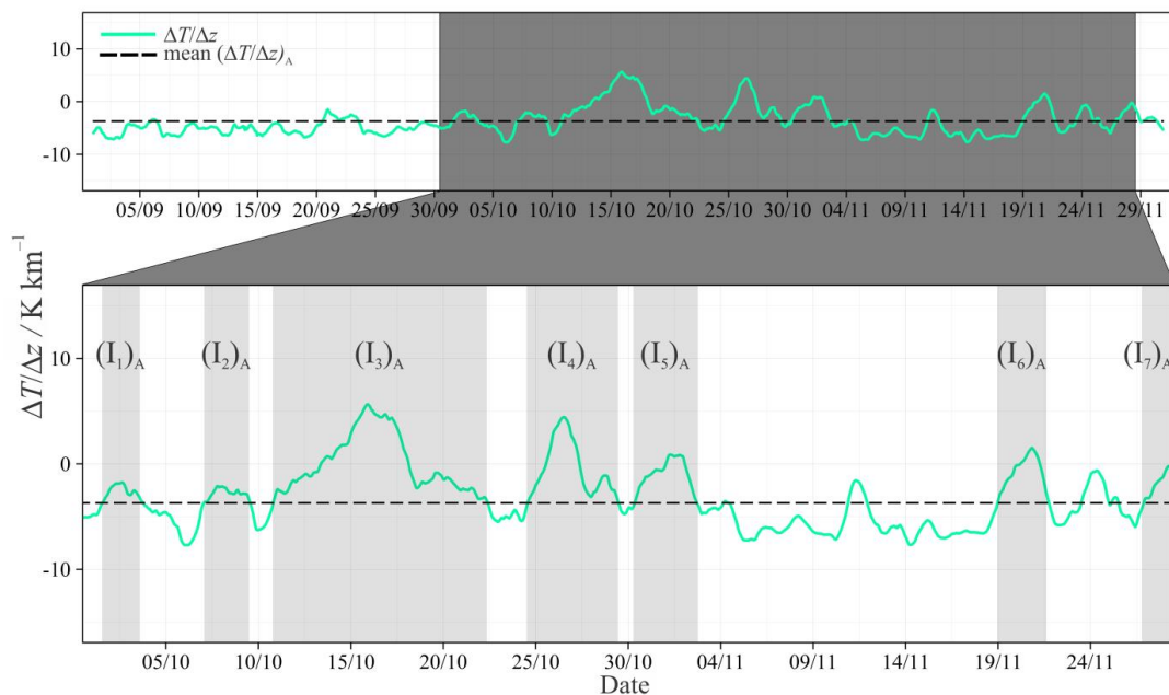
5 Figure 11: 24-h running mean of the pseudo-vertical temperature gradient in autumn; seven ‘persistent temperature inversion’ events (I)_A detected by the TGM are shown in the shaded section and enlarged in the breakout panel beneath; see text in section 2.3.2 for details.
