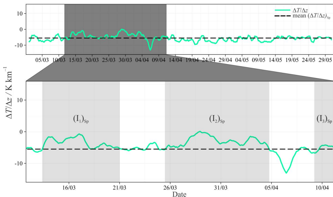
Figure 12: 24-h running mean of the pseudo-vertical temperature gradient in spring; three ‘persistent temperature inversion’ events (I)_{Sp} detected by the TGM are shown in the shaded area and enlarged in the breakout panel beneath; see text in section 2.3.2 for details.
