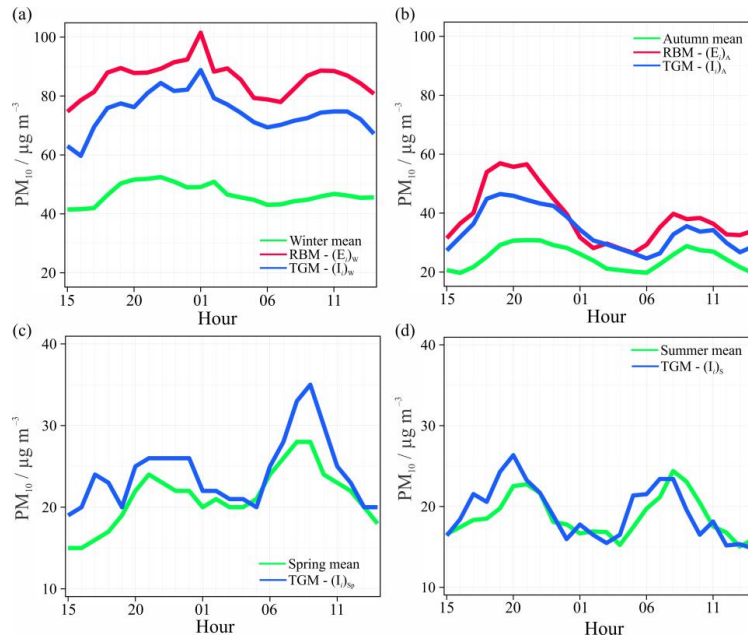
Figure 16: Diurnal PM_{10} composites, based on hourly means, for: (a) winter, (b) autumn, (c) spring, and (d) summer, for all conditions (seasonal mean) and for ‘persistent temperature inversion’ events detected by the RBM and TGM.
