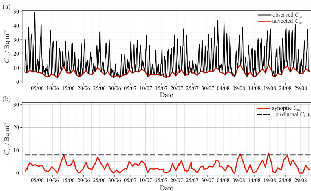
Figure 8: (a) Hourly mean observed radon concentrations with the advected contribution indicated, and (b) isolated synoptic timescale radon contribution in summer with the standard deviation of the diurnal contribution indicated. No ‘persistent temperature inversion’ events were detected by the RBM this season.
