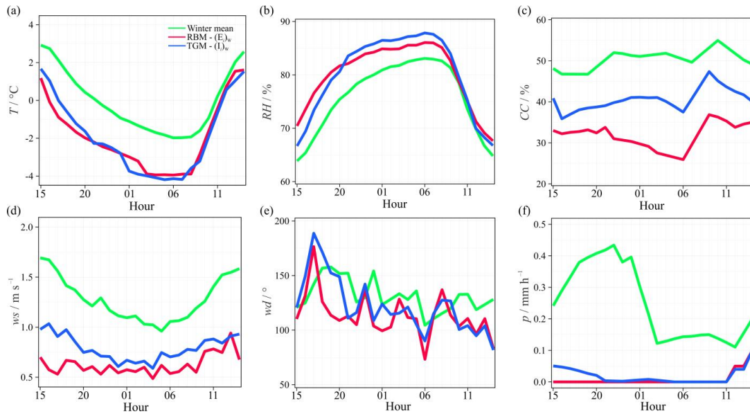
Figure 9: Diurnal composites, based on hourly means, of: (a) air temperature, (b) relative humidity, (c) cloud cover, (d) wind speed, (e) wind direction, and (f) precipitation, for winter mean, and ‘persistent temperature inversion’ events detected in winter by the RBM and TGM.
