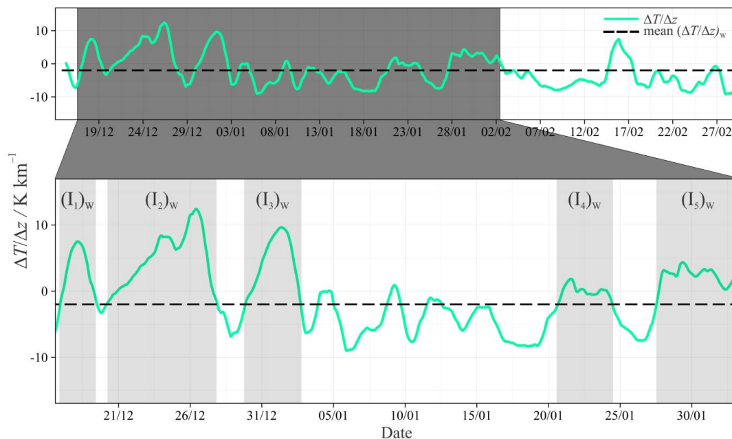
Figure 4: 24-h running mean pseudo-vertical temperature gradient in winter. Five ‘persistent temperature inversion’ events ( I_i ) w detected by the TGM are shown in the shaded area and enlarged in the breakout panel beneath; see text in section 2.3.2 for details.
