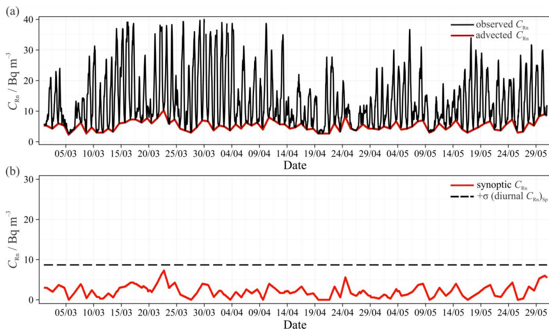
Figure 7: (a) Hourly mean observed radon concentrations with the advected contribution indicated, and (b) isolated synoptic timescale radon contribution in spring with the standard deviation of the diurnal contribution indicated. No ‘persistent temperature inversion’ events were detected by the RBM this season.
