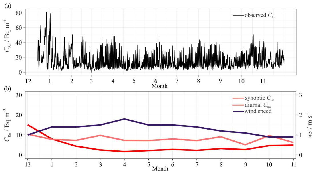
5 Figure 5: (a) One year (Dec–2016 to Nov–2017) of hourly radon concentration, and (b) monthly average of synoptic radon, diurnal mixing of radon, and wind speed.
