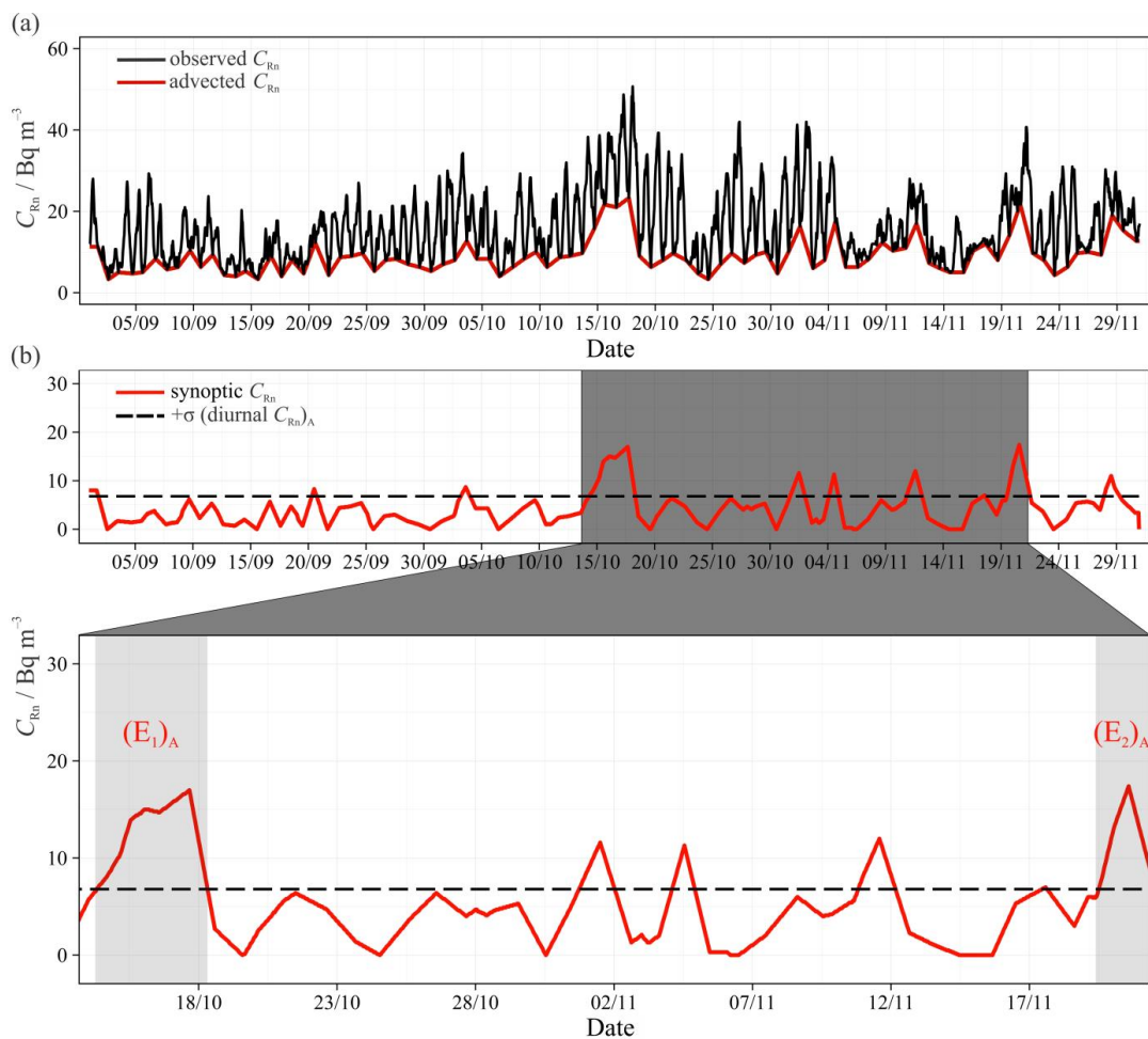
Figure 6: (a) Hourly mean observed radon concentrations with the advected contribution indicated, and (b) isolated synoptic timescale radon contribution in autumn with the standard deviation of the diurnal contribution indicated. Two ‘persistent temperature inversion’ events (E_i)_A detected by the RBM are shown in the shaded area and enlarged in the breakout panel beneath; see text in section 2.3.1 for details.
