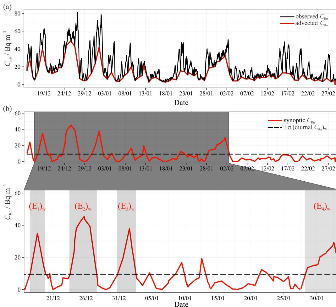
Figure 2: (a) Hourly mean observed radon concentrations with the advected contribution indicated, and (b) isolated synoptic timescale radon contribution in winter with the standard deviation of the diurnal contribution indicated. Four ‘persistent temperature inversion’ events (E)_w detected by the RBM are shown in the shaded area and enlarged in the breakout panel below; see text in section 2.3.1 for details.
