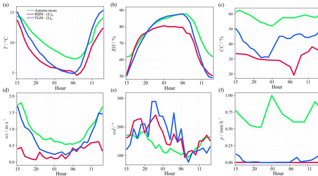
Figure 10: Diurnal composites, based on hourly means, of: (a) air temperature, (b) relative humidity, (c) cloud cover, (d) wind speed, (e) wind direction, and (f) precipitation, for autumn mean, and ‘persistent temperature inversion’ events detected in autumn by the RBM and TGM.
