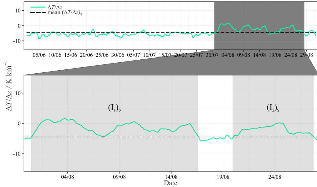
Figure 13: 24-h running mean of the pseudo-vertical temperature gradient in summer; two ‘persistent temperature inversion’ events ( I_1 s and I_2 s) detected by the TGM are shown in the shaded section and enlarged in the breakout panel beneath; see text in section 5.2.3.2 for details.
