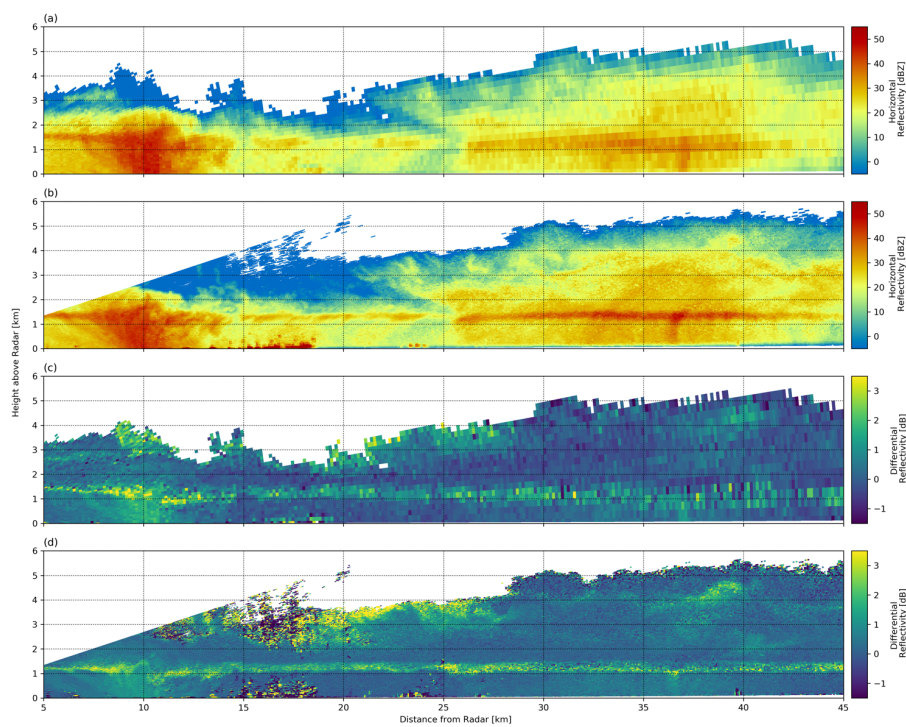
86 Figure 8. Coincident RHIs of Z_H (a and b) and Z_{DR} (c and d) from the NXPoI (a and c) and CAMRa (b and d) on 12 January 2017 87 at 13:36 UTC.
