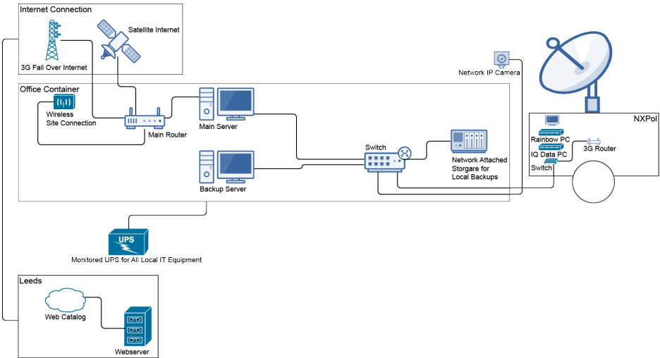
10 Figure 4. Schematic of the IT infrastructure used by the NXPol when on deployment.
