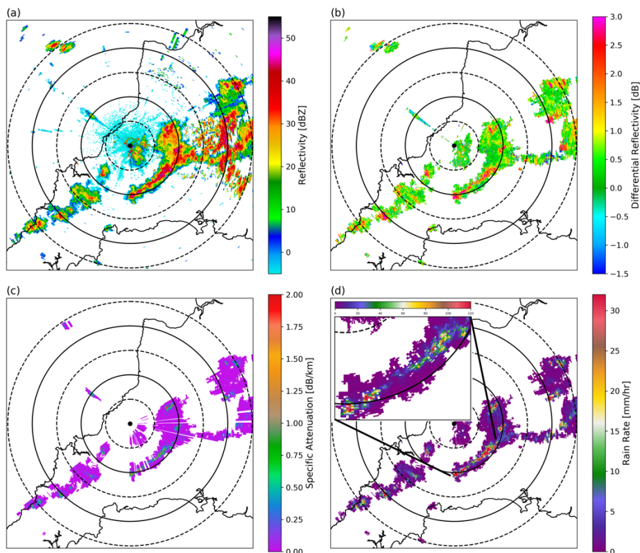
Figure 5. Example of observations made by NXPOL (located at the centre black dot) at 0.5^\circ elevation on 3 August 2013 at 1332 UTC showing: a) calibrated but unfiltered and uncorrected horizontal reflectivity (Shown as to display the importance and impact of the data processing), b) calibrated, filtered and corrected differential reflectivity, c) specific horizontal attenuation ( A_H ) and d) rainfall rates derived using the Marshall-Palmer relation ( R(Z)=aZ^b , with a=200 and b=1.6 ). The sub-panel in d) shows an expanded section of the line of intense rainfall ( >120\text{mm/hr} in some pixels; please note the expanded colorbar to the top of the sub-panel) to the southeast of the radar. Range rings are drawn every 10km.
