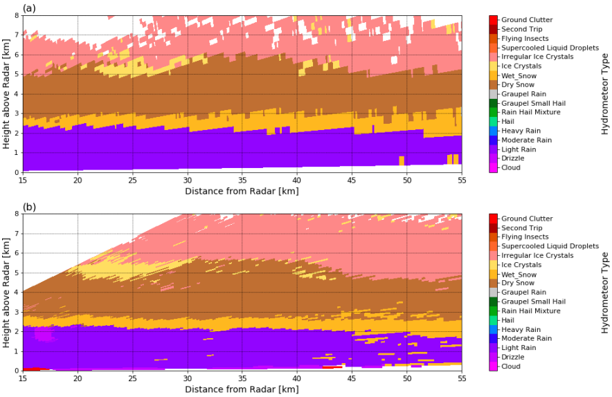
90 Figure 9. Coincident RHIs from the NXPoI (a) and CAMRa (b) on 17 May 2017 at 12:24 UTC with the HCA applied to both.
