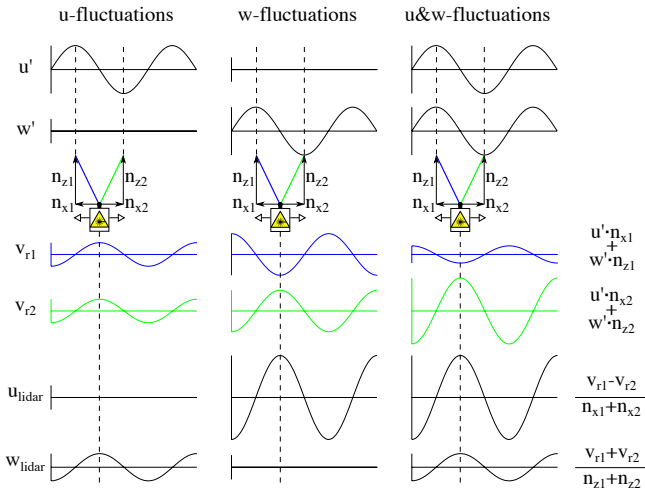
Figure 2. Visualization of cross-contamination caused by longitudinal spacing of measurement points 1 and 2. The wavelength of u' and w' equals twice the separation distance of the lidar (indicated by box with yellow symbol). The resulting measurement values of the u -component are contaminated by fluctuations in w -direction and vice versa.
