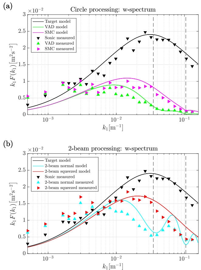
Figure 7. Modelled (solid lines) and measured (triangle markers) w -spectra from data processing where (a) all radial measurements are used and (b) only two beams are used. Colors correspond to processing method. The grey vertical dashed lines represent the first and second resonance wave number.
