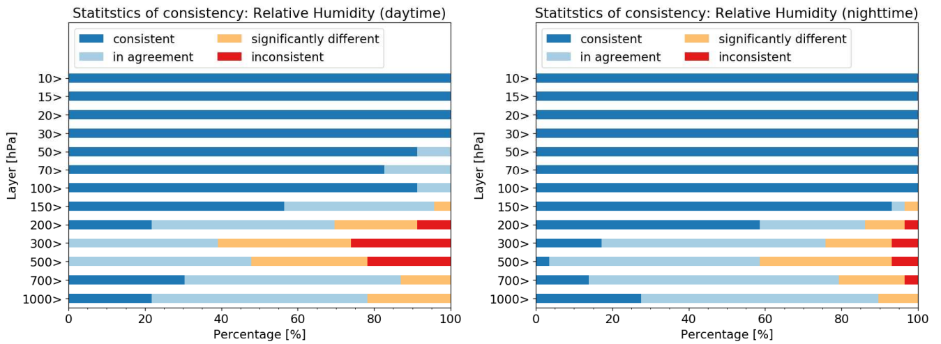
Figure 267: As per Fig. 24, but for RH. RH results for the stratosphere are not discussed here because measurement values for the stratosphere are considered to exceed the limit for reliable measurement.
