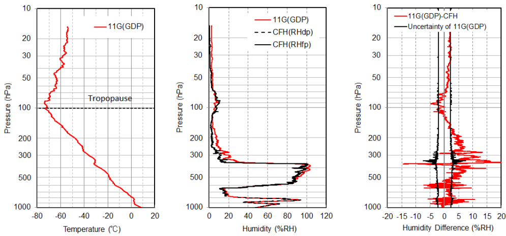
Figure 278: Profiles of temperature and RH/RH difference from an RS-11G and CFH comparison flight launched at 14:50 (LST) on 10 November, 2016. The panel on the left shows temperature data from RS-11G GDP. The middle panel shows the RH of RS-11G GDP (red), converted RH from CFH dewpoint temperature (black dashed line) below the height of the forced freezing point (Vömel et al., 2007), and converted RH from CFH frost point temperature (black thick line) above the height of the forced freezing point. The panel on the right shows RS-11G GDP minus CFH humidity difference (red) and the overall uncertainty of RS-11G GDP (black).
