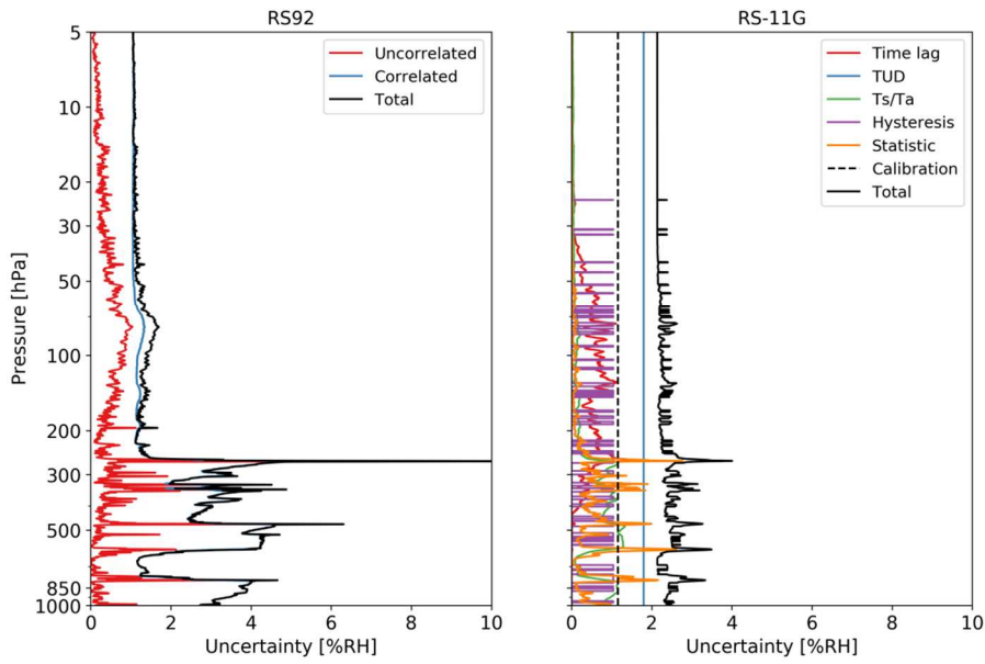
Figure 256: As per Fig. 23, but for RH
