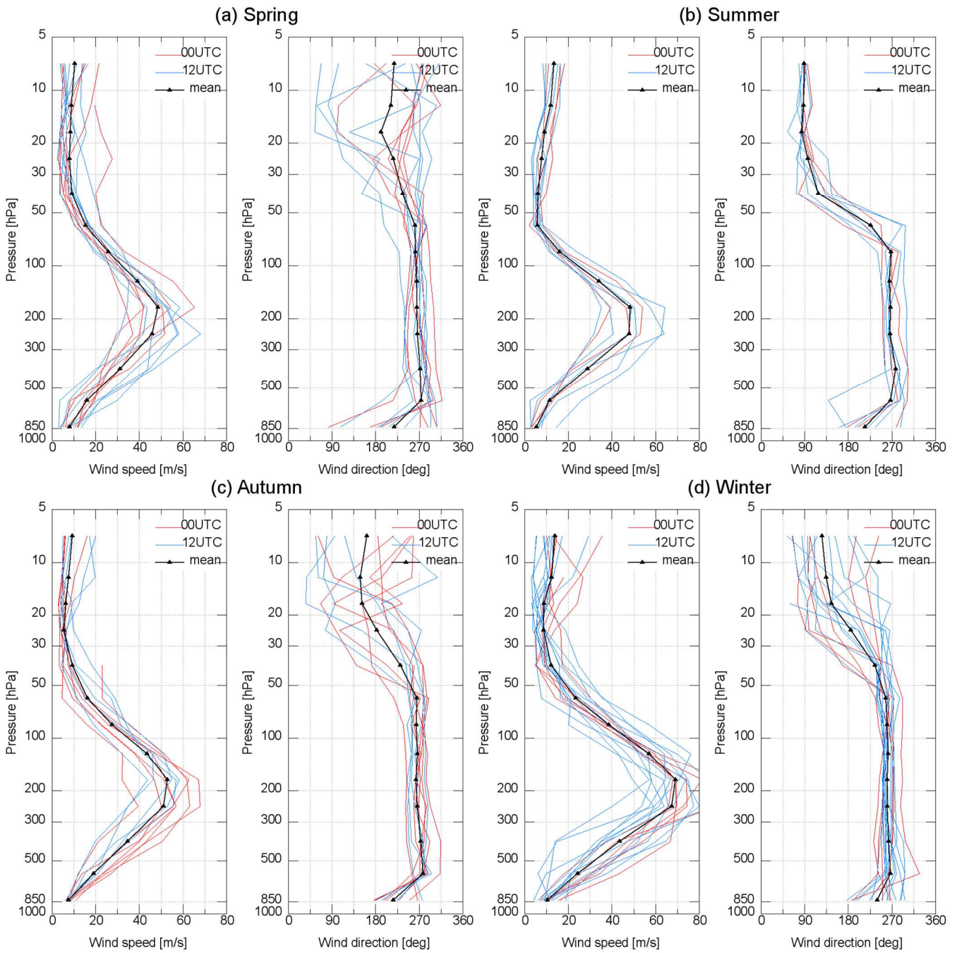
Figure 16: Seasonal profiles for wind speed and direction (As former Fig. 9), but for wind speed and direction
