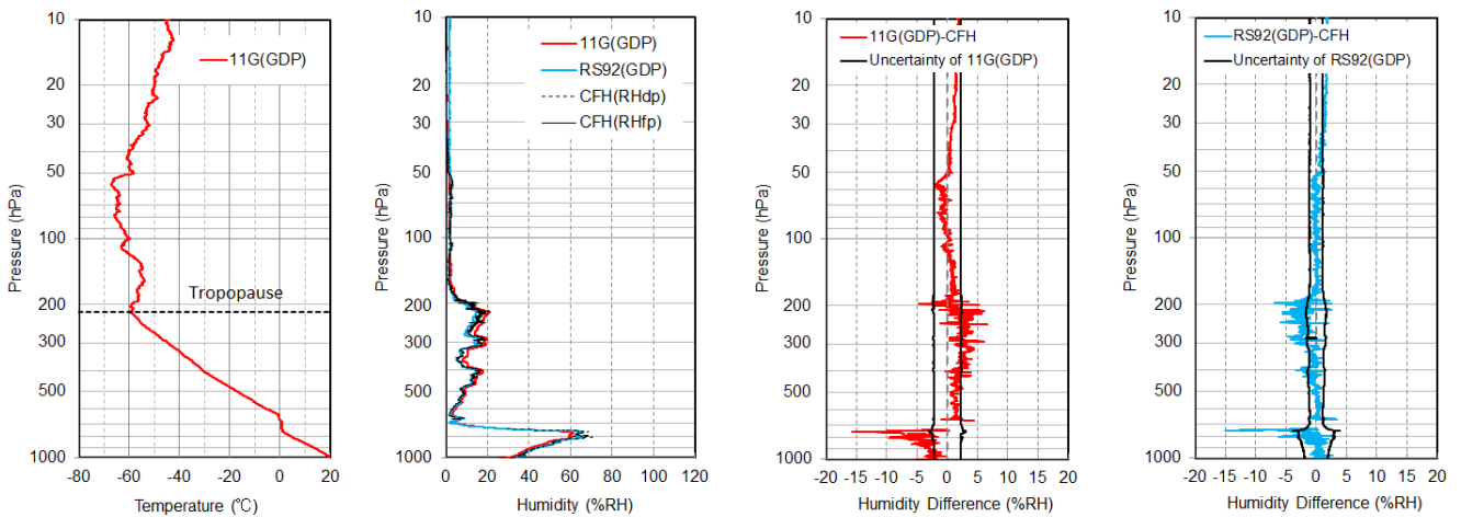
Figure 289: Profiles of temperature and RH/RH difference from an RS-11G, RS92, and CFH comparison flight launched at 14:50 (LST) on 20 April, 2018. The panel on the left shows temperature data from RS-11G GDP and the RH of RS-11G GDP (red), RS92 (light blue), converted RH from CFH dewpoint temperature (dashed black line) below the height of the forced freezing point, and converted RH from CFH frost point temperature (thick black line) above the height of the forced freezing point. The panel on the right shows RH differences for RS-11G GDP (red) and RS92 GDP (light blue) from CFH, and the overall uncertainties of RS-11G GDP and RS92 GDP (black).
