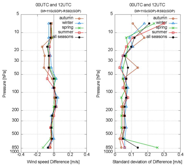
Figure 17: Profiles of differences and standard deviation, as for Fig. 10, but for wind speed for all soundings (00 and 12 UTC combined). As per Fig. 10, but for wind speed for all soundings (00 and 12 UTC combined)
