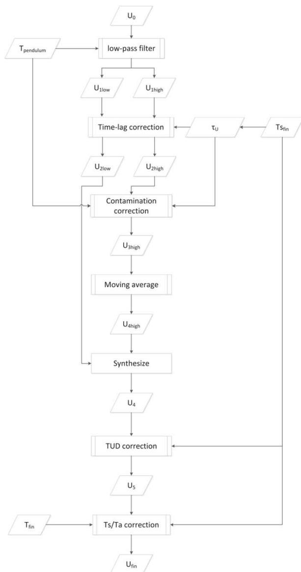
Figure 2: GRUAN data processing flow for RS-11G RH measurement (Kizu et al., 2018). U_0 is the uncorrected RH, T_{\text{pendulum}} is the period of pendulum motion, U_{1\text{low}} and U_{1\text{high}} are low- and high-frequency components of U_0 , \tau_U is the sensor response time, T_{S_{\text{fin}}} is the corrected RH sensor temperature, T_{\text{fin}} is the corrected final temperature, and U_{\text{fin}} is the corrected final RH value.
