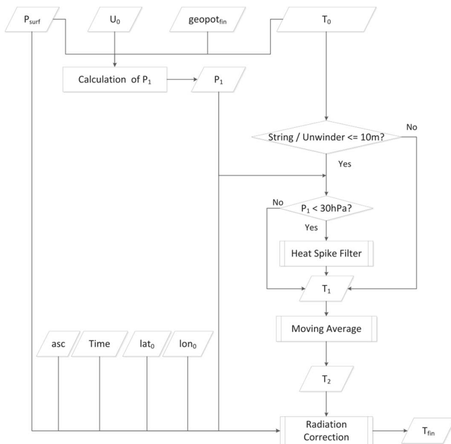
Figure 1: GRUAN data processing flow for RS-11G temperature measurement (excerpt from Kizu et al., 2018). T_0 and U_0 represent uncorrected temperature and RH, respectively, P_{surf} is surface pressure, lat_0 and lon_0 are the initial data set of GPS latitude and longitude, respectively, geopot_{fin} is the final geopotential height as derived from GPS altitude and latitude, asc is the ascent rate, and T_{fin} is the corrected final temperature value.
