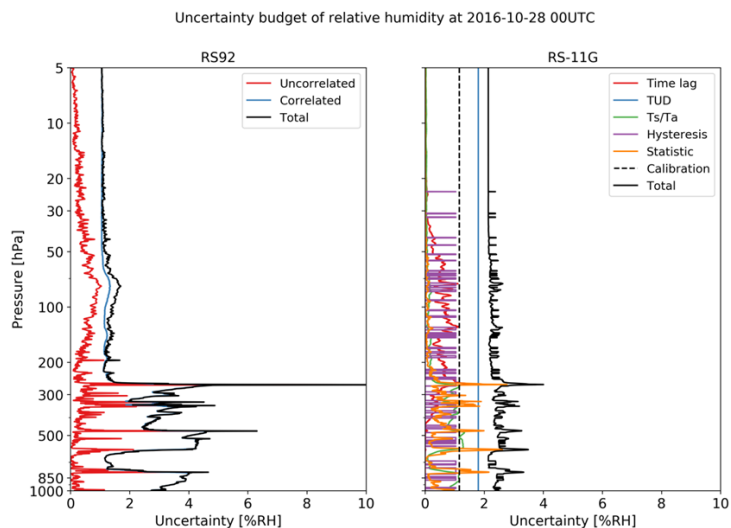
Figure 23: As per Fig. 21, but for RH
