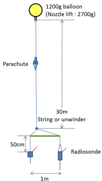
Figure 5: Flight configuration
