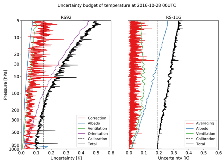
Figure 21: Uncertainty budget for temperature measurements at 00 UTC (daytime) on 28th October, 2016, for RS92 GDP (left) and RS-11G GDP (right)
