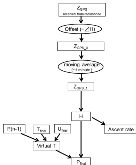
Figure 3: GRUAN data processing flow for RS-11G geopotential height and pressure measurement (Kizu et al., 2018). Z_{GPS} is the GPS geometric altitude, \Delta H is the offset between balloon release altitude and GPS geometric altitude upon balloon release, H is the geopotential height, T_{final} and U_{final} are the corrected final temperature and RH, respectively, and P_{final} is the corrected final pressure.
