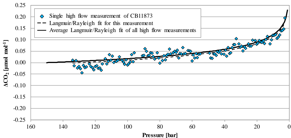
Figure 8: The blue diamonds represent the \text{CO}_2 mole fraction measurement of the high flow experiment done on 5.4.2017 with CB11873 vertically positioned as a function of pressure, note the inverse pressure scale. The black dashed line is a fit following the combined Langmuir adsorption/desorption and Rayleigh distillation model, the black solid line represents the average of the combined Langmuir and Rayleigh fit using all high flow experiments with vertically positioned cylinders. In order to plot all data in one plot, the corresponding (X_{\text{CO}_2, \text{ini}} - X_{\text{CO}_2, \text{ad}}) was subtracted from the measurements and the fits.
