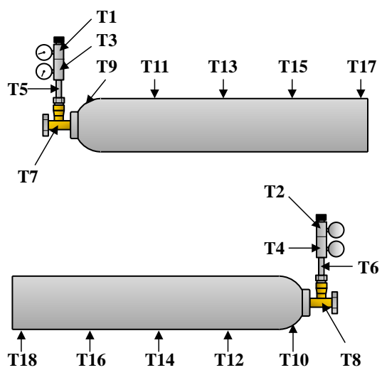
Figure 5: Schematic of the locations of the thermistors on the cylinder in vertical (a) and horizontal position (b) as well as the heating bands if used. Thermistors 19 to 25 were bundled and used to measure the background temperature of the laboratory.
