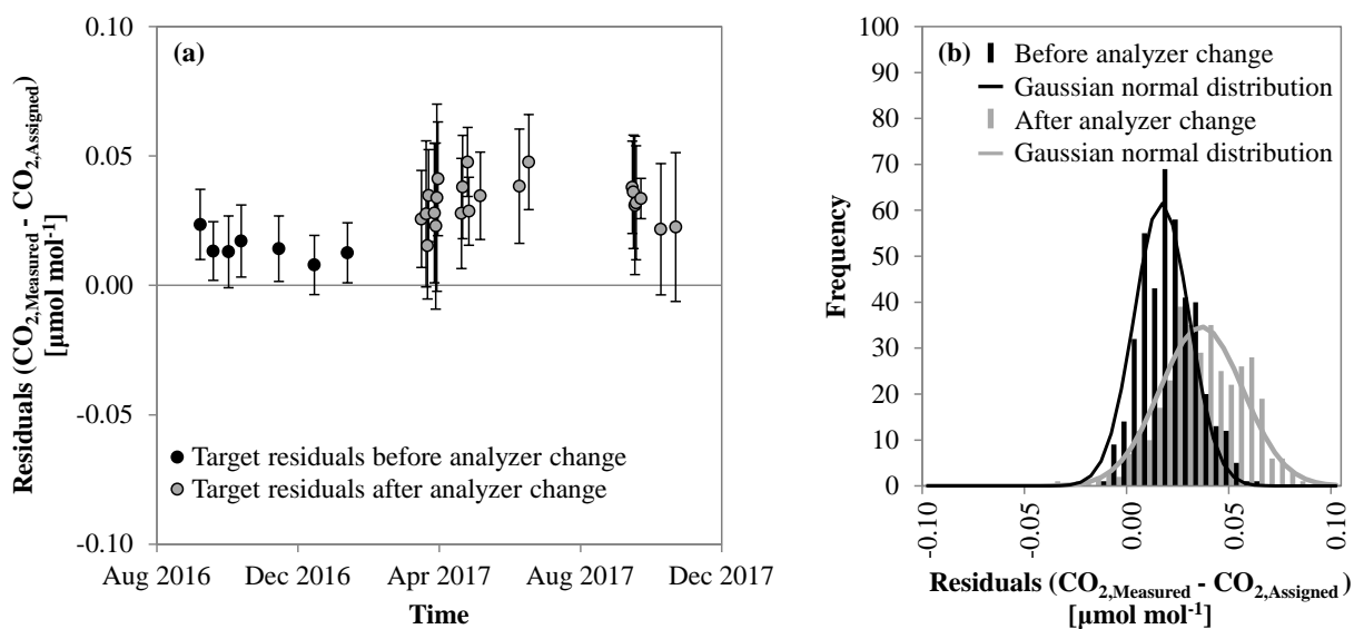
Figure 4: Panel (a): Average of the difference of the target gas measurement minus the assigned CO 2 mole fraction for each run against time, black indicates the measurements before the analyzer change, grey after the analyzer change in March 2017. The error bars correspond to the standard deviation of the individual target gas measurements within each run. Panel (b): Histogram of the residuals of the target gas measurements, again, black stands for the measurements before, grey after the analyzer change.
