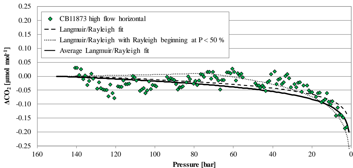
Figure 12: The green diamonds represent the \text{CO}_2 mole fraction measurement of the high flow experiment done on 4.5.2017 with CB11873 horizontally positioned as a function of pressure, note the inverse pressure scale. The black dashed line is a fit following the combined Langmuir adsorption/desorption and Rayleigh distillation model, the black dotted line is a fit following the combined Langmuir adsorption/desorption and Rayleigh distillation model with the Rayleigh distillation starting when the cylinder is half empty, the black solid line represents the average of the combined Langmuir and Rayleigh fit using all high flow experiments with horizontally positioned cylinders. In order to plot all data in one plot, the corresponding (X_{\text{CO}_2, \text{ini}} - X_{\text{CO}_2, \text{ad}}) was subtracted from the measurements and the fits.
