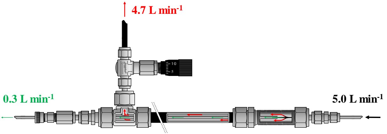
Figure 2: Flow schematic of the high flow inlet system. The sample gas enters on the right side at 5.0 \text{ L min}^{-1} . A small aliquot of 0.3 \text{ L min}^{-1} goes to the analyzer, the remainder of 4.7 \text{ L min}^{-1} goes to the exhaust. The ratio between the gas going to the analyzer and the exhaust, respectively, is set by the dimensions of the inner and outer tube and can be adjusted by the needle valve on the exhaust side.
