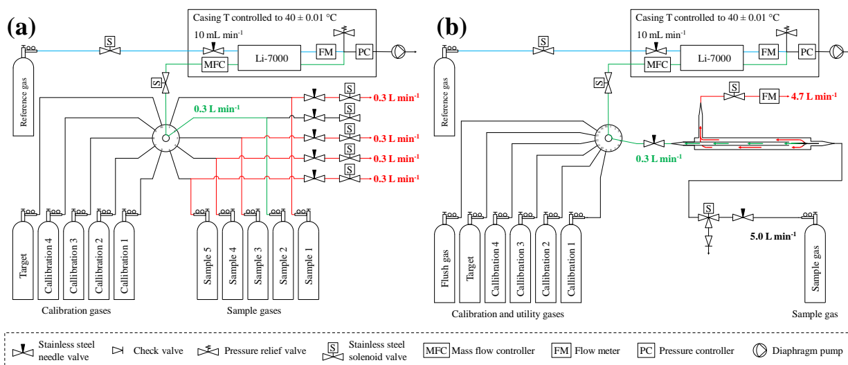
Figure 1: Schematic of the low flow measurements system setup, here with the 10-port vici valve (a) and the high flow measurement system setup with the 16-port VICI valve (b). The red lines and numbers indicate the gas that is drained to the room to maintain a steady flow out of the cylinder, the green lines and numbers are what goes into the analyzer, the blue lines are the reference gas flow.
