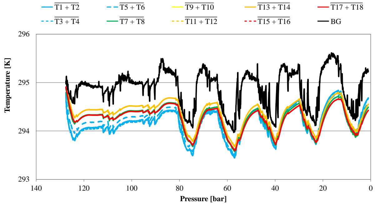
5 Figure 7: Temperature development of CB11795 during the low flow measurement with horizontally positioned cylinders as a function of pressure, note the inverse pressure scale. The lines represent averages of the following thermistors: Pressure regulator to stem: Solid blue: T1 and T2; dotted blue: T3 and T4; dashed blue: T5 and T6; Cylinder valve: green: T7 and T8; Cylinder body: yellow: T9 and T10; dashed orange: T11 and T12; solid orange: T13 and T14; dashed red: T15 and T16; solid red: T17 and T18; laboratory background: black: T19 to T25.
