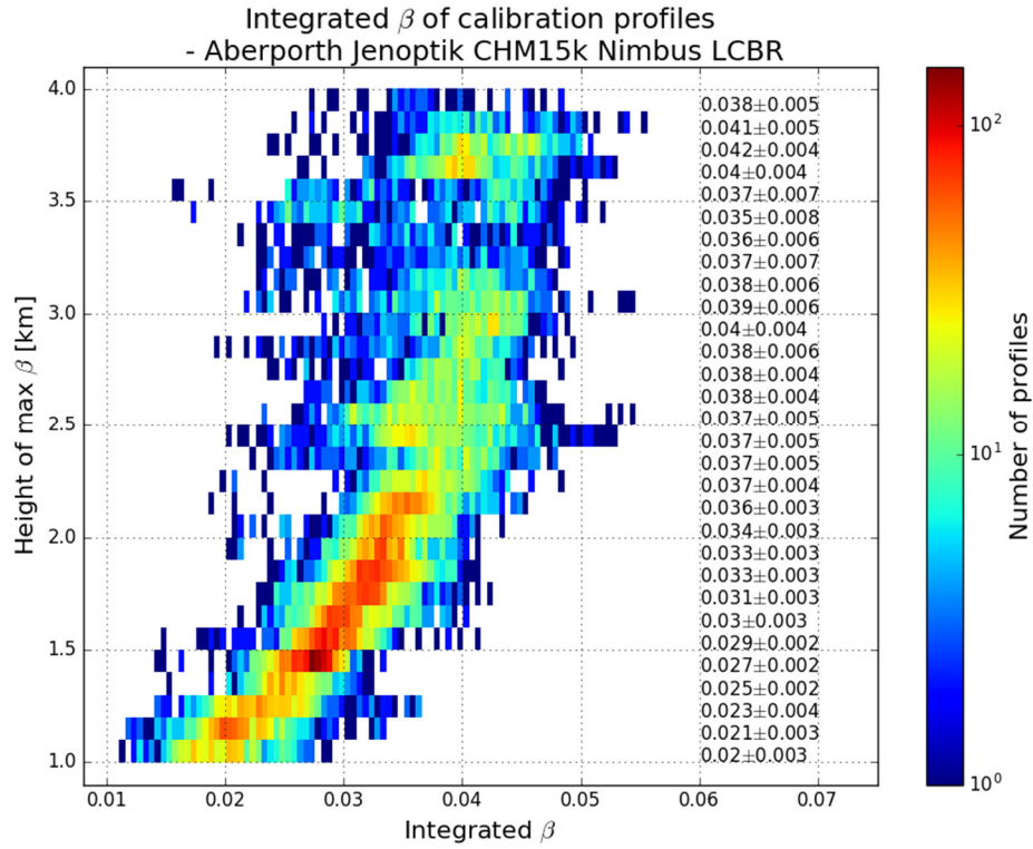
Figure 11: As for Figure 6, but illustrating the saturation of the CHM15k ceilometer for most clouds with bases below 2km. 2D histogram of the value of the integrated attenuated backscatter in profiles used for calibration with range. A height dependent multiple scattering correction has been applied. Darker colours (towards red) indicate a higher density of profiles. The values shown along the right-hand side give the mean \pm the standard deviation of the integrated attenuated backscatter (units \text{sr}^{-1} ) at 100m intervals.
