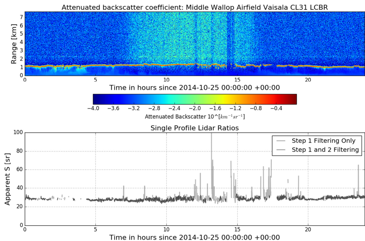
Figure 3: (a) Uncalibrated attenuated backscatter vertical profiles (colours shown on a log scale) for 25th October 2014 from a CL31 ceilometer at Middle Wallop airfield (51.1489 N, 1.5700 W) and (b) the apparent lidar ratio for the same day. In panel (b), the grey line shows the apparent S for profiles that pass the step 1 filtering of the calibration algorithm and the black line shows the profiles that pass the step 2 filtering and are used to calculate the calibration coefficient.
