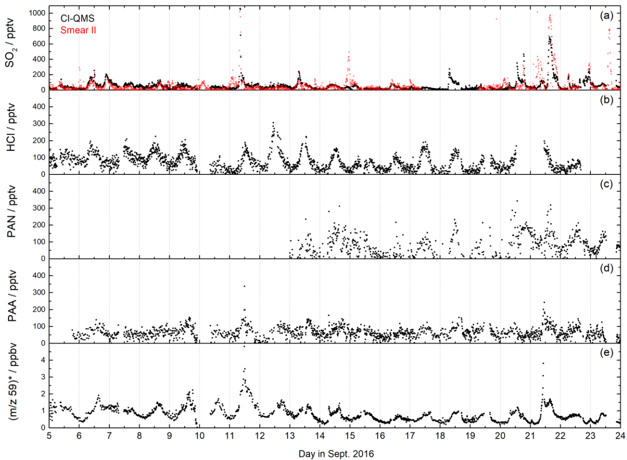
Figure 8: CI-QMS time series of \text{SO}_2 , HCl, PAN, PAA mixing ratios and m/z 59 during the IBAIRN campaign in the boreal forest. The red \text{SO}_2 trace was obtained using a TEI 43 CTL fluorescence analyser (Smear II). The signal at m/z 59 was converted to ppbv assuming that it consists only of acetic acid (no peracetic acid). The mixing ratios are therefore only an upper limit.
