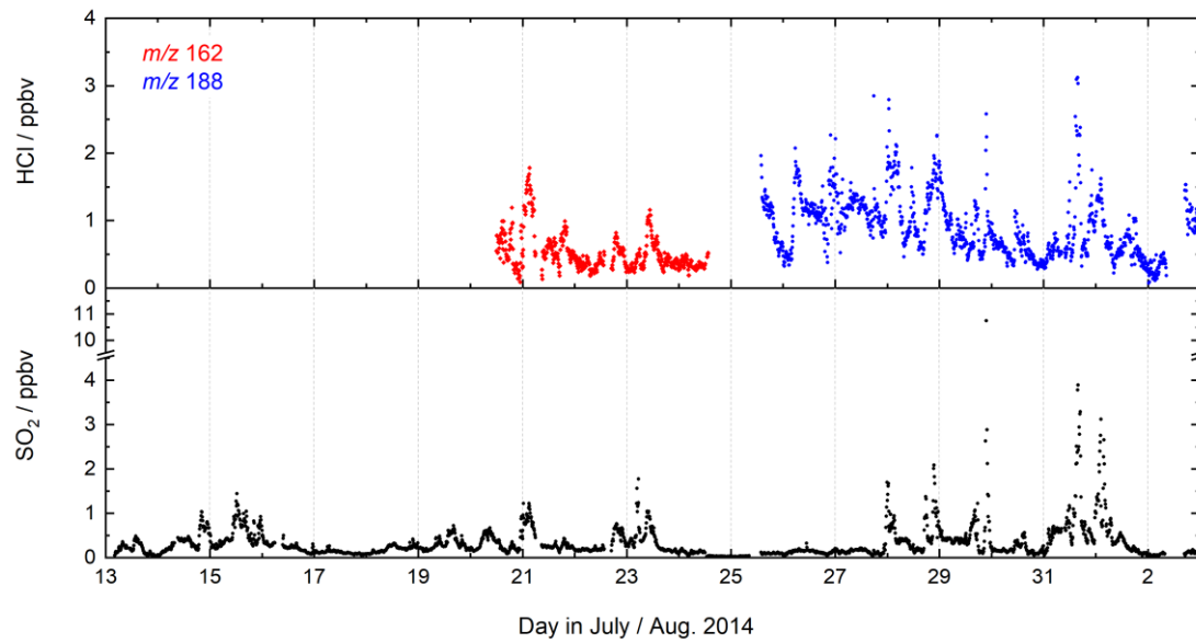
Figure 6: CI-QMS time series of SO_2 and HCl mixing ratios during the CYPHEX field campaign in Cyprus.
