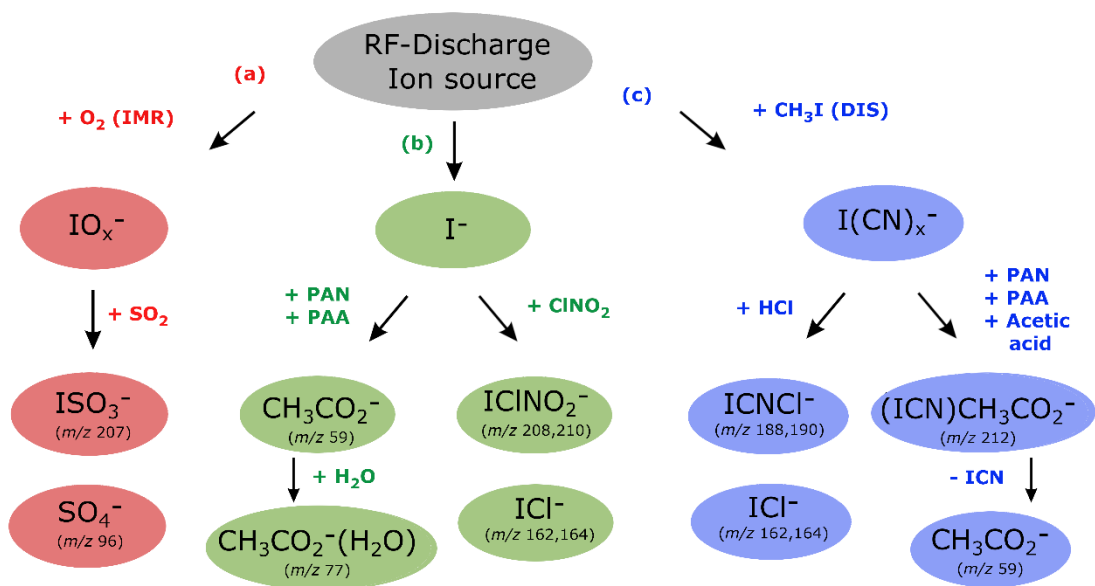
Figure 4: Ion detection schemes for SO 2 , PAN, PAA, acetic acid, ClNO 2 and HCl using the RF discharge ion source.
