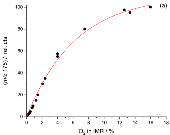
Figure S2. (a): Dependence of \text{IO}_3^- signal ( m/z 175) on the fractional pressure of \text{O}_2 in the IMR when adding 800 sccm \text{N}_2 / \text{CH}_3\text{I} through the RF discharge region. (b): Signal at m/z 207 ( \text{ISO}_3^- ) for a constant amount of \text{SO}_2 over the same range of \text{O}_2 partial pressures.
