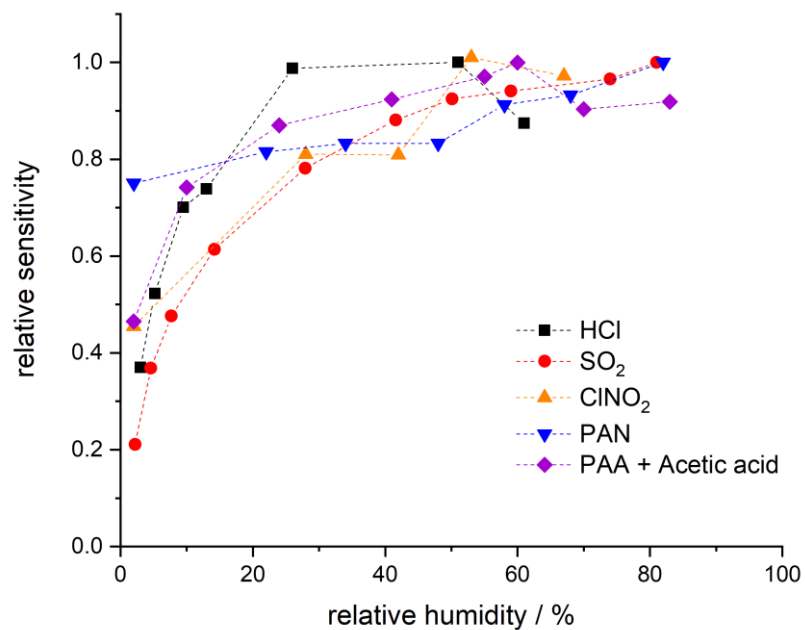
5 Figure 5: Dependence of ion signal on the relative humidity (at 25 °C and 1 bar) of the air sampled. For PAA + acetic acid on m/z 59 only a combined humidity dependence is given as their contributions to the signal could not reliably be quantified.
