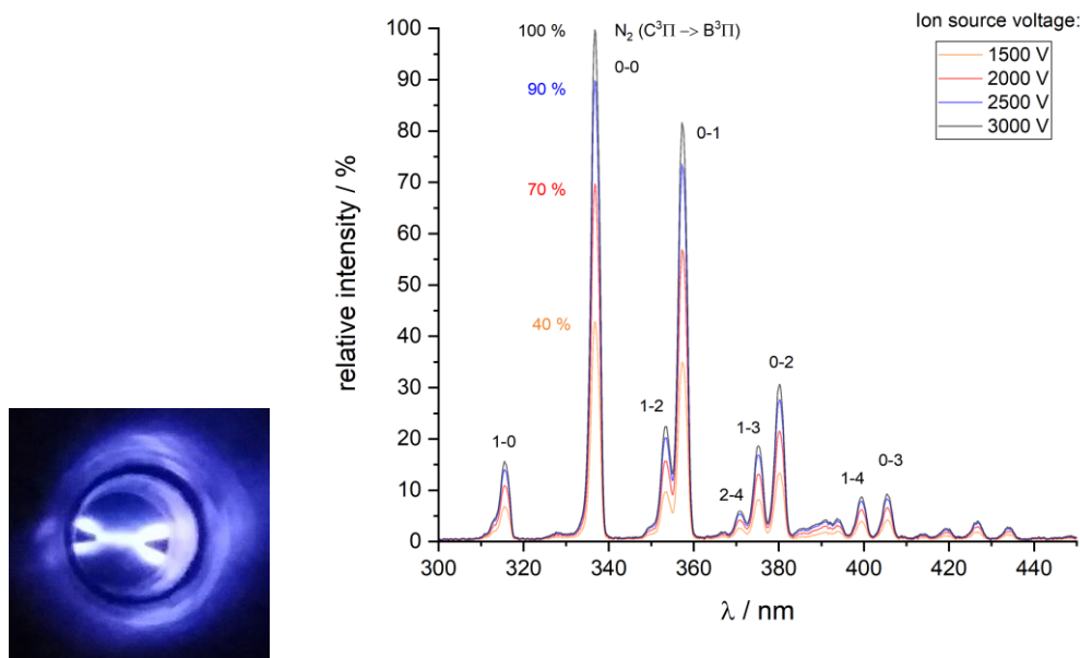
Figure S1. Photo: N 2 emission observed between and around the pointed tungsten tips of the electrodes of the RF discharge source. Right: The emission spectrum was recorded with an Ocean-Optics USB-4000 spectrometer with optical fibre at various high-voltages. The strongest features (not fully resolved using the low-resolution ( \Delta\lambda \approx 1.5 nm) spectrograph) can be assigned to transitions from the ground vibrational level of the electronically excited N 2 (C 3 Π u ) state to the B 3 Π g state.
