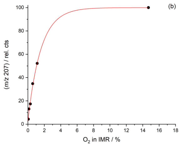
Figure S2. (a): Dependence of \text{IO}_3^- signal ( m/z 175) on the fractional pressure of \text{O}_2 in the IMR when adding 800 sccm \text{N}_2 / \text{CH}_3\text{I} through the RF discharge region. (b): Signal at m/z 207 ( \text{ISO}_3^- ) for a constant amount of \text{SO}_2 over the same range of \text{O}_2 partial pressures.
