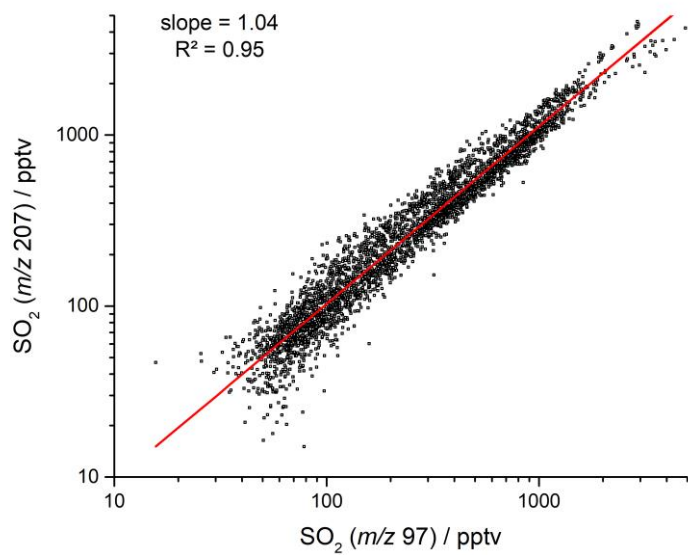
5 Figure S6: Correlation between the CI-QMS measurement of SO 2 at m/z 207 (ISO 3 - ) vs. m/z 97 (HSO 4 - ) during NOTOMO.
