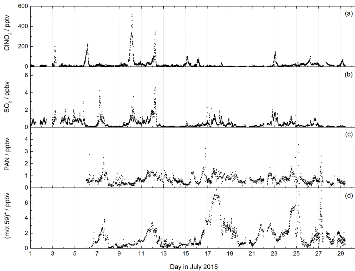
Figure 7: CI-QMS time series of CINO 2 , SO 2 , PAN mixing ratios and m/z 59 during the NOTOMO field campaign in Germany. The signal at m/z 59 was converted to ppbv assuming that it consists only of acetic acid (no peracetic acid). The mixing ratios are therefore only an upper limit. For comparison with PARADE campaign at the same location see Fig. S7 in the supplement.
