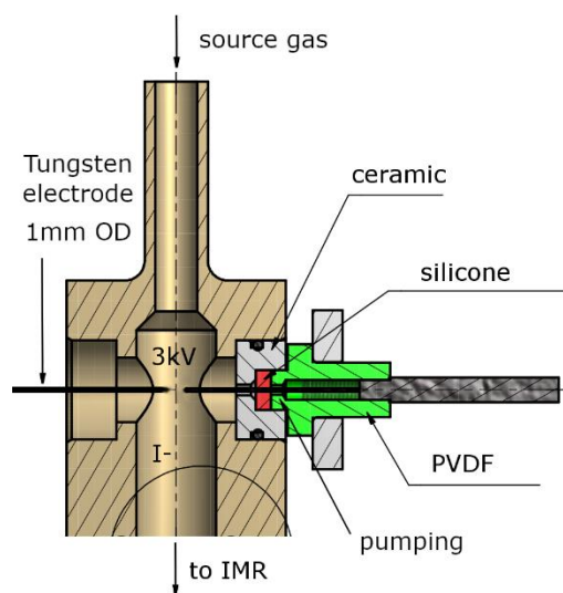
Figure 2: Schematic drawing of the RF-discharge ion source. The high voltage and the distance between the tips of the tungsten electrodes are variable, as described in the text. PVDF is polyvinylidene fluoride. The region around the electrodes can be optionally pumped as described in the text.
