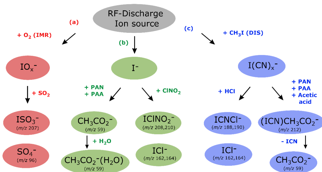
Figure 4: Ion detection schemes for SO 2 , PAN, PAA, acetic acid, ClNO 2 and HCl using the RF discharge ion source.
