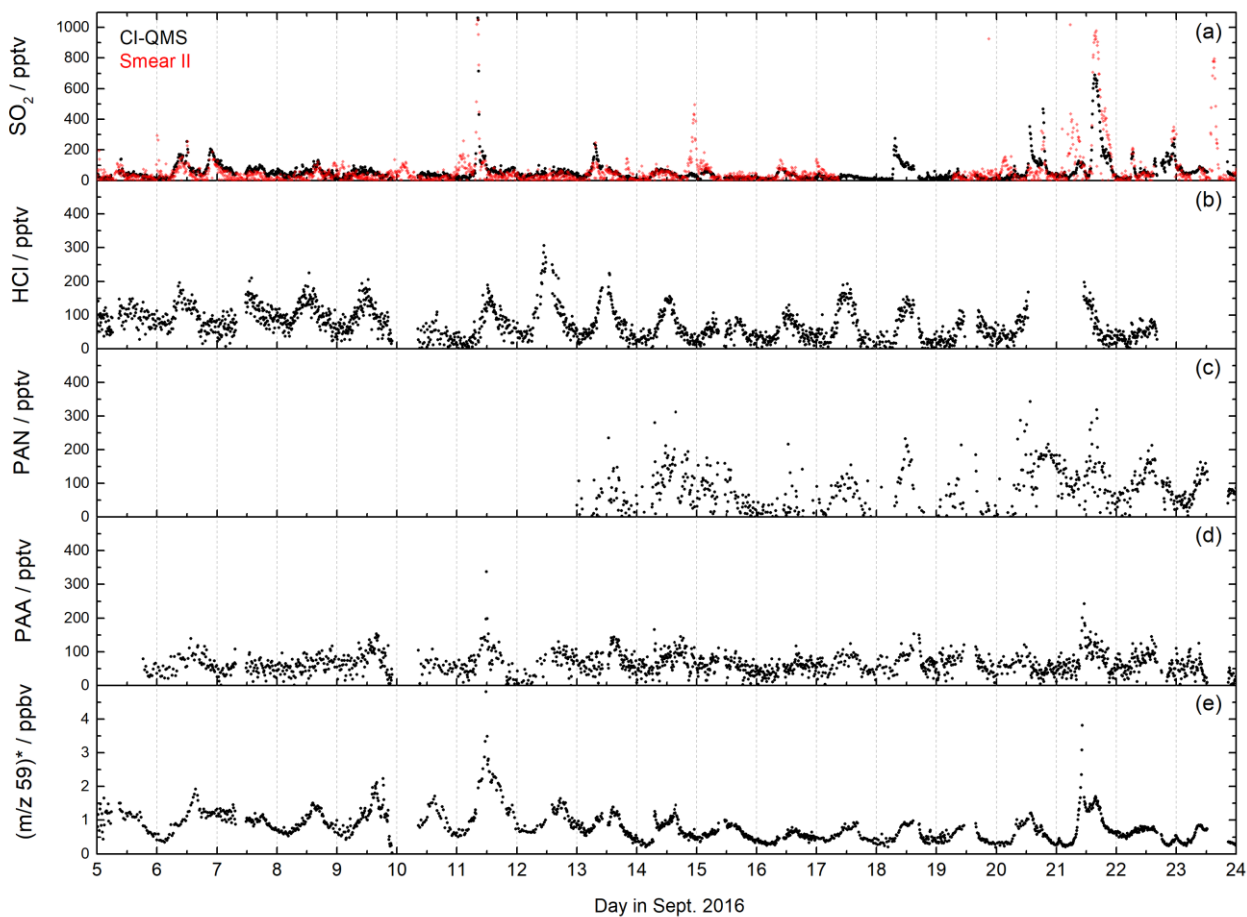
Figure 8: CI-QMS time series of SO 2 , HCl, PAN, PAA mixing ratios and m/z 59 during the IBairn campaign in the boreal forest. The red SO 2 trace was obtained using a TEI 43 CTL fluorescence analyser (Smear II). The signal at m/z 59 was converted to ppbv assuming that it consists only of acetic acid (no peracetic acid). The mixing ratios are therefore only an upper limit.
