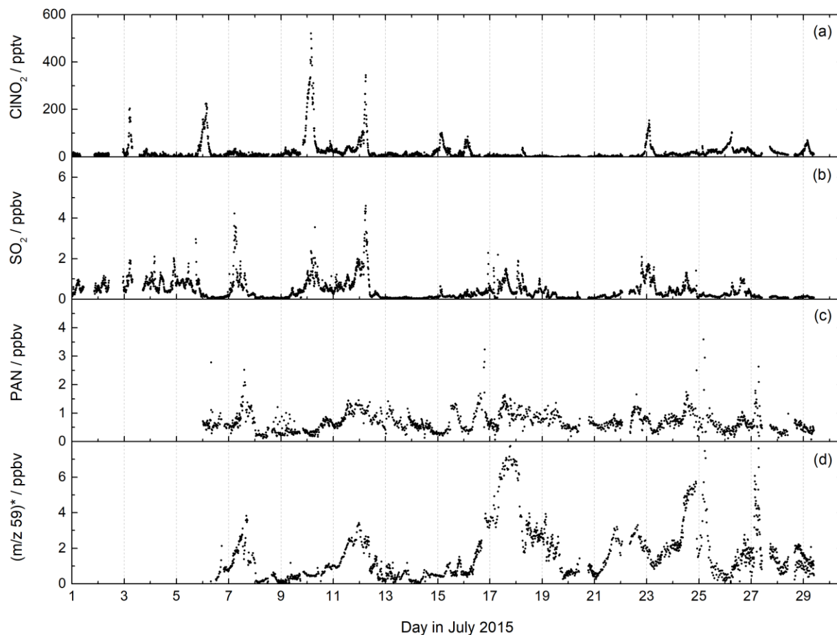
Figure 7: CI-QMS time series of ClNO 2 , SO 2 , PAN mixing ratios and m/z 59 during the NOTOMO field campaign in Germany. The signal at m/z 59 was converted to ppbv assuming that it consists only of acetic acid (no peracetic acid). The mixing ratios are therefore only an upper limit. For comparison with PARADE campaign at the same location see Fig. S6 in the supplement.
