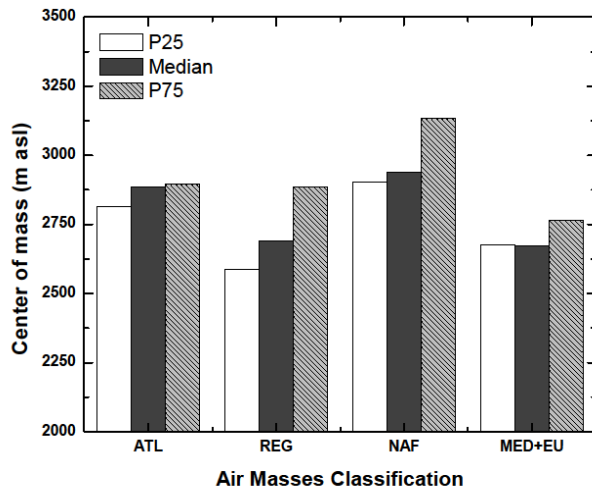
10 Figure 7: Bar-plot of the center of mass in (m a.s.l. ( note that MSA observatory is at 1570 m a.s.l. )) of the 25 th percentile (P25), median and 75 th percentile (P75) profiles, separated as a function of air mass (ATL = Atlantic, REG = Regional, MED+EU = Mediterranean and European, NAF = North African).
