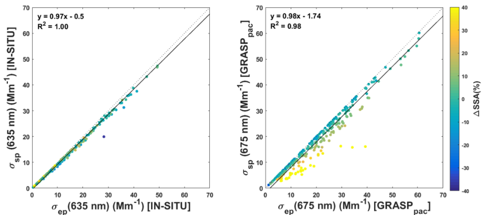
10 Figure 3: Scatter plots of the hourly averaged aerosol light scattering and extinction coefficients measured in-situ (left panel) and retrieved with GRASP pac algorithm (right panel). The color scale represents the relative difference in the single scattering albedo, SSA, between in-situ and GRASP pac data.
