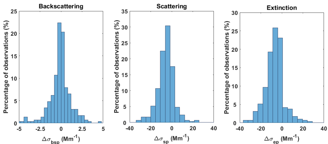
Figure 2: Histograms of the relative-absolute difference between in-situ measured and retrieved with GRASP pac optical parameters (aerosol light -backscattering, scattering and extinction coefficients) at low ambient RH ( \text{RH}_{\text{ambient}} < 50\% ).
