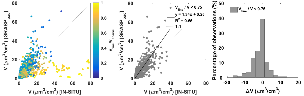
10 Figure 4: (a) Scatter plot of the hourly averaged aerosol volume concentration determined with GRASP pac from the ceilometer and photometer data at MSA height versus the in-situ concentrations at low ambient RH ( \text{RH}_{\text{ambient}} < 50\% ), with the color scale representing the contribution of fine particles to the total volume concentration. (b) Same than (a) but restricted to situations with contribution of fine particles to the total aerosol volume concentration < 75% ( V_{\text{fine}} / V < 0.75 ). (c) Frequency of occurrence of the relative absolute difference between the volume concentrations measured in-situ and determined with GRASP pac for situations with 15 V_{\text{fine}} / V < 0.75 .
